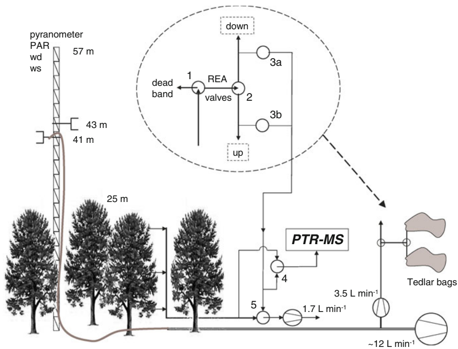
Fig. 1 Experimental setup at the Soroee field site (not to scale). Inset magnifies REA setup for the bag sampling. Circles with numbers mark the high speed PTFE valves. Valves 1 and 2 decided between sampling or not, and into which bag, respectively. Valves 3a and 3b are used to access the bag samples consecutively, and Valve 4 allowed the PTR-MS to switch between the bag samples and the gradient
