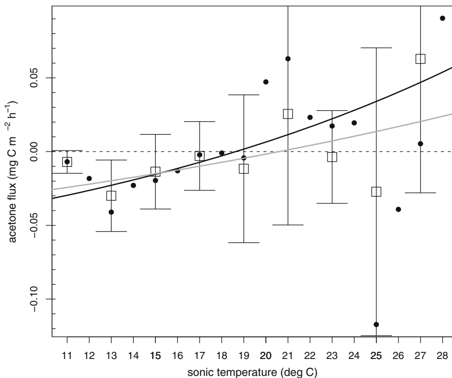
Fig. 5 Acetone flux as a function of sonic virtual temperature. Closed circles show 1-degree, open squares 2-degree binned average fluxes, error bars show \pm 1 standard deviation ( N = 6-31 ). The solid black and grey lines are weighted log-linear regressions to the circles and squares , respectively
