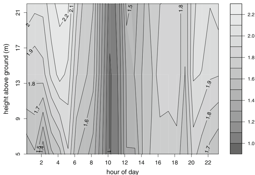
Fig. 7 Interpolated mean methanol mixing ratios as a function of time of day and height above ground inside the beech forest. Only measurements after DOY 164 are shown to avoid averaging skewed distributions
