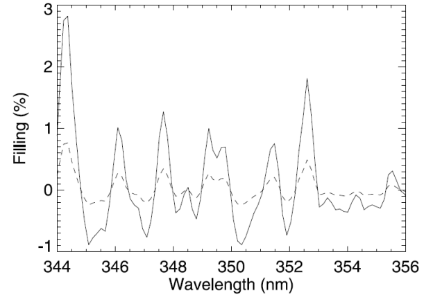
Figure 3.4: A nadir observation of RRS filling-in at 700 hPa (solid line) and at 200 hPa (dashed line) with albedo of 0.6 for a Lambertian surface (Vasilkov et al., 2008).
