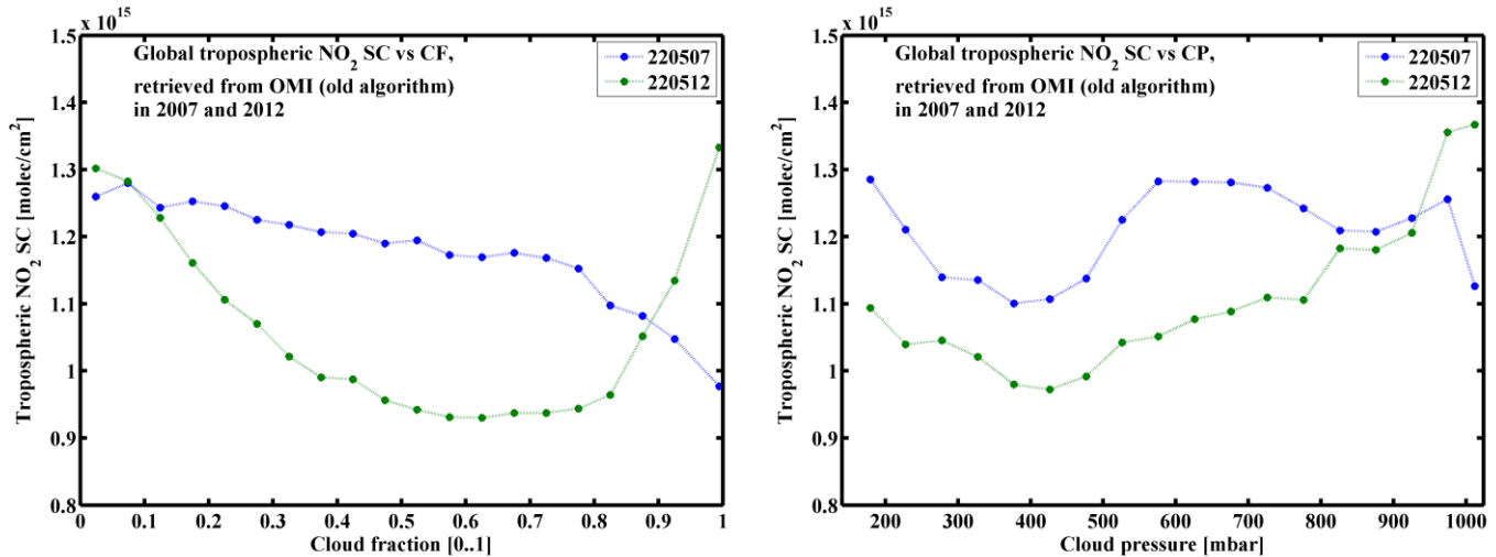
Figure 7.3: Global cloud impacts on tropospheric NO 2 SC retrieved from OMI old algorithm on one day of 2007 and 2012, with CF (left) and CP (right).
