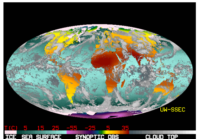
Figure 2.1: Cloud appearance viewed from space. Combined from GMS, GOES-8 and Meteosat imagery on October 15, 2015. http://www.ssec.wisc.edu/data/comp/latest_cmoll.gif
