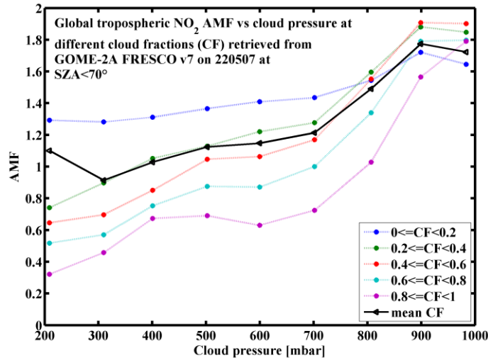
Figure 5.2: The difference of NO 2 AMF with respect to cloud pressure using GOME-2A FRESCO7 algorithm on May 22, 2007 averaged over global dataset.
