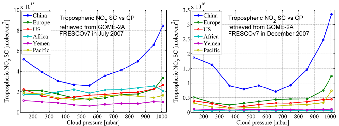
Figure 4.7: Cloud pressure impacts on tropospheric NO 2 SC from GOME-2A FRESCOv7 in July (left) and December (right) 2007 over 6 different regions
