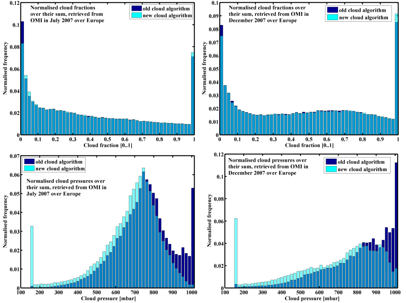
Figure 6.2: The OMI cloud distribution over Central Western Europe in July (left column) and in December (right column) 2007, CFs (upper row) and CPs (lower row).
