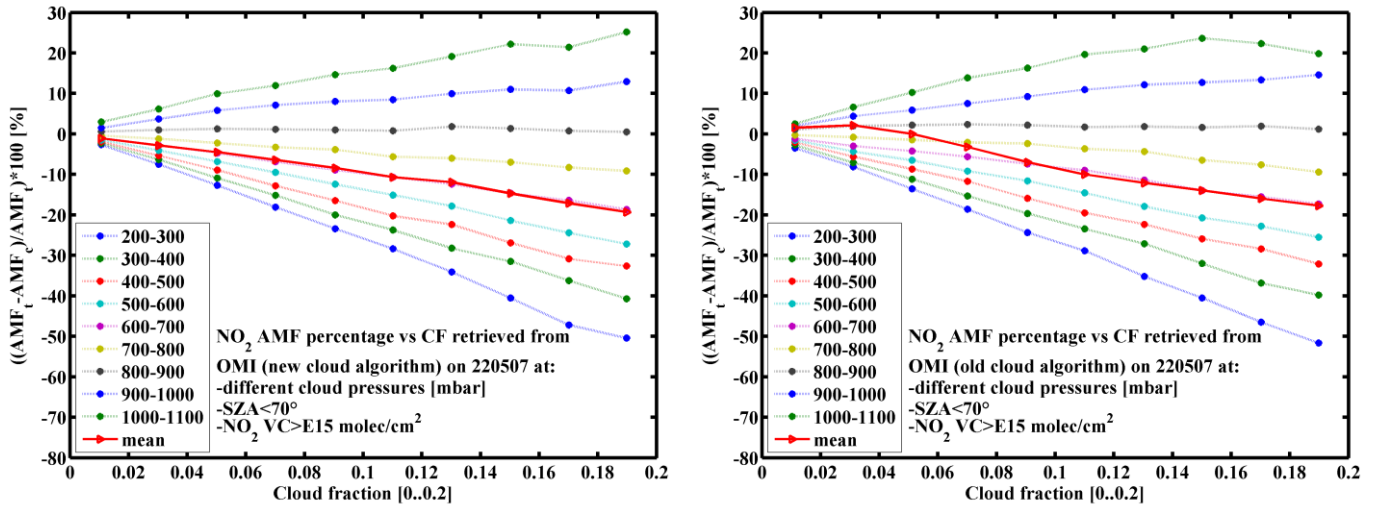
Figure 5.3: The effect of cloud correction on the tropospheric NO 2 AMF for cloud fraction <0.2 at different cloud pressures from OMI using new cloud algorithm (left) and old cloud algorithm (right) for a global retrieval on May 22, 2007.
