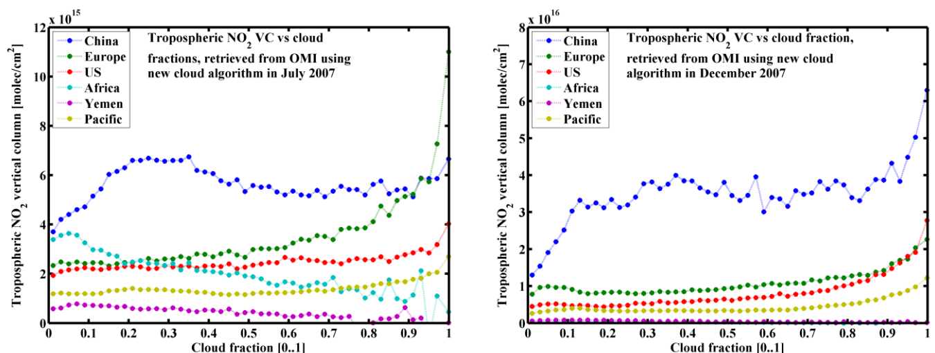
Figure 6.9: Cloud impacts on tropospheric NO 2 VC from OMI new cloud algorithm in July (left) and December 2007 (right) over 6 regions
