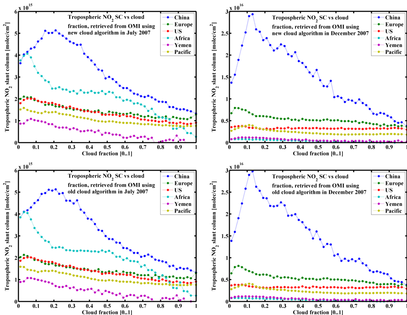
Figure 6.7: Cloud impacts on tropospheric \text{NO}_2 SC in July (left column) and December (right column) 2007 over 6 regions, from OMI using new algorithm (upper row) and old algorithm (lower row).
