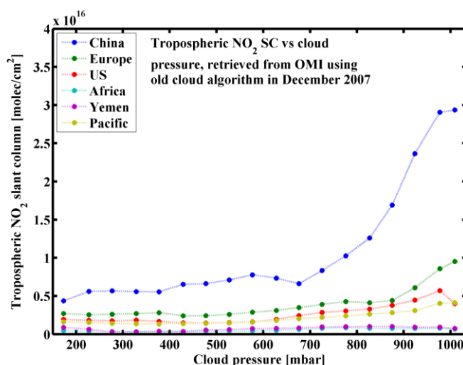
Figure 6.8: Cloud pressure impacts on tropospheric NO 2 SC retrieved from OMI old algorithm in December 2007 over 6 regions
