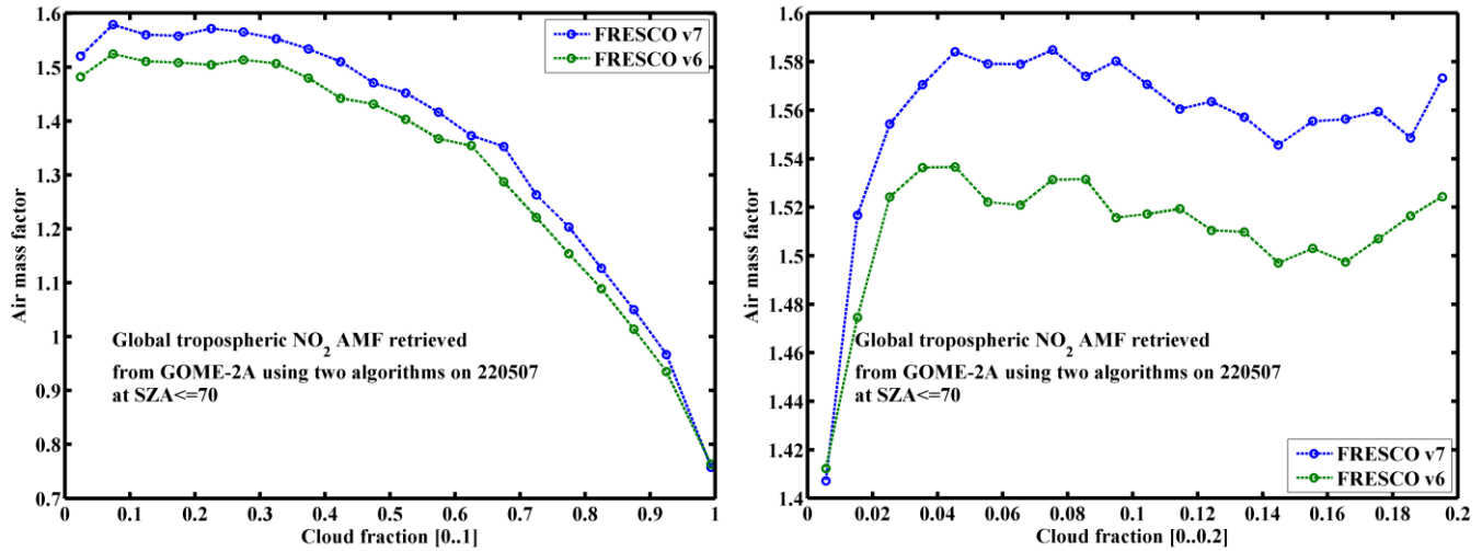
Figure 5.1: The difference of NO 2 AMFs with respect to cloud fraction using GOME-2A FRESCO7 and FRESCO6 algorithms on May 22, 2007 averaged over the global dataset.
