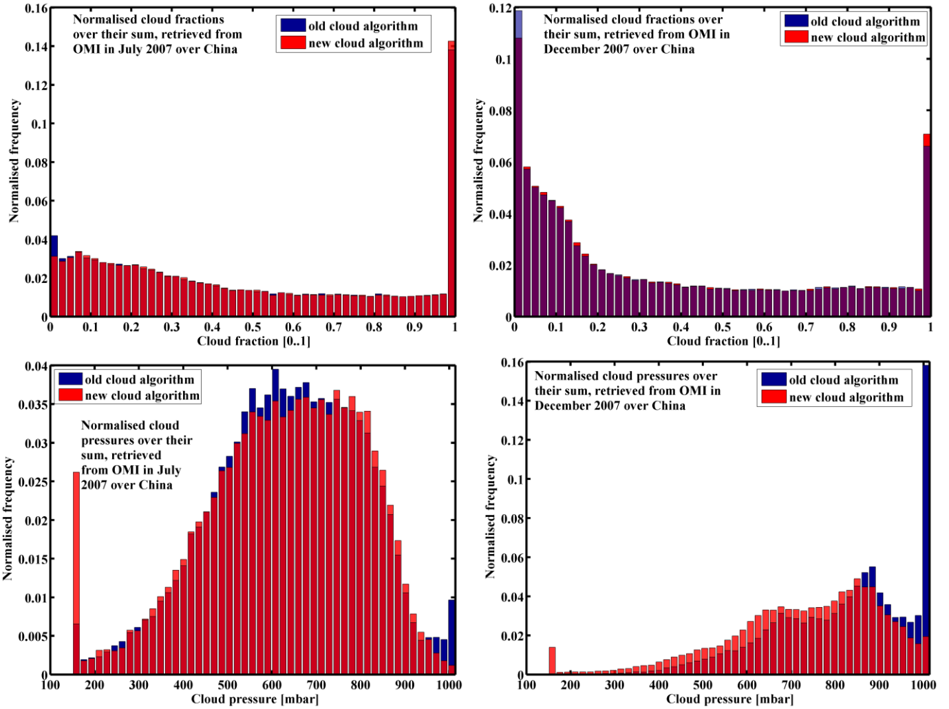
Figure 6.1: OMI cloud property frequency distributions over Central Eastern China in July (left column) and in December (right column) 2007, CFs (upper row) and CPs (lower row).
