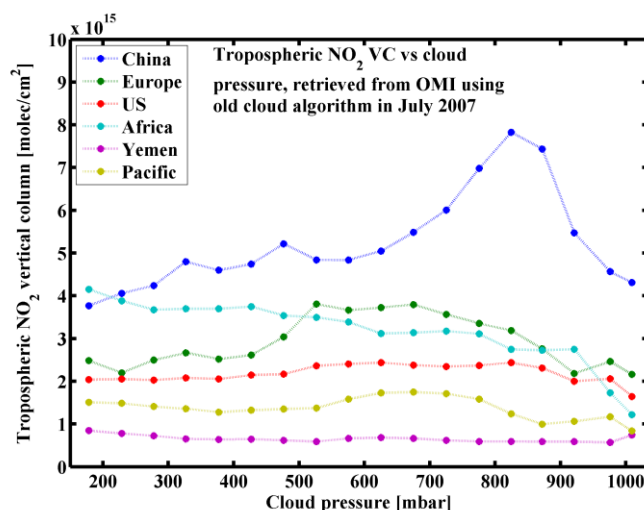
Figure 6.10: Cloud pressure effect on tropospheric NO 2 VC from OMI old cloud algorithm in July 2007 over 6 regions
