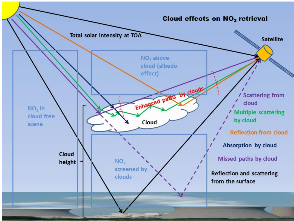
Figure 3.1: Scheme of the relevant effects of cloud on \text{NO}_2 column retrievals
