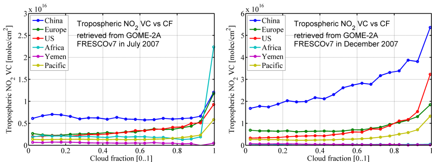
Figure 4.8: The tropospheric NO 2 VC from GOME-2A FRESCOv7 in July (left) and in December (right) 2007 over the mentioned regions
