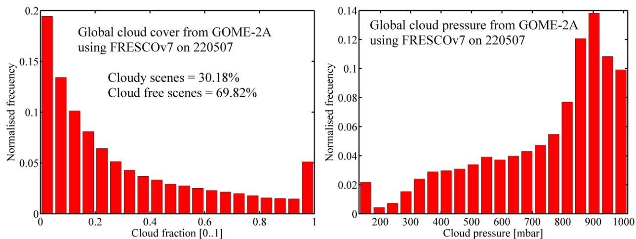
Figure 11.8: Global cloud statistics from GOME-2A on 220507, cloud fraction (left) and cloud pressure (right).
