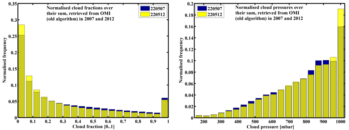
Figure 7.1: OMI global cloud statistics for May 22 in 2007 and 2012, cloud fraction (left) and cloud pressure (right).
