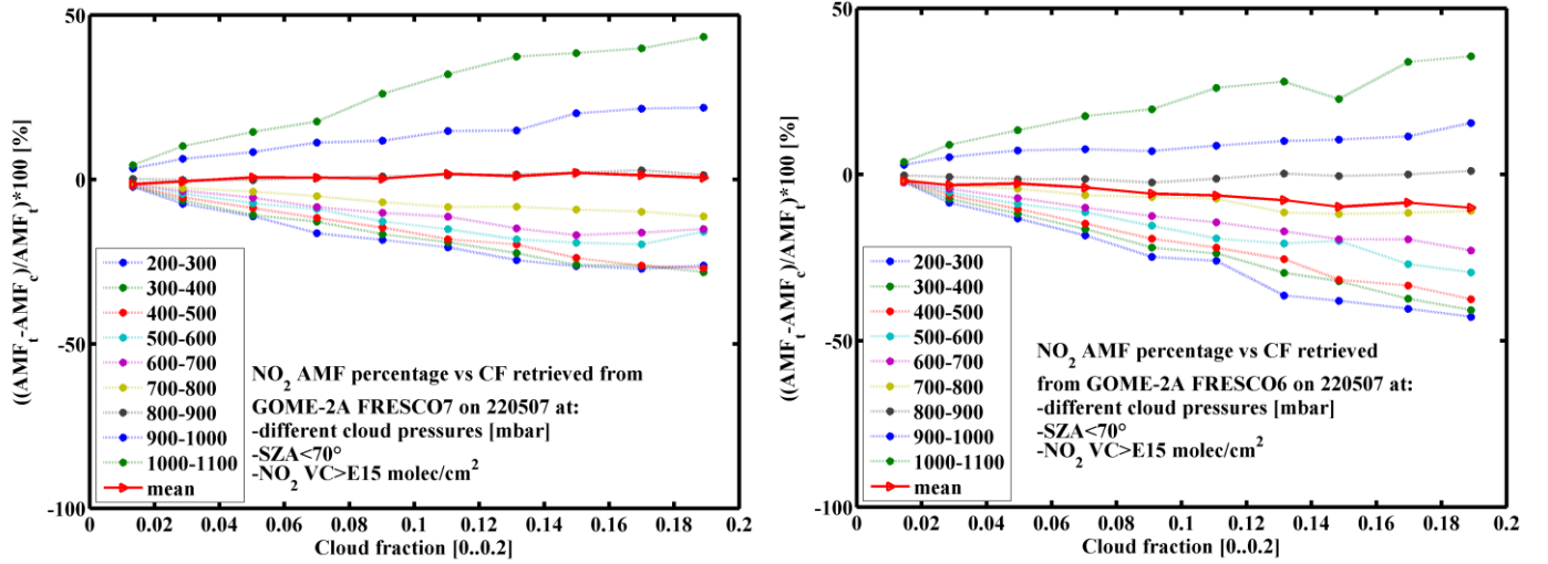
Figure 5.4: The effect of cloud correction on the tropospheric NO_2 AMF for cloud fraction <0.2 at different cloud pressures from GOME-2A using FRESCOv7 (left) FRESCOv6 (right) for a global retrieval on May 22, 2007.
