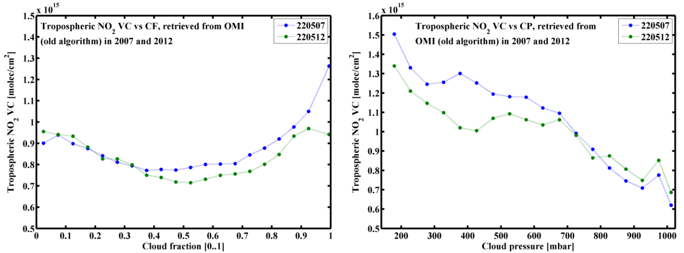
Figure 7.5: Global tropospheric NO 2 VC versus CF (left) and CP (right) over one day of 2007 and 2012.
