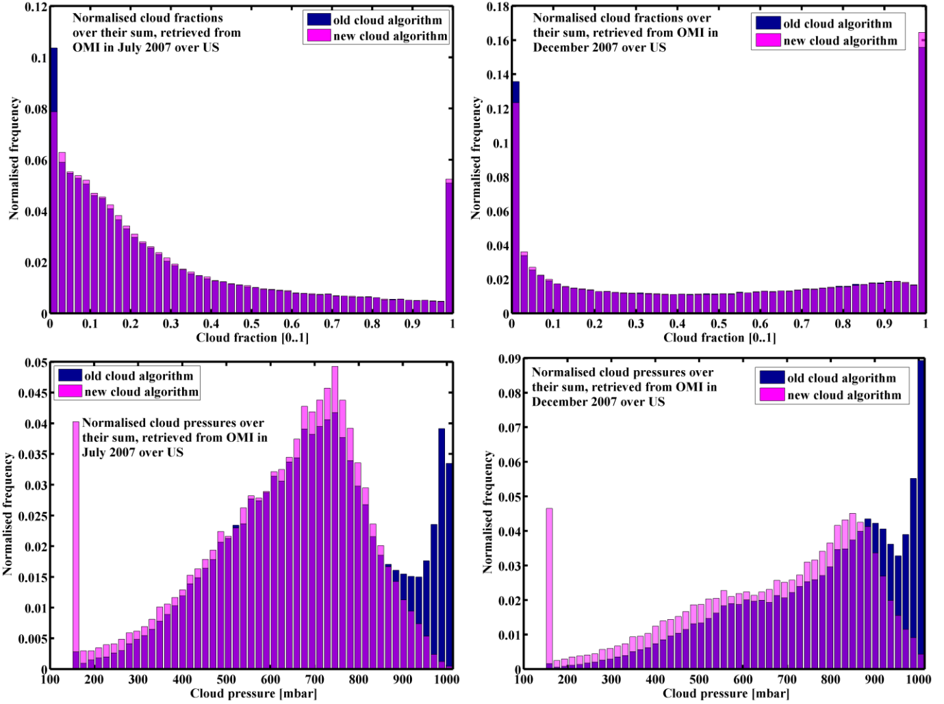
Figure 6.3: The OMI cloud distribution over Eastern US in July (left column) and in December (right column) 2007, CFs (upper row) and CPs (lower row).
