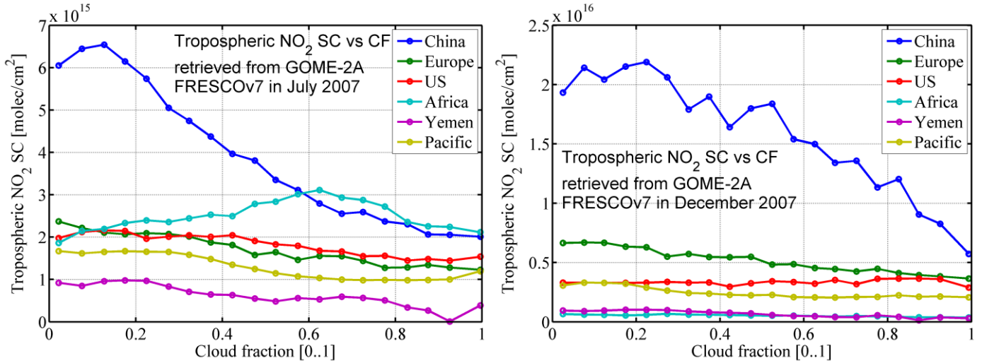
Figure 4.5: Cloud fraction effects on tropospheric \text{NO}_2 slant columns using GOME-2A FRESKOv7 in July (left) and December (right) 2007 over 6 regions
