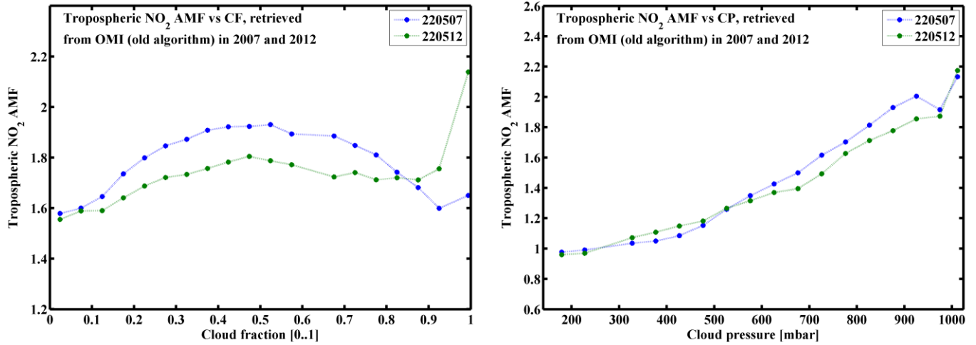
Figure 7.4: Global tropospheric NO 2 AMF versus CF (left) and CP (right) over one day of 2007 and 2012
