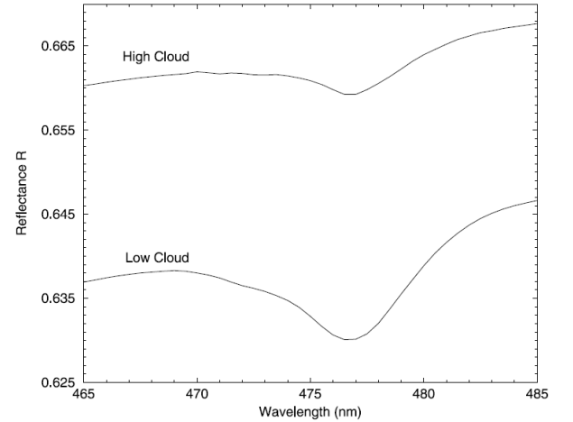
Figure 3.3: A simulated reflectance of the O 2 -O 2 band over the ocean from low and high clouds for a fully cloudy scene (Acarreta et al., 2004).
