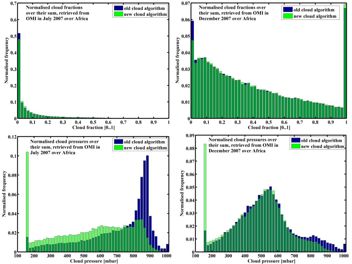
Figure 6.4: The OMI cloud distribution over Central Africa in July (left column) and in December (right column) 2007, CFs (upper row) and CPs (lower row).
