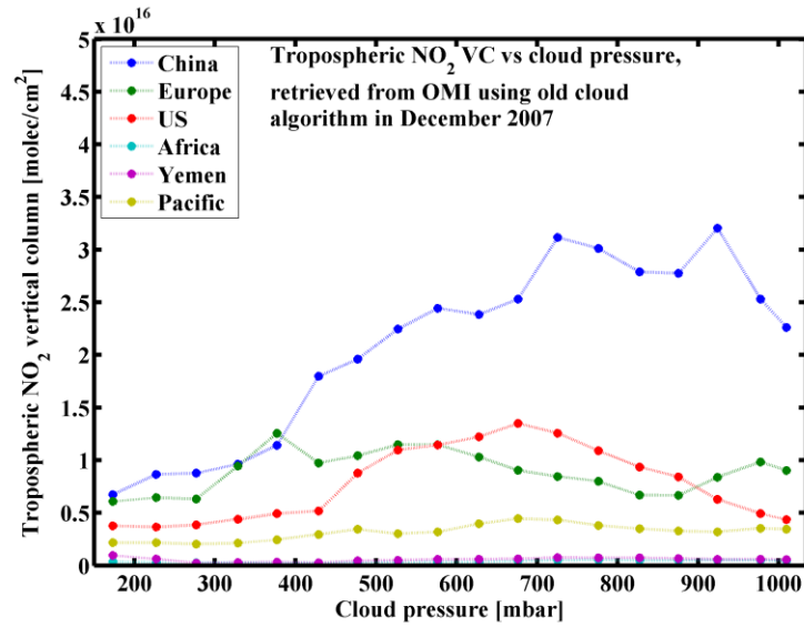
Figure 11.3: Cloud pressure effects on tropospheric NO 2 VC in December 2007 over 6 regions.
