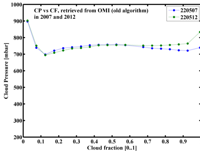
Figure 7.2: Global statistics of cloud fraction and cloud pressure from OMI on one day of 2007 and 2012
