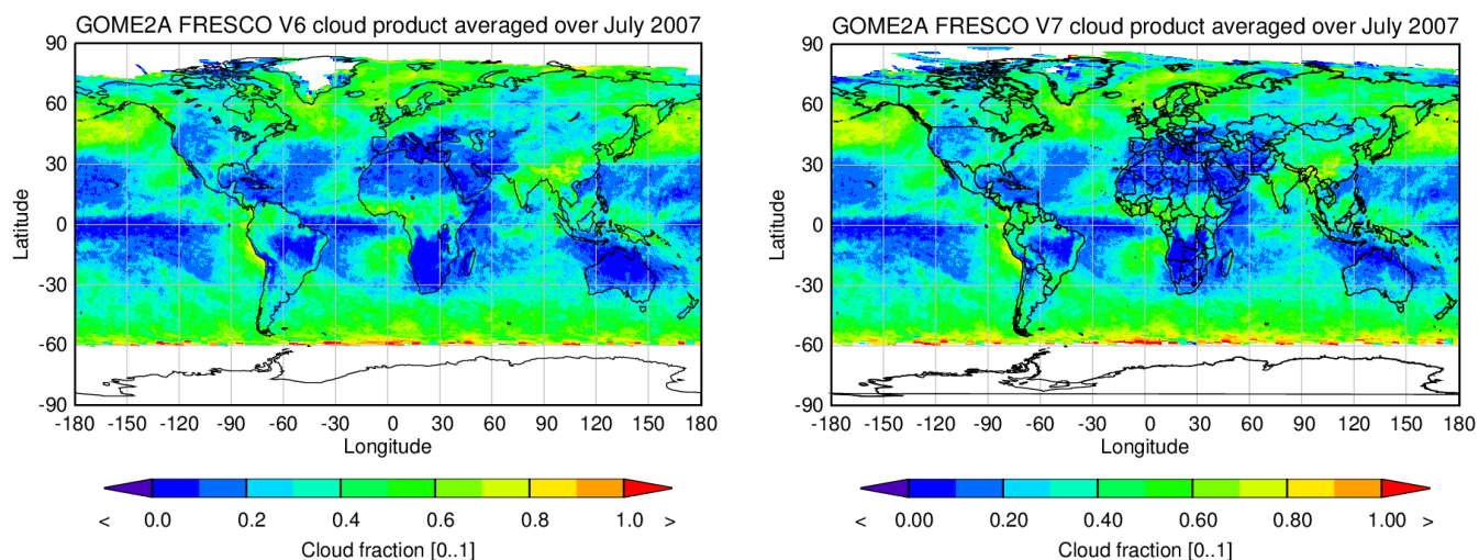
Figure 4.2: Global cloud fraction retrieved by FRESKOv6 and FRESKOv7 algorithms averaged over July, 2007.
