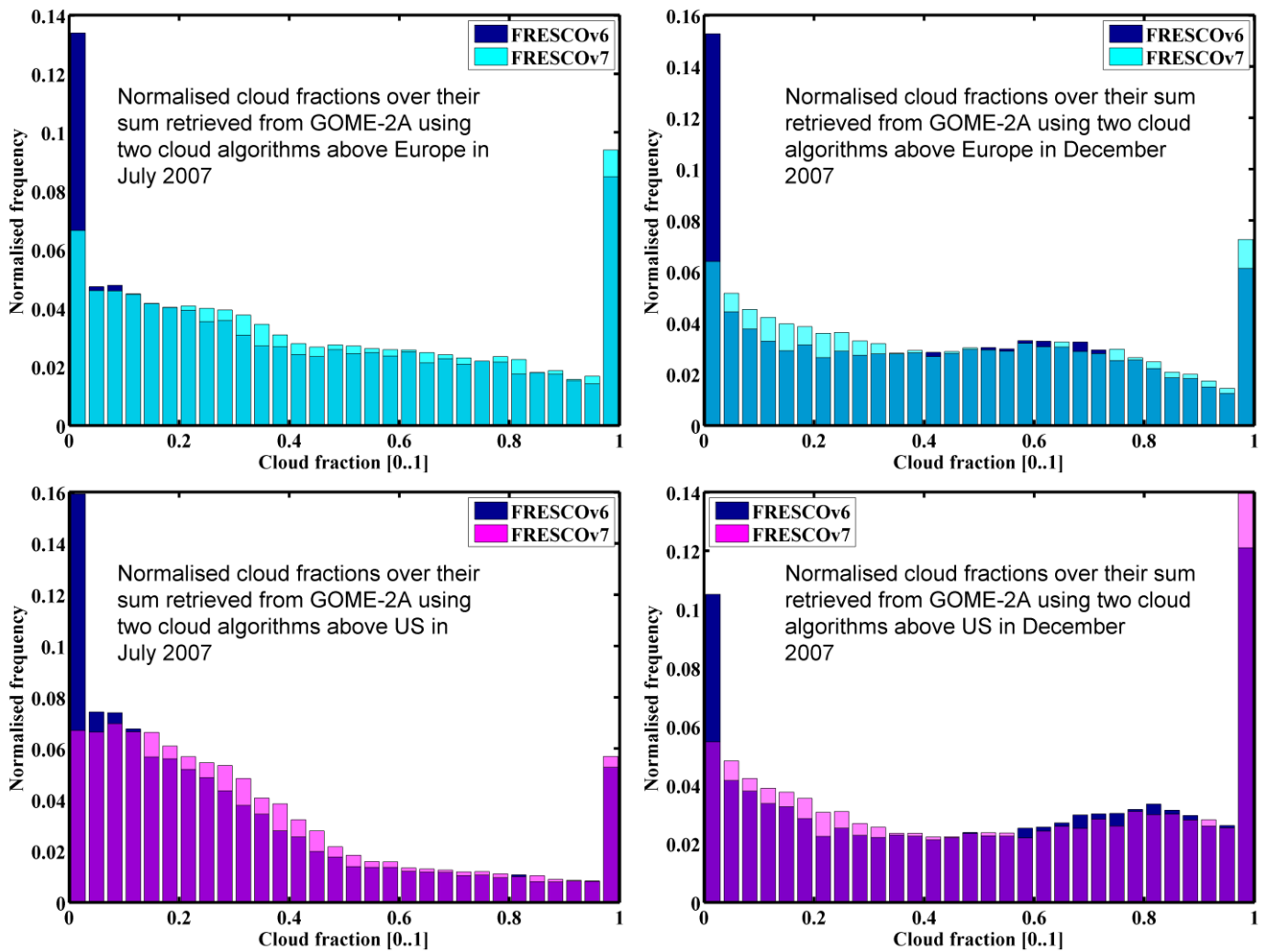
Figure 4.1: Normalised frequencies of cloud fraction from FRESCOv6 and FERSCOv7 algorithms from GOME-2A over Europe and US in July and December 2007.
