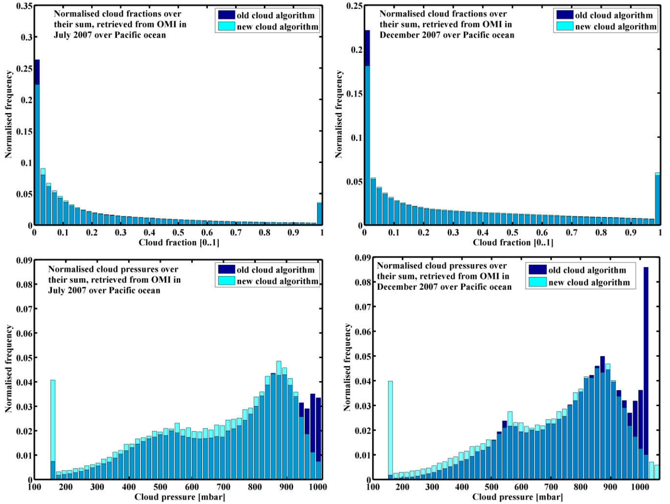
Figure 6.6: OMI cloud distribution over the Northern Pacific Ocean in July (left column) and in December (right column) 2007, CFs (upper row) and CPs (lower row).
