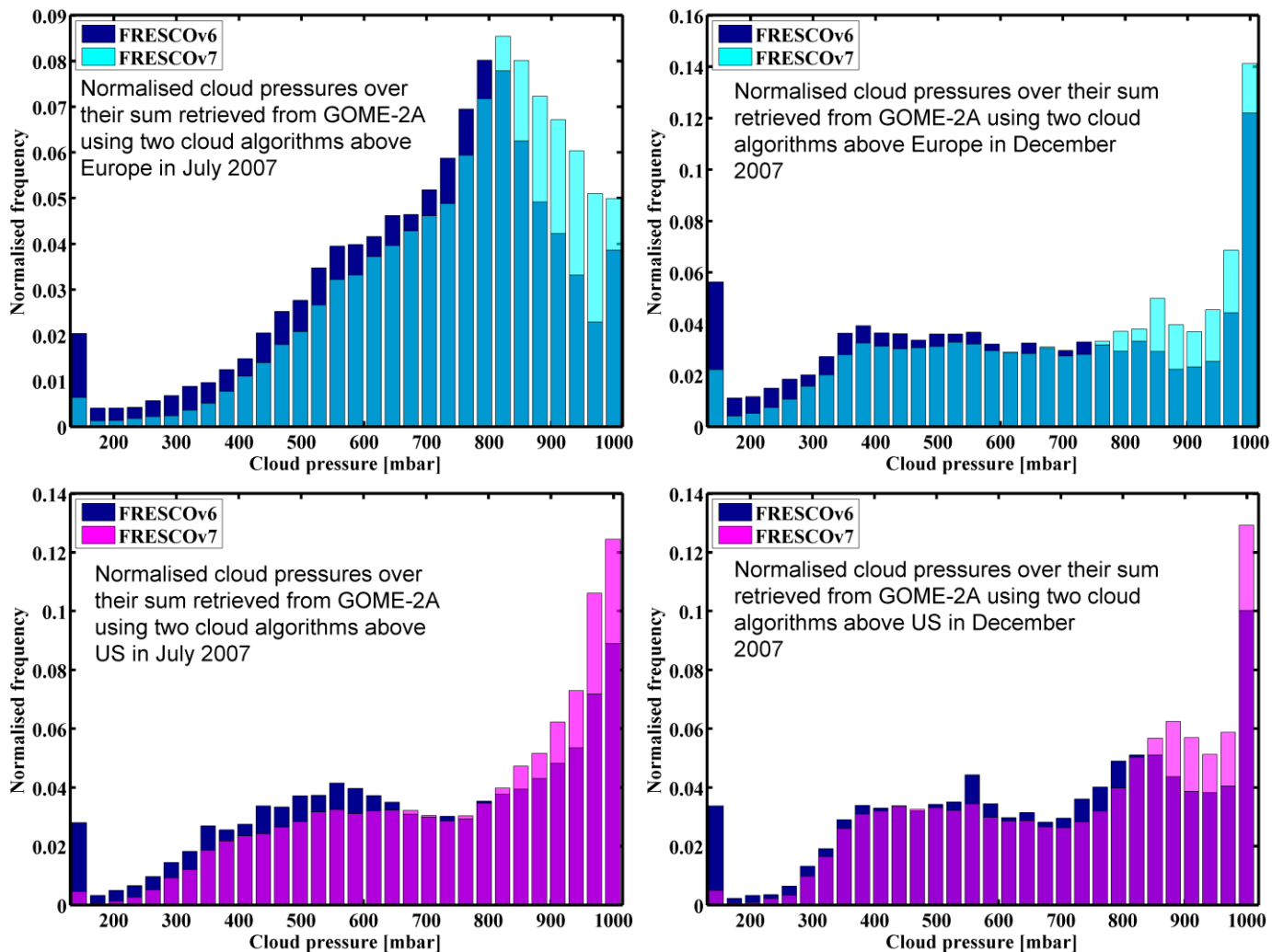
Figure 4.3: Cloud pressure differences between FRESKOv6 and v7 over Europe and the US in July and December 2007.
