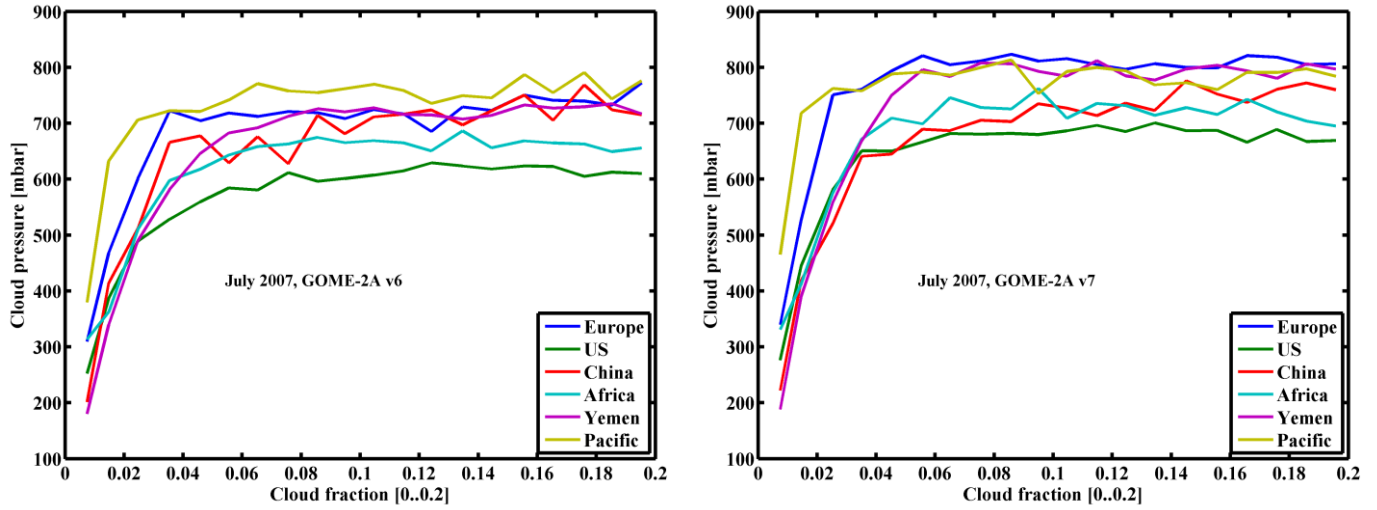
Figure 4.4: The contrast between FRESKOv6 and FRESKOv7 algorithms for cloud parameter at cloud fraction of <0.2 over six regions in July 2007.
