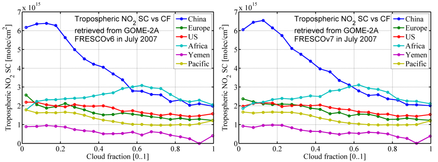
Figure 4.6: A comparison of FRESCOv6 (left) and FRESCOv7 (right) cloud fraction effects on tropospheric \text{NO}_2 SC in July 2007 above 6 regions.
