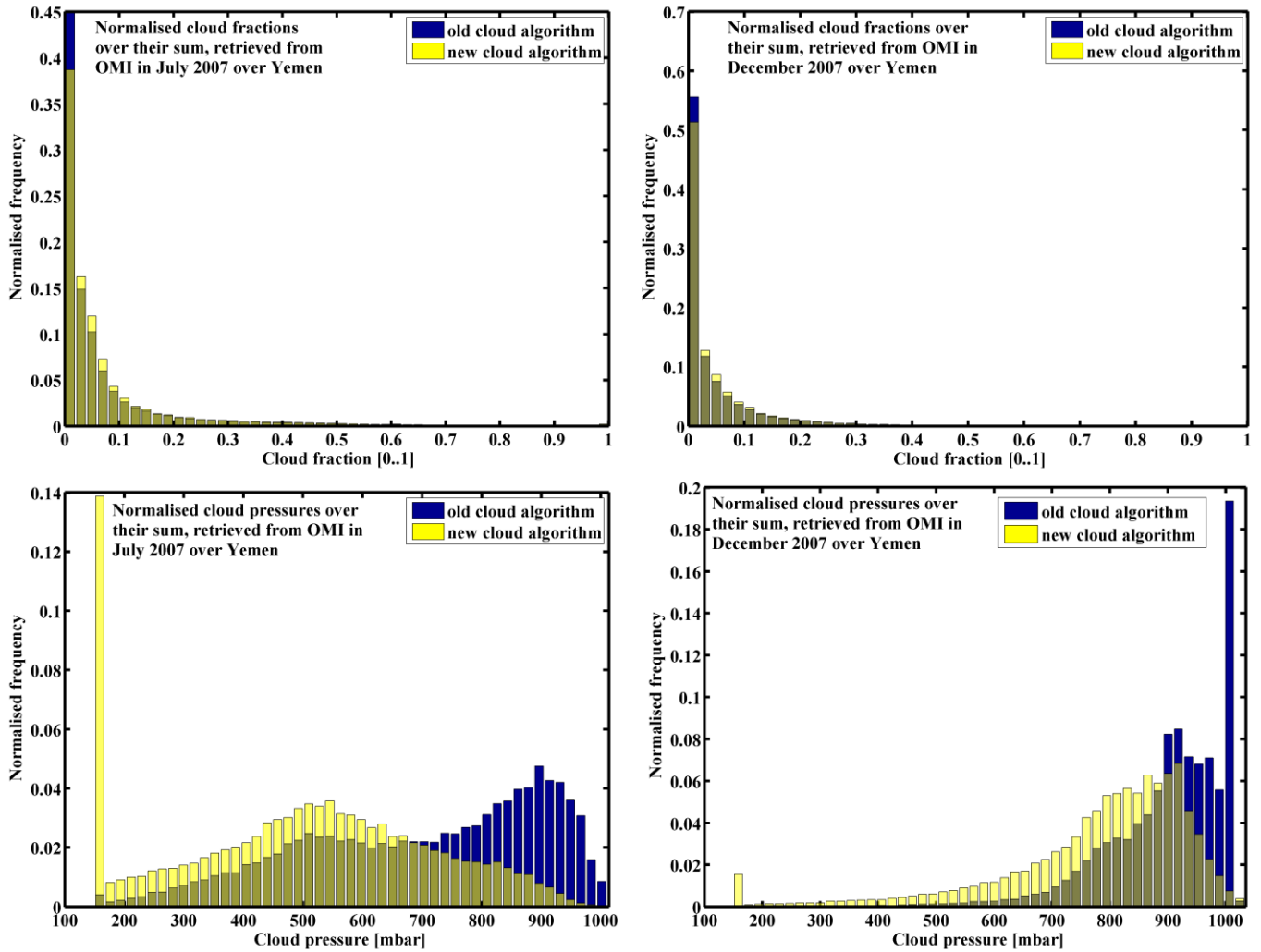
Figure 6.5: OMI cloud distribution over Yemen in July (left column) and in December (right column) 2007, CFs (upper row) and CPs (lower row).
