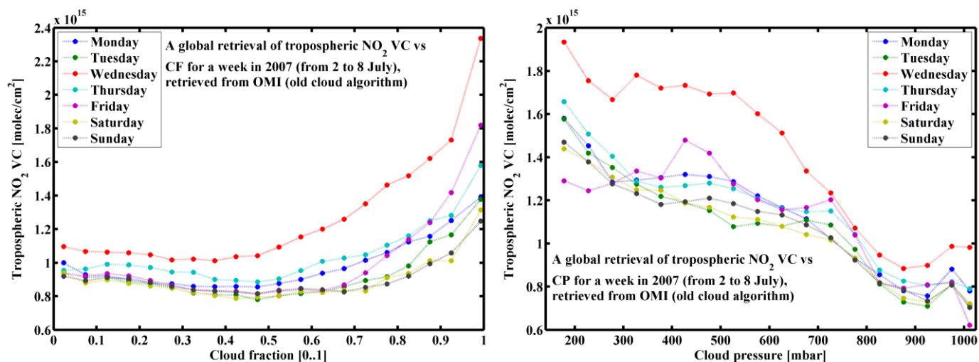
Figure 11.7: Global cloud fraction (left) and cloud pressure (right) impacts on tropospheric \text{NO}_2 VC retrieved from OMI over one week in 2007.
