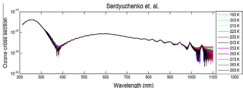
Fig. 8. SER cross-sections [8].
