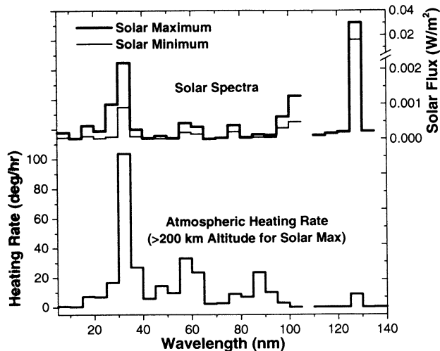
Figure 1. Solar spectra (top curves) for solar minimum and solar maximum and the resulting atmospheric heating rate for solar maximum (bottom curve). Note that the 30.4 nm He II emission produces much of the heating.
