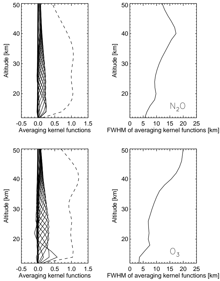
Figure 1. Averaging kernel functions (left) and the full width of half maximum of the averaging kernel functions (right) for a typical N_2O (top panel) and ozone (bottom panel) measurement. The dashed line is the sum of the averaging kernels.
