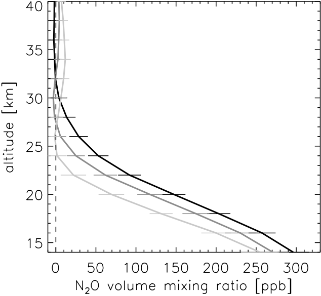
Figure 3. Evolution of ASUR N 2 O measurements during winter 1999/2000. The profiles are an average of all measurements with an equivalent latitude between 70 and 90 degrees for each deployment. Black: December 1999, grey: January 2000, light grey: March 2000. Error bars indicate standard deviation about the mean.
