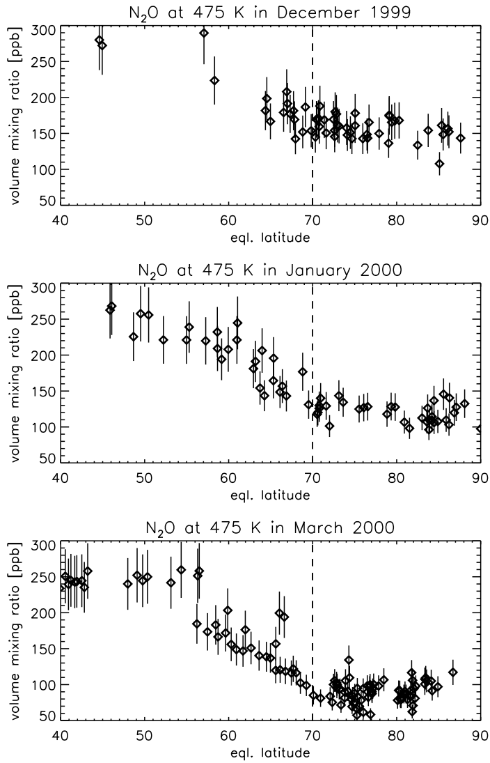
Figure 2. All ASUR N 2 O measurements during winter 1999/2000 as a function of equivalent latitude. N 2 O volume mixing ratios in [ppb] at 475 K of potential temperature are plotted. Top: December 1999, middle: January 2000, and bottom: March 2000. Error bars indicate precision of the single measurement.
