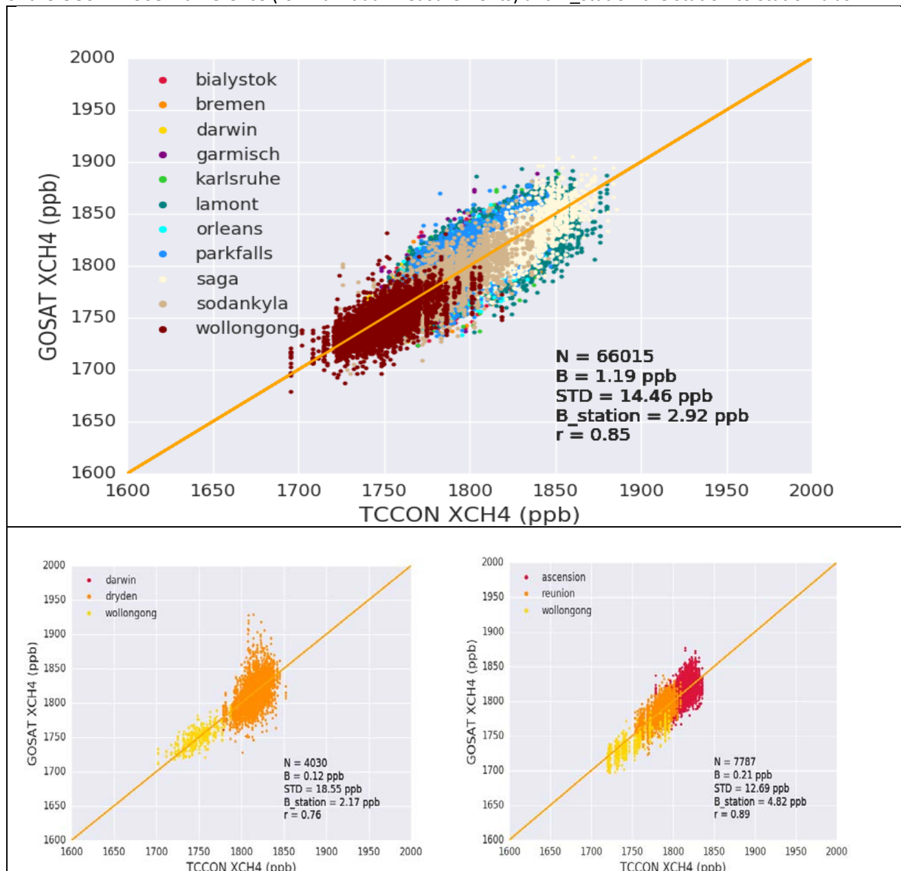
Figure 4: Validation of XCH 4 retrieved by GOSAT-RemoTeC with ground based TCCON measurements for gain H (Top), gain M (bottom left) and sunglint (bottom right) soundings. N(coloc) indicates the number of GOSAT-TCCON collocations, B indicates the bias between GOSAT and TCCON, and STD the standard deviation of the GOSAT TCCON difference (for individual measurements) and B station the station to station bias.
