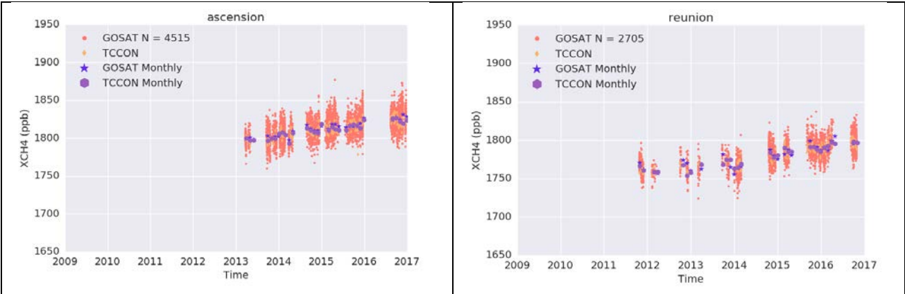
Figure 11: Timeseries for the individual stations for sunglint.
