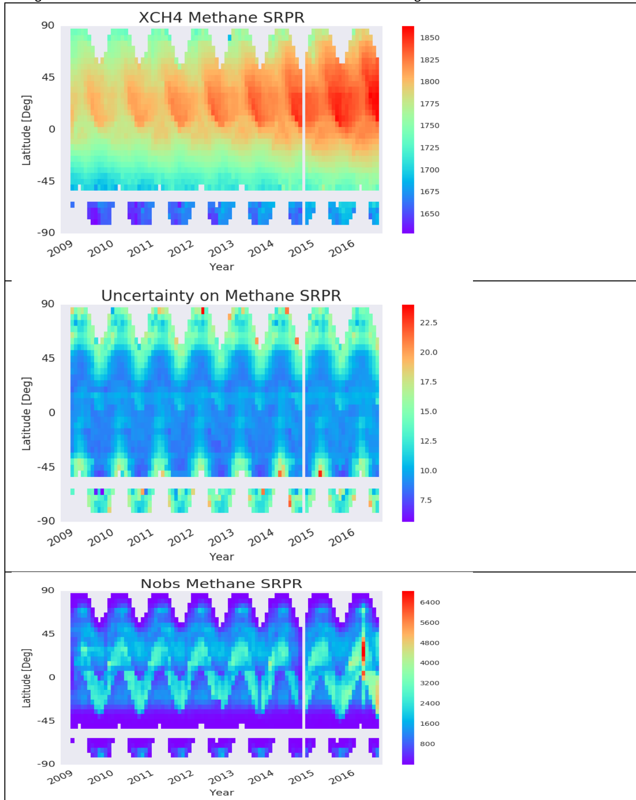
Figure 6: The CH 4 _GOS_SRPR global dataset in slices of 10 degrees latitude as a function of time. The increase in XCH 4 concentrations during the last couple of years can clearly be seen. The gap in data coverage during Dec 2014 and Jan 2015 is due to GOSAT maintenance and testing.
