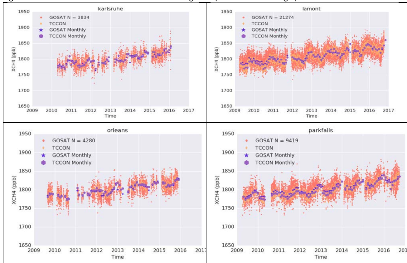
Figure 8: Timeseries for the individual stations for gain H (continued from Fig 6).
