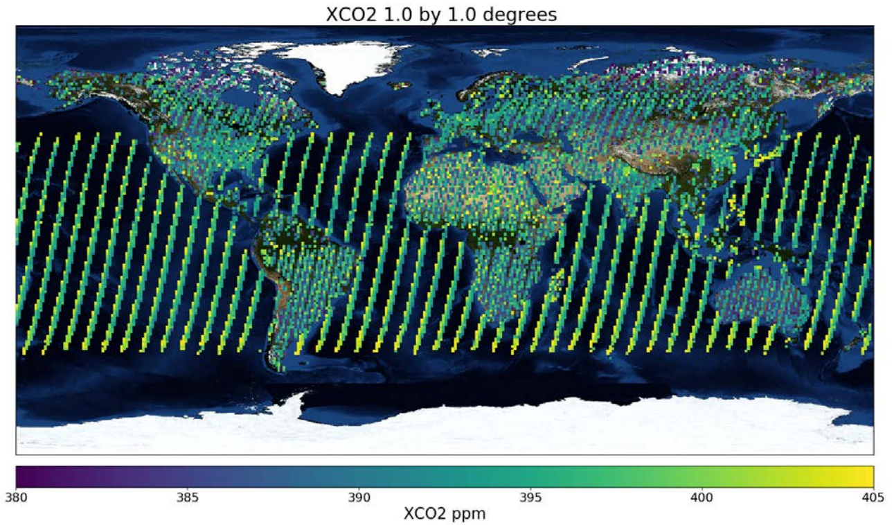
Figure 1: Global XCO 2 for the 2009-2017 period for the CO 2 _GOS_SRFP product on a 1 by 1 degree resolution.
