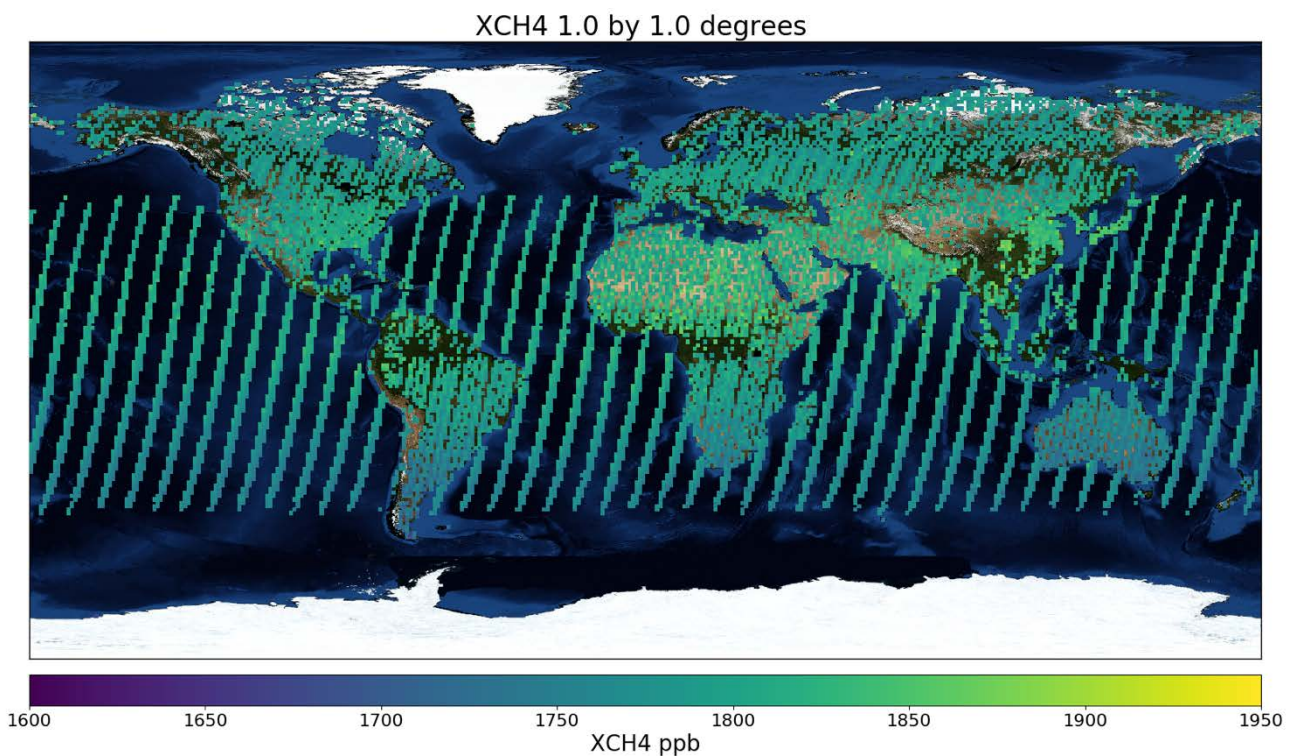
Figure 2: Global XCH 4 for the 2009-2017 period for the CH 4 _GOS_SRFP product on a 1 by 1 degree resolution.
