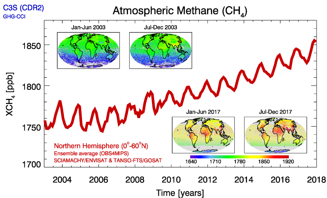
Figure 2 - Overview of the C3S XCH 4 products during 2003-2017 in terms of global maps and time series.
