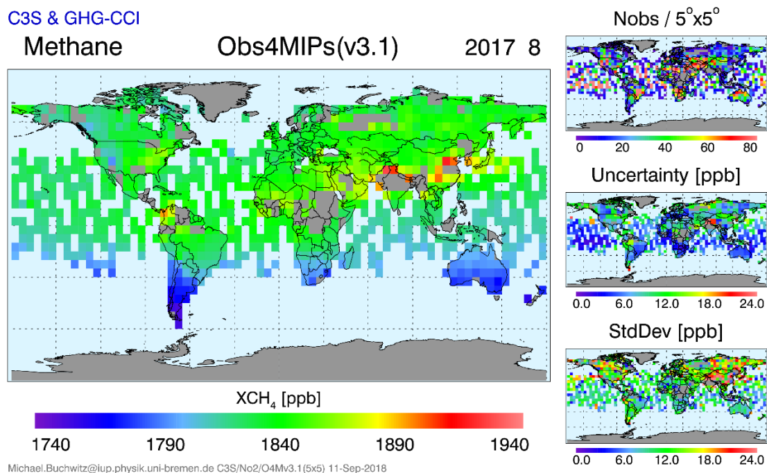
Figure 34 – OBS4MIPS maps for August 2017. Left: XCH 4 . Right: Number of observations (top), reported uncertainty (middle) and standard deviation of the individual observations contributing to each 5°x5° grid cell (bottom).
