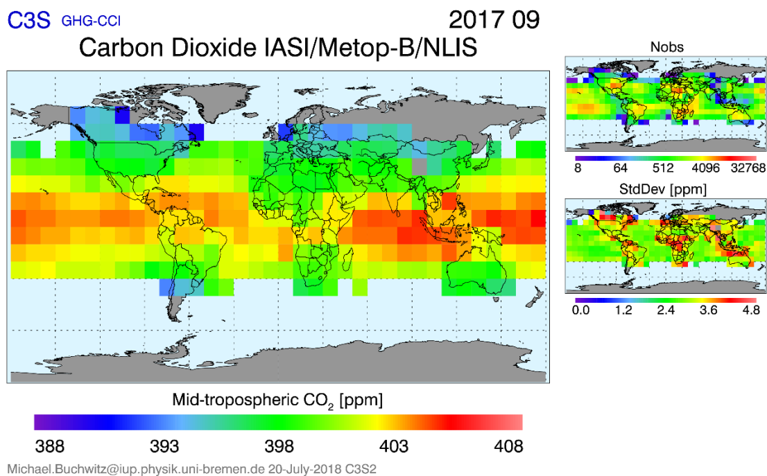
Figure 22 - Map of mid-tropospheric CO 2 from IASI/Metop-B for September 2017 (left). Right: Number of observations per 10°x10° grid size (top) and standard deviation (bottom).
