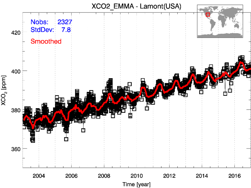
Figure 4 – As Figure 3 but for product XCO2_EMMA.
