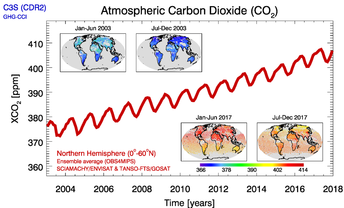
Figure 1 - Overview of the C3S XCO 2 products during 2003-2017 in terms of global maps and time series.
