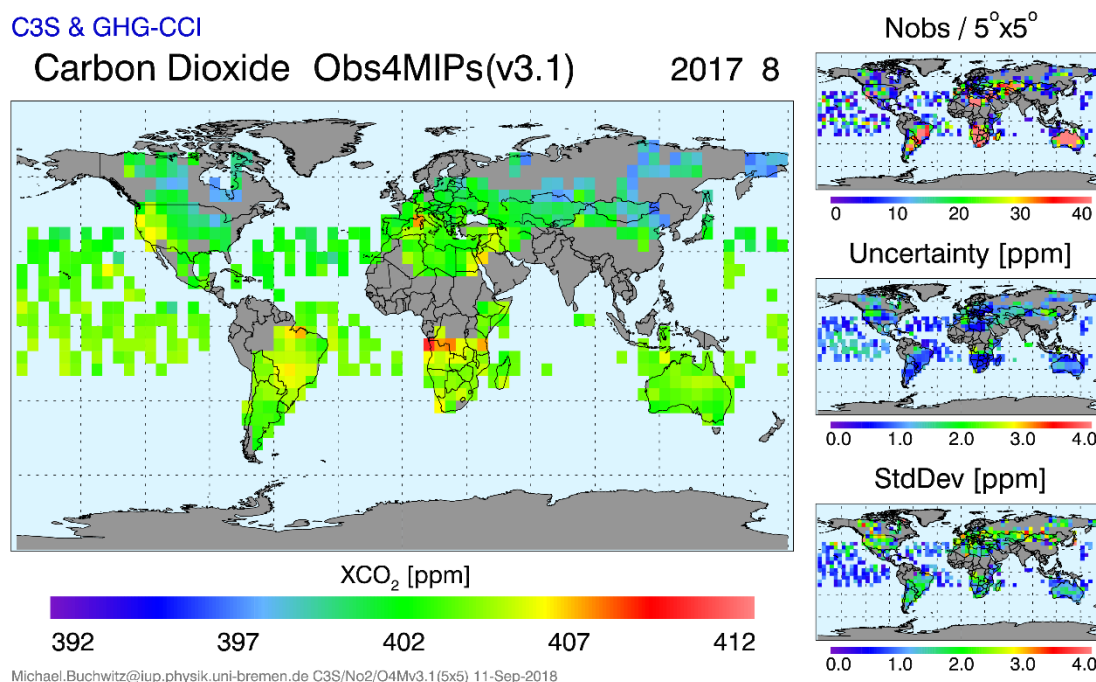
Figure 32 – OBS4MIPS maps for August 2017. Left: XCO 2 . Right: Number of observations (top), reported uncertainty (middle) and standard deviation of the individual observations contributing to each 5°x5° grid cell (bottom).
