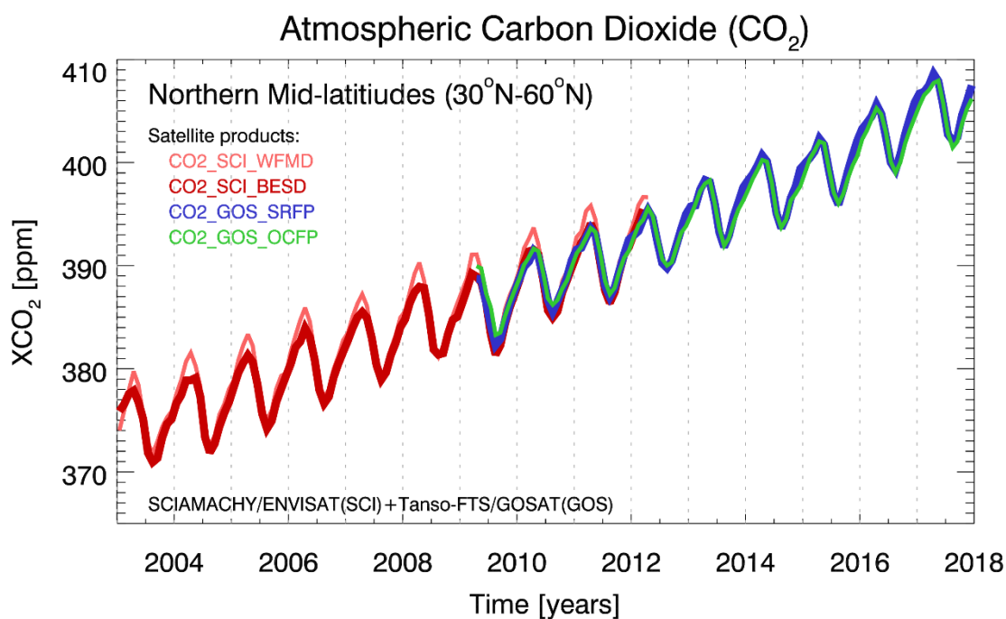
Figure 5 – Satellite-derived northern mid-latitudes XCO 2 time series. Shown are four time series, each corresponding to one of the four individual satellite sensor Level 2 XCO 2 products, which are described in this document.
