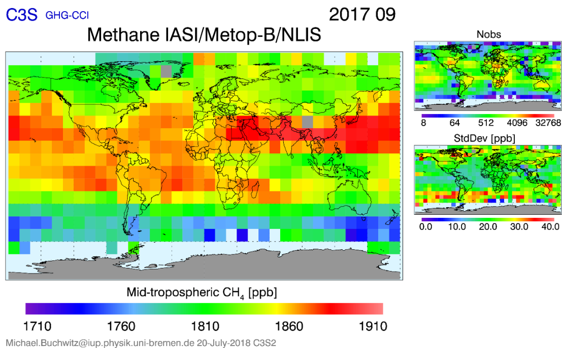
Figure 26 - Map of mid-tropospheric CH 4 from IASI/Metop-B for September 2017 (left). Right: Number of observations per 10°x10° grid size (top) and standard deviation (bottom).
