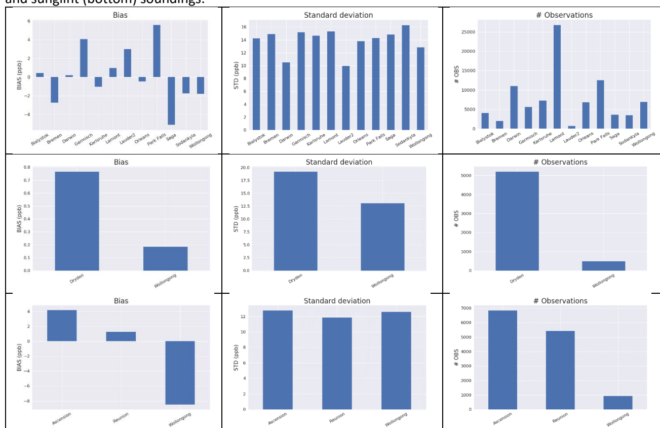
Figure 5: The bias, standard deviation and # of measurements per station for gain H (top), gain M (middle) and sunglint (bottom) soundings.
