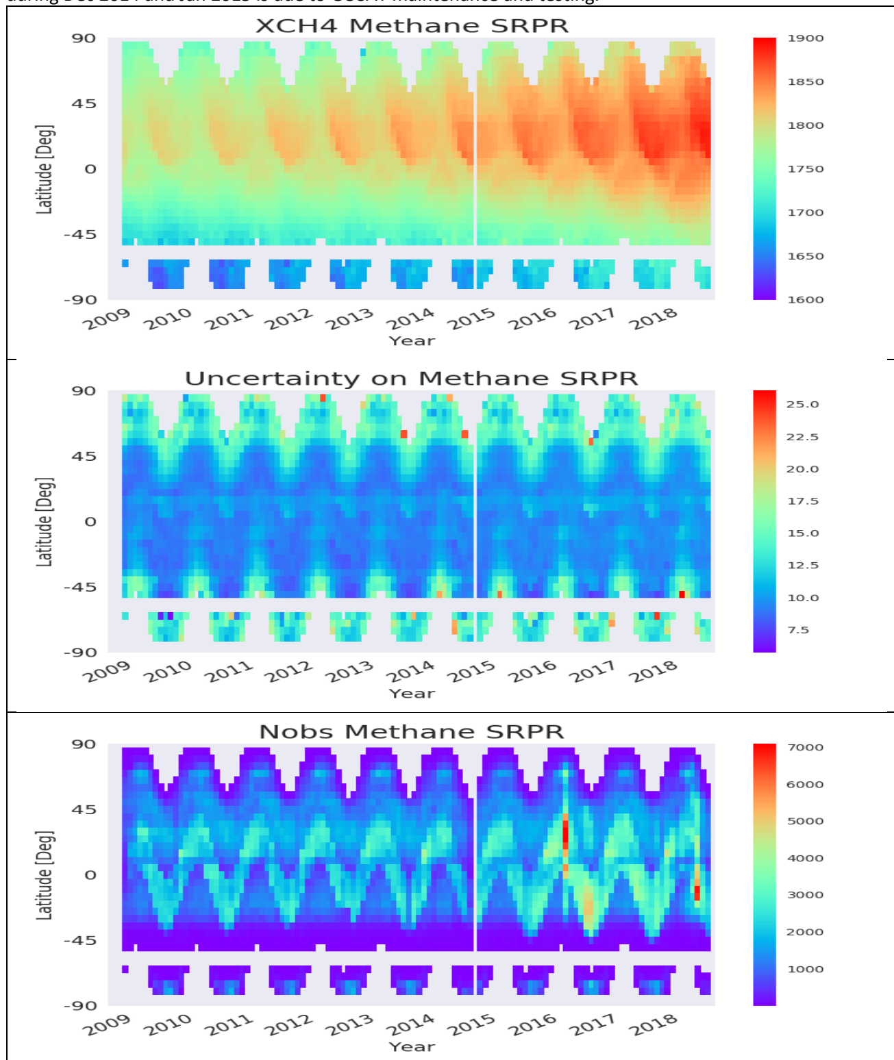
Figure 6: The CH 4 _GOS_SRPR global dataset in slices of 10 degrees latitude as a function of time. The increase in XCH 4 concentrations during the last couple of years can clearly be seen. The gap in data coverage during Dec 2014 and Jan 2015 is due to GOSAT maintenance and testing.
