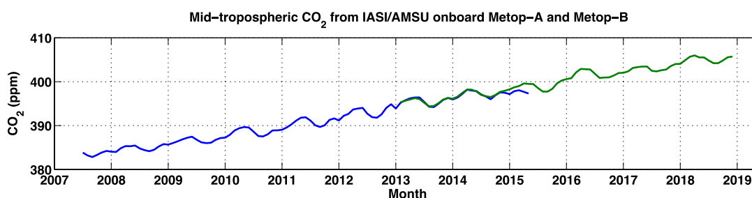
Figure 3: Mid-tropospheric CO 2 retrieved from IASI/AMSU onboard Metop-A (blue) between July 2007 and June 2015, and from IASI/AMSU onboard Metop-B (green) between February 2013 and December 2018.
