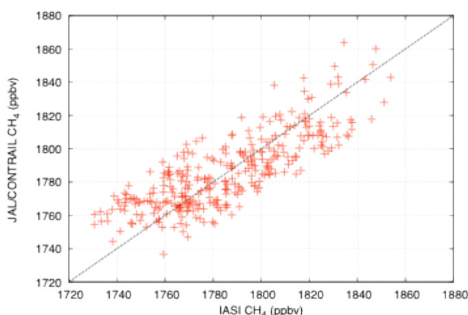
Figure 4: CONTRAIL CH 4 vs. IASI CH 4 for all CONTRAIL measurements over July 2007-December 2014. The 1x1 line is shown as black. Difference between CONTRAIL and IASI CH 4 is -0.89 \pm 16.13 ppb, with a correlation R factor of 0.81.
