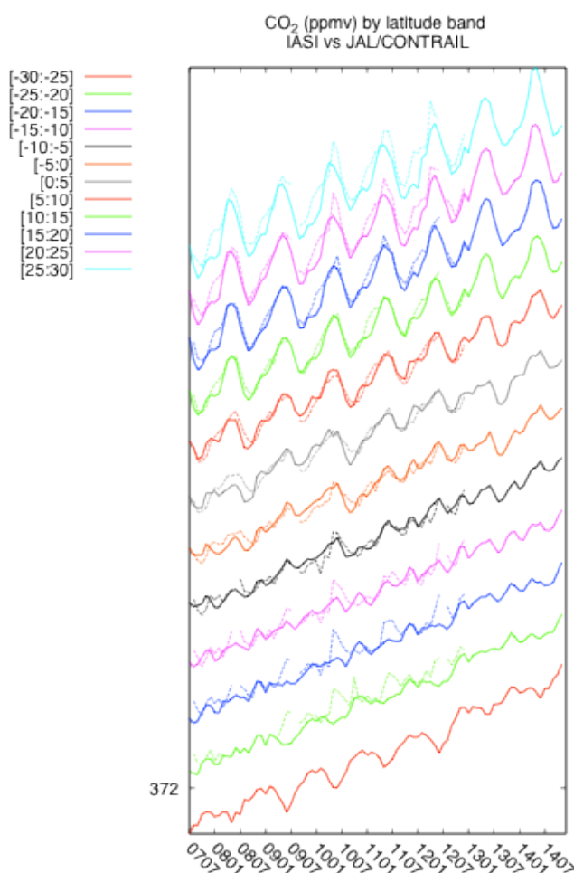
Figure 1: Monthly variation of IASI mid-tropospheric CO 2 V4.0 (full line) and of CONTRAIL CO 2
