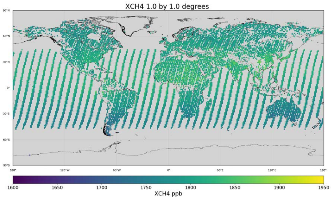
Figure 2: Global XCH 4 for the 2009-2018 period for the CH 4 _GOS_SRFP product on a 1 by 1 degree resolution.
