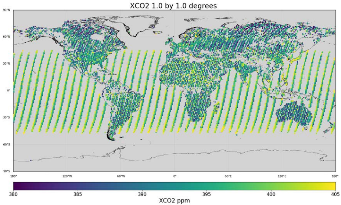
Figure 1: Global XCO 2 for the 2009-2018 period for the CO 2 _GOS_SRFP product on a 1 by 1 degree resolution.
