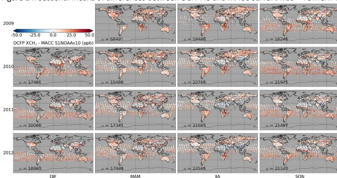
Figure 14: Seasonal means of differences between OCFP7.3 and MACC S1NOAAv10 + TOMCAT \text{XCH}_4 .
