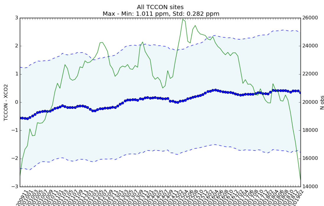
Figure 6: Year-to-year Stability of the TCCON-OCFPv7.3 XCO 2 bias calculated with \pm 6 month averaging window for each month of the GOSAT time series between April 2009 and December 2019, using the T700 co-location method. The thick blue symbols give the mean bias for a 12 month period and the shaded area indicates the standard deviation (1-sigma) of the data. The green lines give the number of data points per 12 month period.
