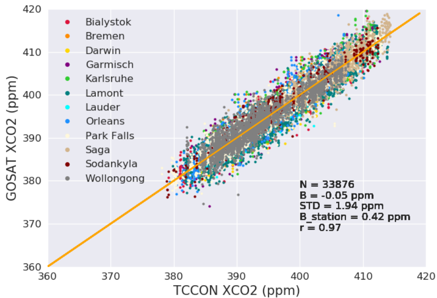
Figure 4: Co-located GOSAT-TCCON XCO2 measurements for gain H measurements
