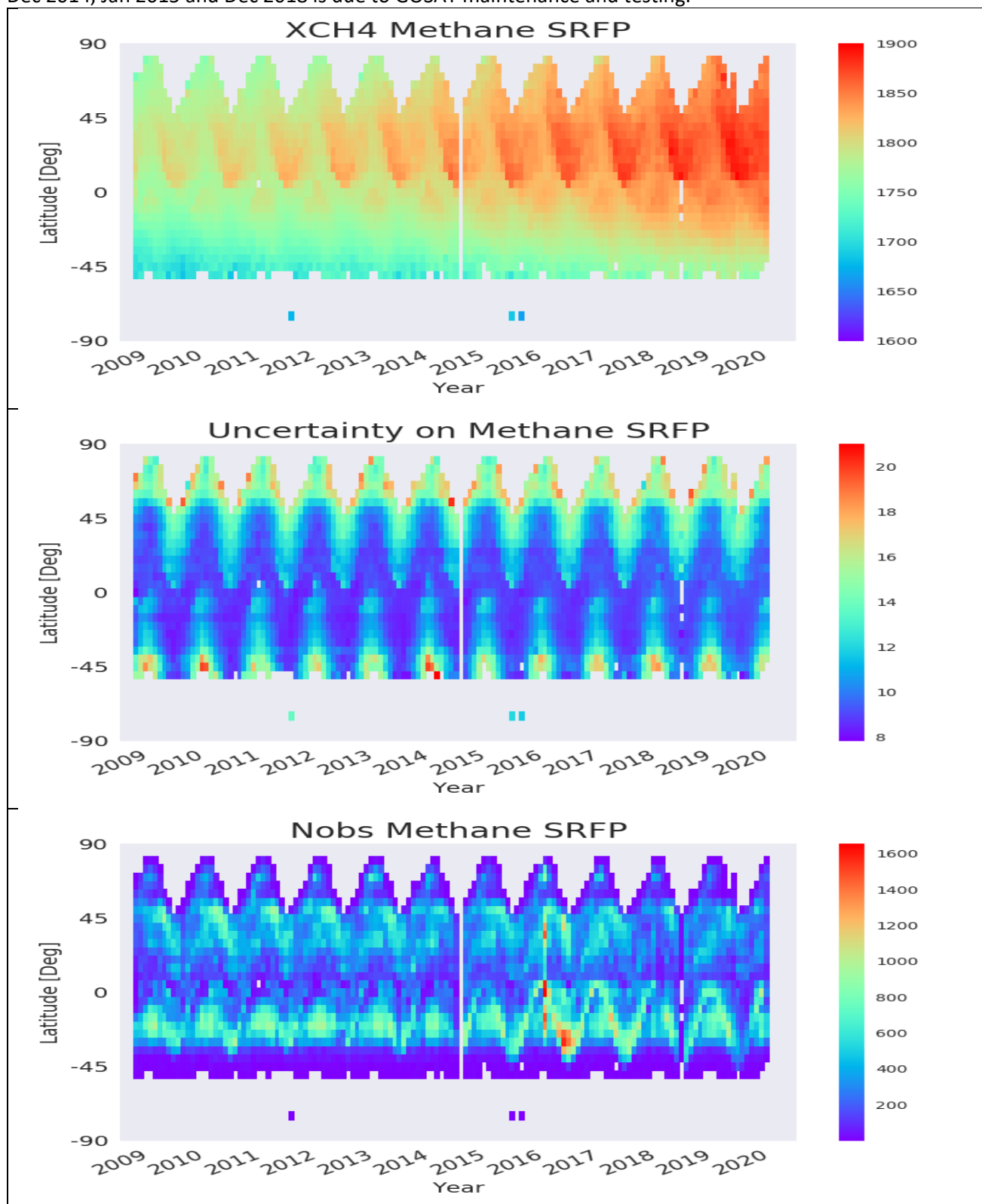
Figure 14: The CH 4 _GOS_SRFP global dataset in slices of 10 degrees latitude as a function of time. The increase in XCH 4 concentrations during the last couple of years can clearly be seen. The gap in data coverage during Dec 2014, Jan 2015 and Dec 2018 is due to GOSAT maintenance and testing.
