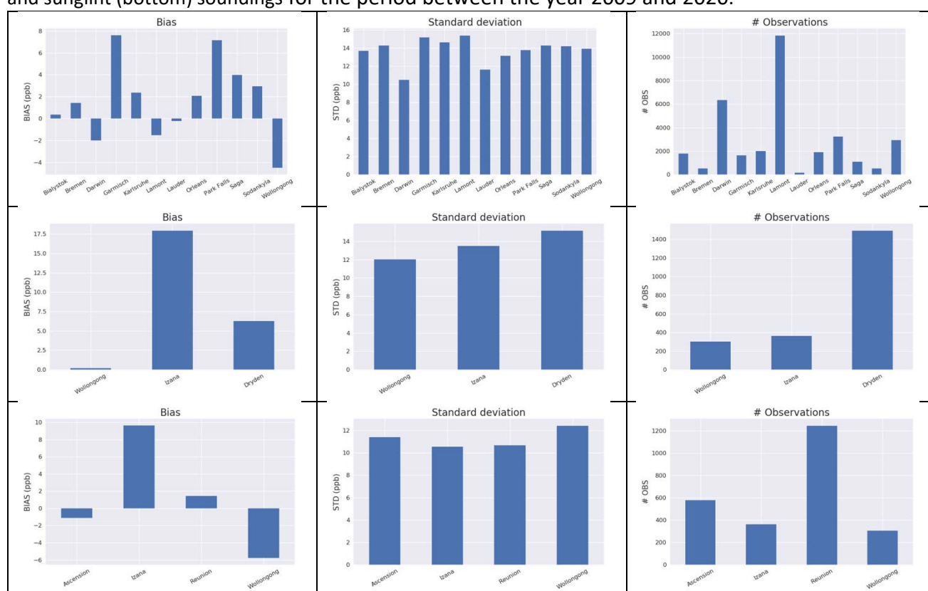
Figure 13: The bias, standard deviation and # of measurements per station for gain H (top), gain M (middle) and sunglint (bottom) soundings for the period between the year 2009 and 2020.
