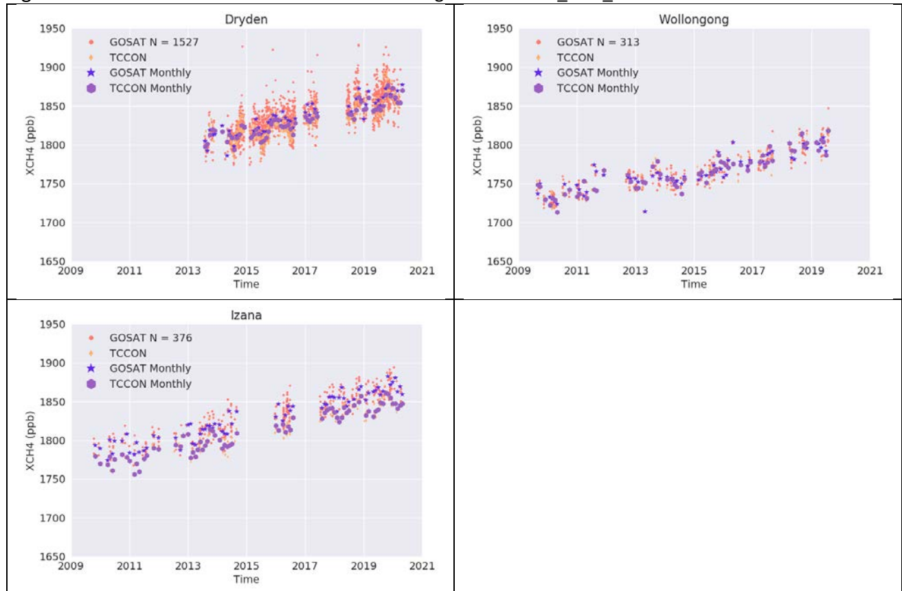
Figure 18: Timeseries for the individual stations for gain M for CH4_GOS_SRFP.
