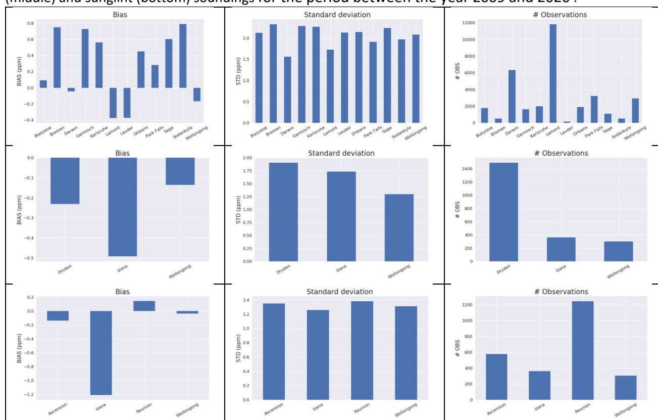
Figure 5: The bias, standard deviation and number of measurements per station for gain H (top), gain M (middle) and sunglint (bottom) soundings for the period between the year 2009 and 2020 .
