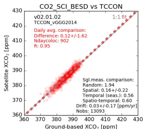
Figure 10 - Product Quality Summary Figure for product CO2_SCI_BESD. Please see the main text for a detailed explanation.
