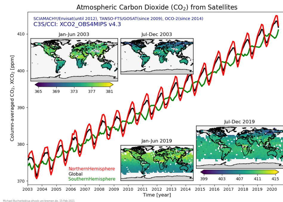
Figure 1 - Overview of the C3S XCO 2 product during 2003-mid2020 in terms of global maps and time series.
