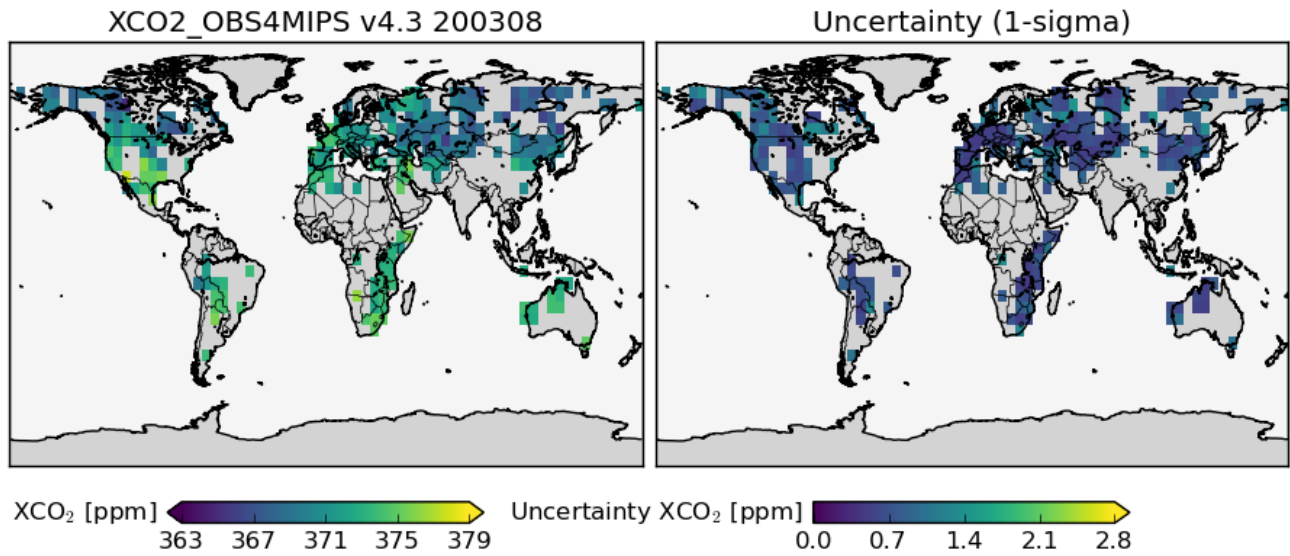
Figure 31 –OBS4MIPS XCO 2 (left) and corresponding uncertainty (right) for August 2003.
