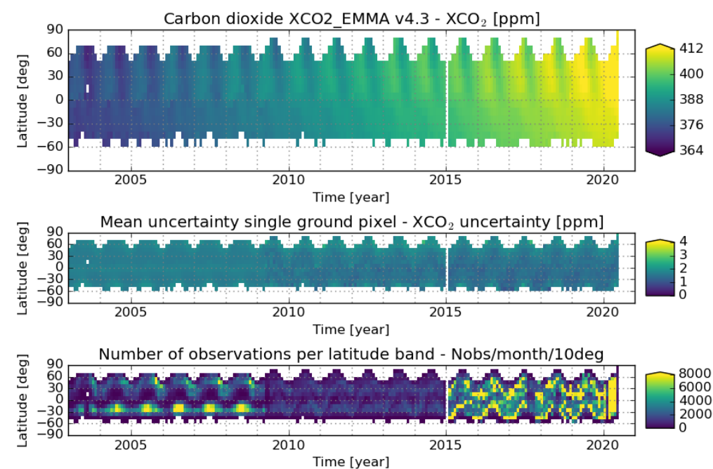
Figure 17 – Latitude – time plot of XCO 2 product XCO 2 _EMMA.
