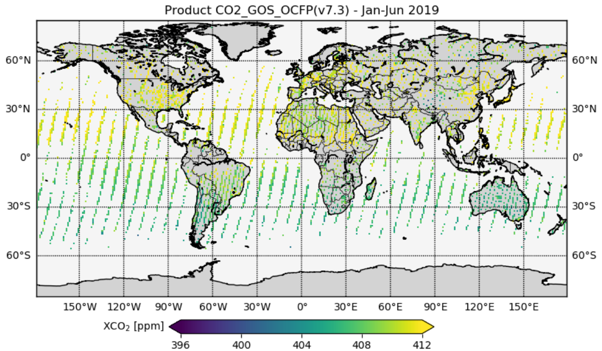
Figure 9 - XCO 2 product CO2_GOS_OCFP. Top: January to June 2019. Bottom: July – December 2019.
