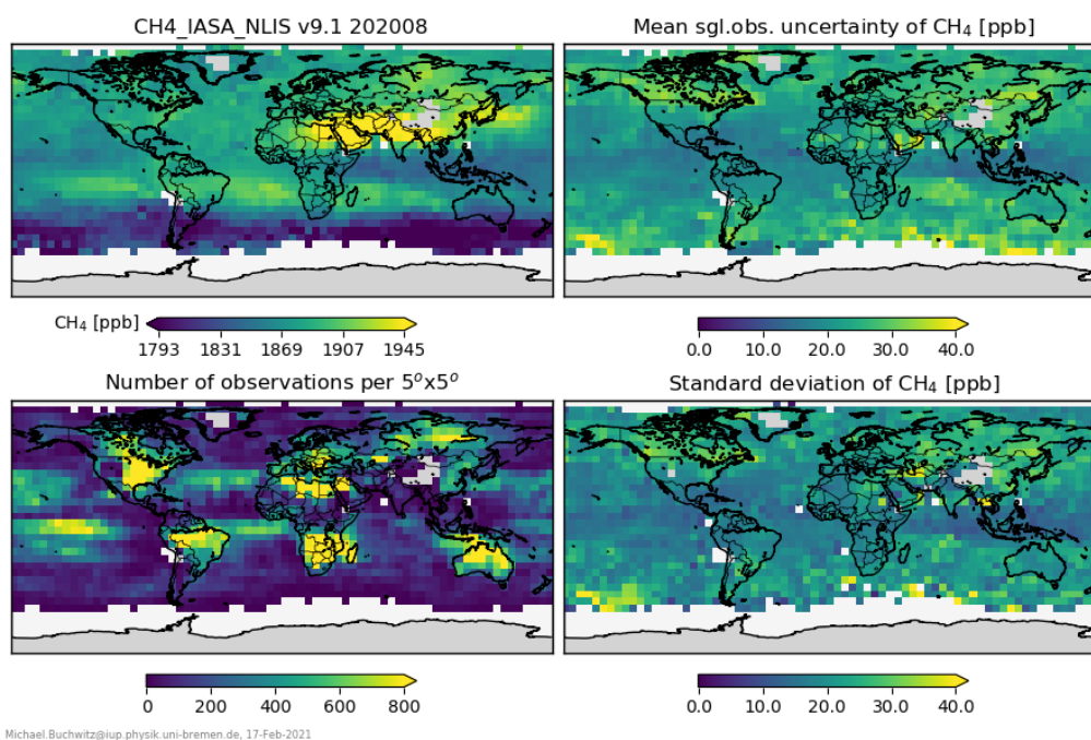
Figure 26 - Map of mid-tropospheric CH 4 from IASI/Metop-B for August 2020 (top left). Mean value of the reported uncertainty (top right), number of observations per 5°x5° grid size (bottom left) and standard deviation (bottom right).
