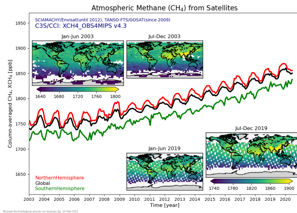
Figure 2 - Overview of the C3S XCH 4 product during 2003-mid2020 in terms of global maps and time series.
