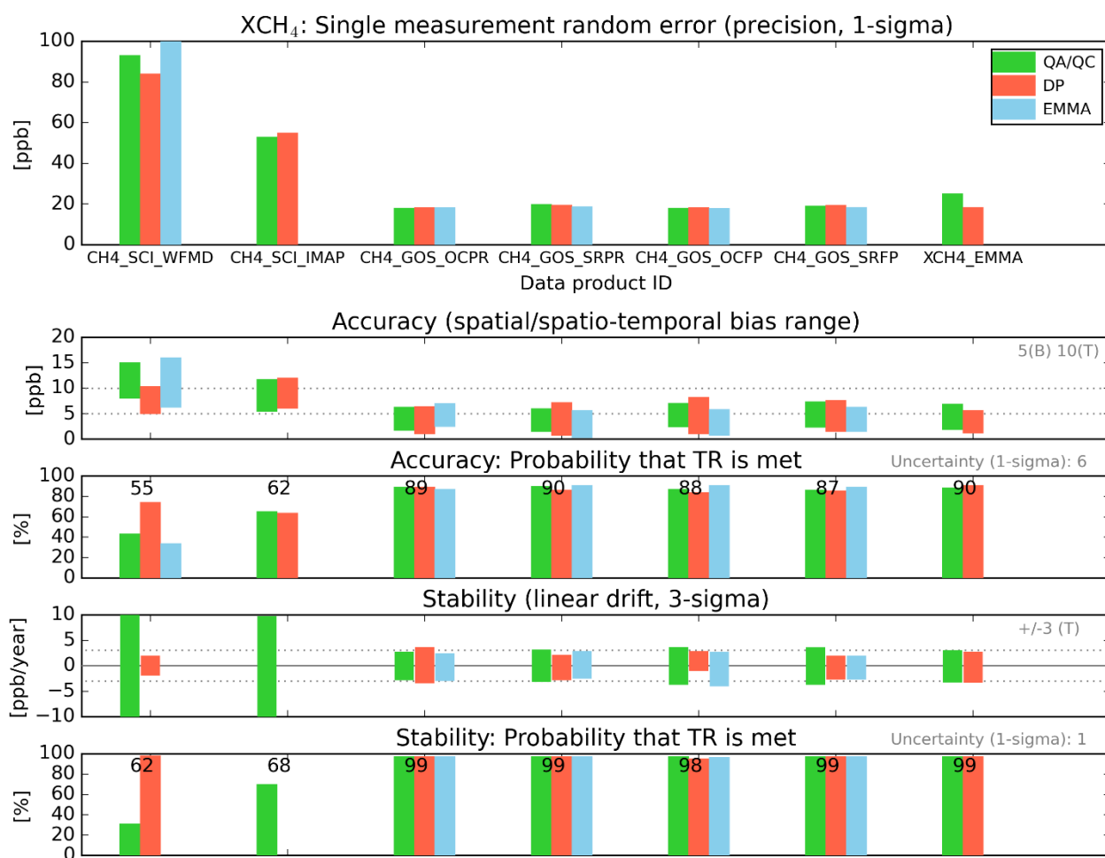
Figure 37 - Overview data quality assessment results for Level 2 XCH 4 data products. The green bars refer to the “Quality Assessment / Quality control” (QA/QC) results as described in this document. The red bars refer to results obtained by the data providers (DPs), as described in separate Annexes (see Sect. 9). For “Accuracy” and “Stability” also the numerical values for the “Probability that TR is met” are given (computed as mean value if more than one value (bar) exists). Also listed (in grey on the right hand side) is the uncertainty of the reference data as used for the Target Requirement (TR) assessments.
