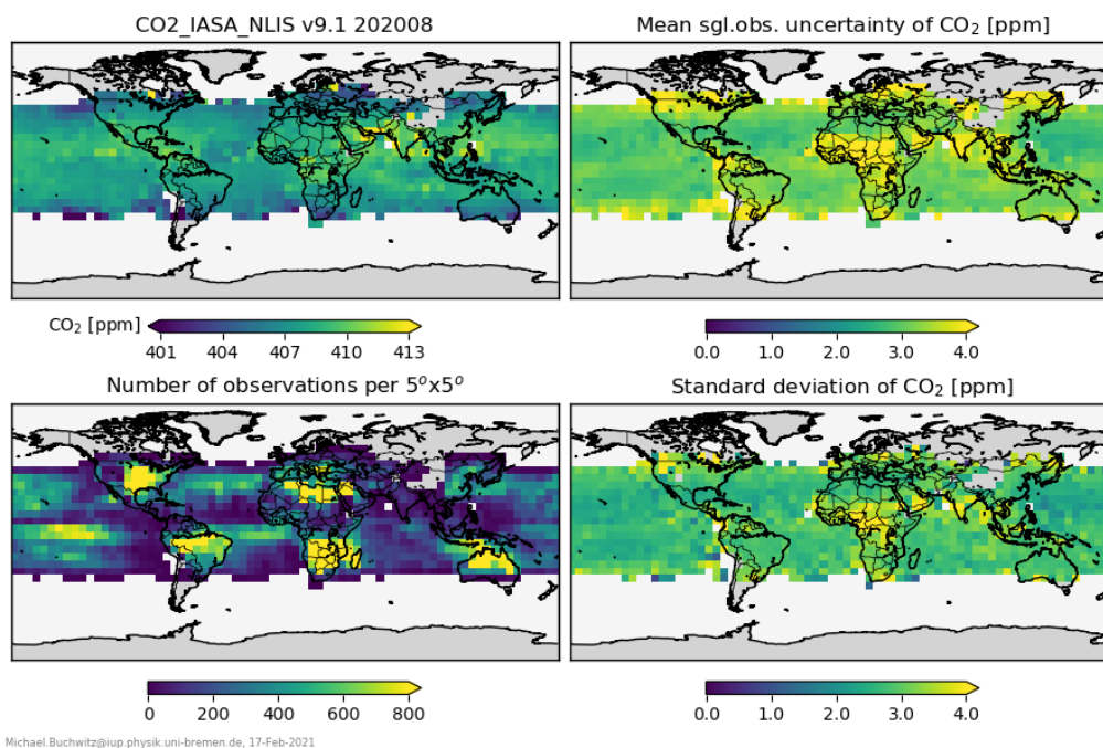
Figure 22 - Map of mid-tropospheric CO 2 from IASI/Metop-B for August 2020 (top left). Mean value of the reported uncertainty (top right), number of observations per 5°x5° grid size (bottom left) and standard deviation (bottom right).
