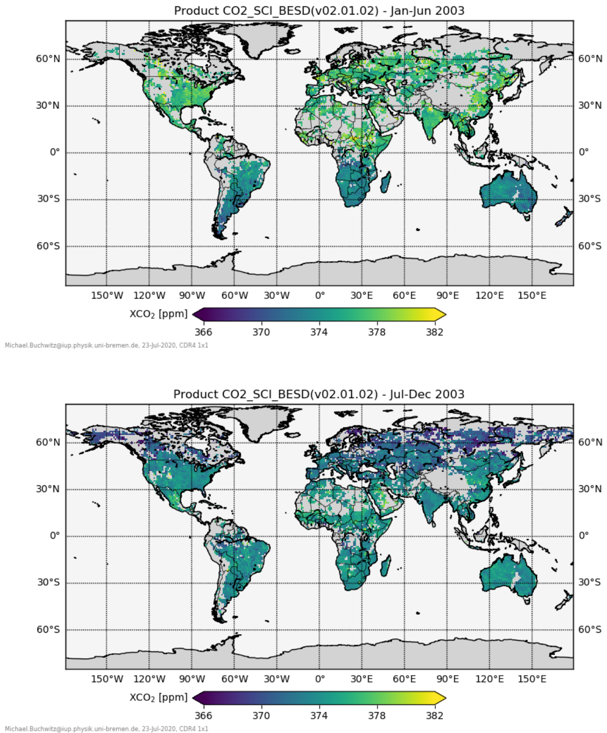
Figure 7 - XCO 2 product CO2_SCI_BESD. Top: January to June 2003. Bottom: July – December 2003.
