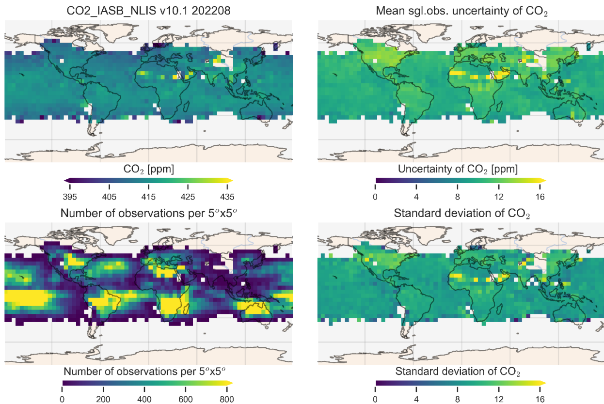
Figure 17 - Map of mid-tropospheric CO 2 from IASI/Metop-B for August 2022 (top left). Mean value of the reported uncertainty (top right), number of observations per 5°x5° grid size (bottom left) and standard deviation (bottom right). Note that the scale for uncertainty and standard deviation (i.e., scatter) has been increased by a factor of 2 compared to the corresponding IASI-A and IASI-C figures (i.e., Figure 16 and Figure 18, respectively).
