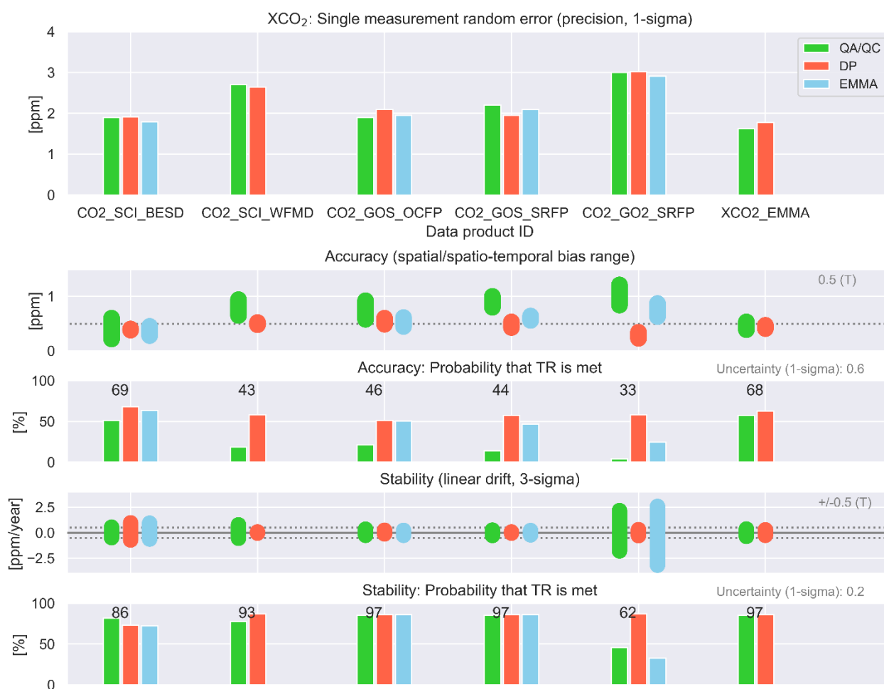
Figure 29 - Overview data quality assessment results for Level 2 XCO 2 data products (from D9). The green bars refer to the “Quality Assessment / Quality control” (QA/QC) results as described in detail in document D9. The red bars refer to results obtained by the data providers (DPs) (see D9). For “Accuracy” and “Stability” also the numerical values for the “Probability that TR is met” are given (computed as mean value if more than one value (bar) exists). Also listed (in grey on the right hand side) is the uncertainty of the reference data as used for the Target Requirement (TR) assessments. The listed values for products generated in previous C3S projects (products CO 2 _SCI_BESD, CO 2 _SCI_WFMD and CO 2 _GOS_SFFP) are listed here for completeness but have not been updated (for details see D9).
