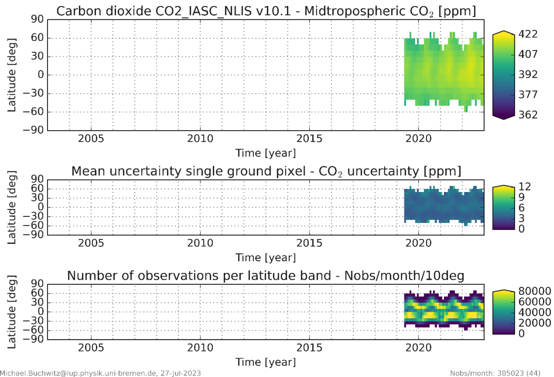
Figure 15 - Mid-tropospheric CO 2 (top) as seen by IASI/Metop-C, reported uncertainty (middle) and number of observations per month and 10 deg latitude band (bottom).
