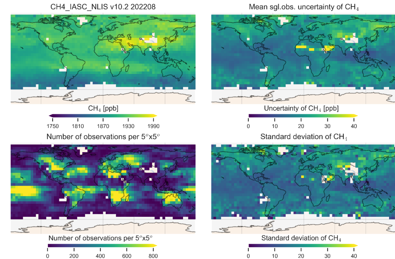
Figure 24 - Map of mid-tropospheric CH 4 from IASI/Metop-C for August 2022 (top left). Mean value of the reported uncertainty (top right), number of observations per 5°x5° grid size (bottom left) and standard deviation (bottom right).
