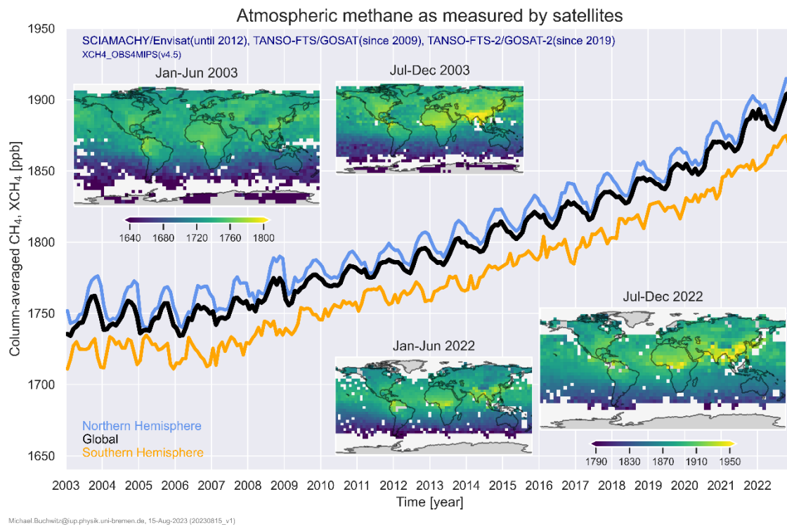
Figure 2 - C3S XCH 4 global maps and time series (product XCH 4 _OBS4MIPS version 4.5).
