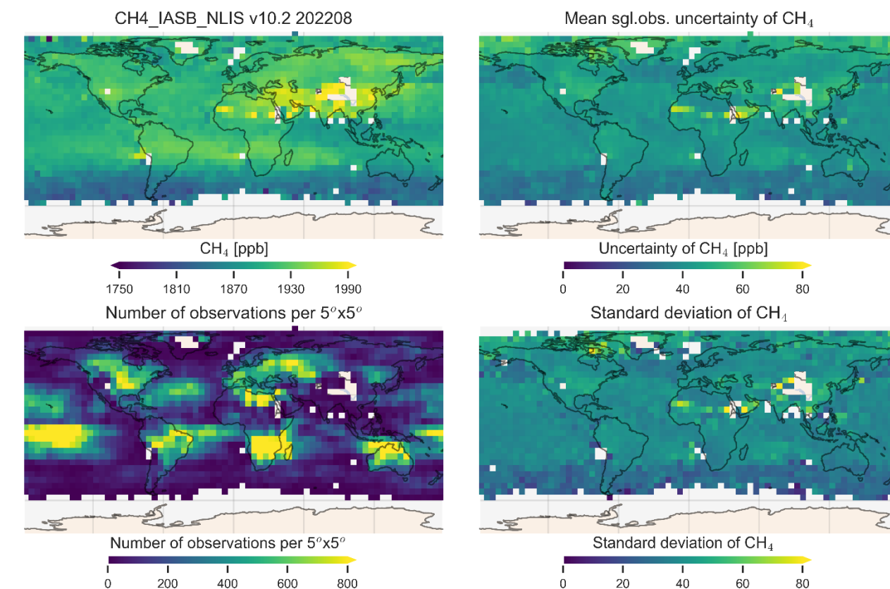
Figure 23 - Map of mid-tropospheric CH 4 from IASI/Metop-B for August 2022 (top left). Mean value of the reported uncertainty (top right), number of observations per 5°x5° grid size (bottom left) and standard deviation (bottom right). Note that the scale for uncertainty and standard deviation (i.e., scatter) has been increased by a factor of 2 compared to the corresponding IASI-A and IASI-C figures (i.e., Figure 22 and Figure 24, respectively).
