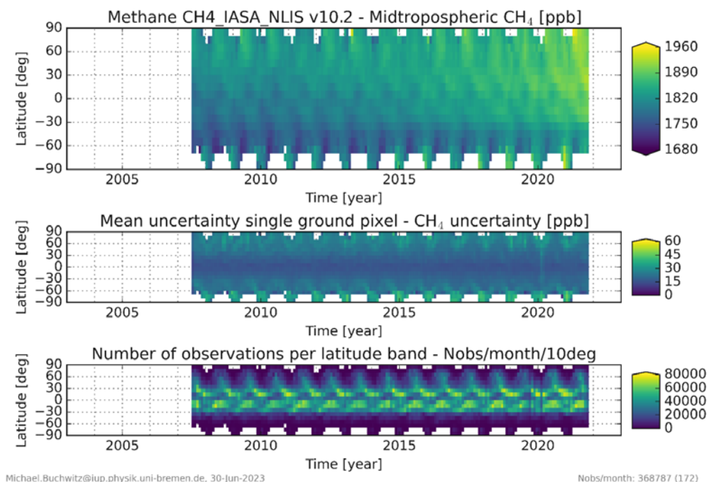
Figure 19 – Mid-tropospheric CH 4 (top) as seen by IASI/Metop-A, reported uncertainty (middle) and number of observations per month and 10 deg latitude band (bottom).
