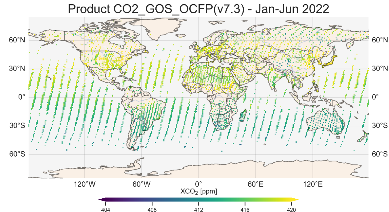
Figure 5 - XCO 2 product CO2_GOS_OCFP. Top: January to June 2022. Bottom: July – December 2022.
