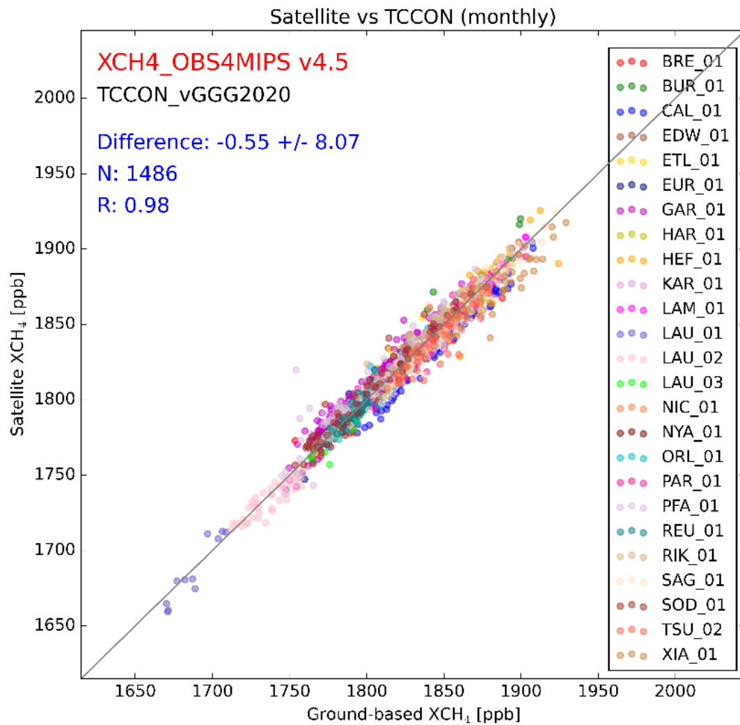
Figure 36 - Overview data quality assessment results for Level 3 XCH 4 Obs4MIPs format data product. Note that each dot corresponds to a given TCCON site and month.
