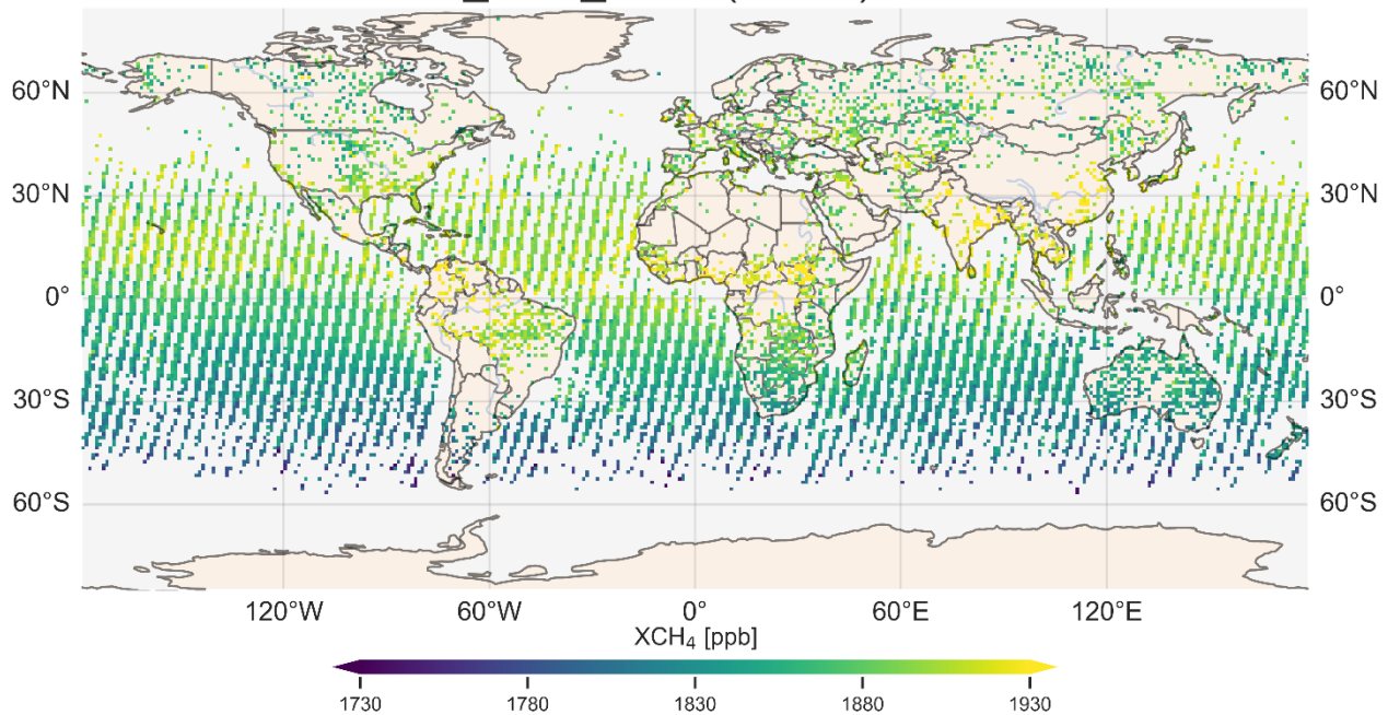
Figure 9 - XCH 4 product CH 4 _GO2_SRFP. Top: January to June 2022. Bottom: July – December 2022.
