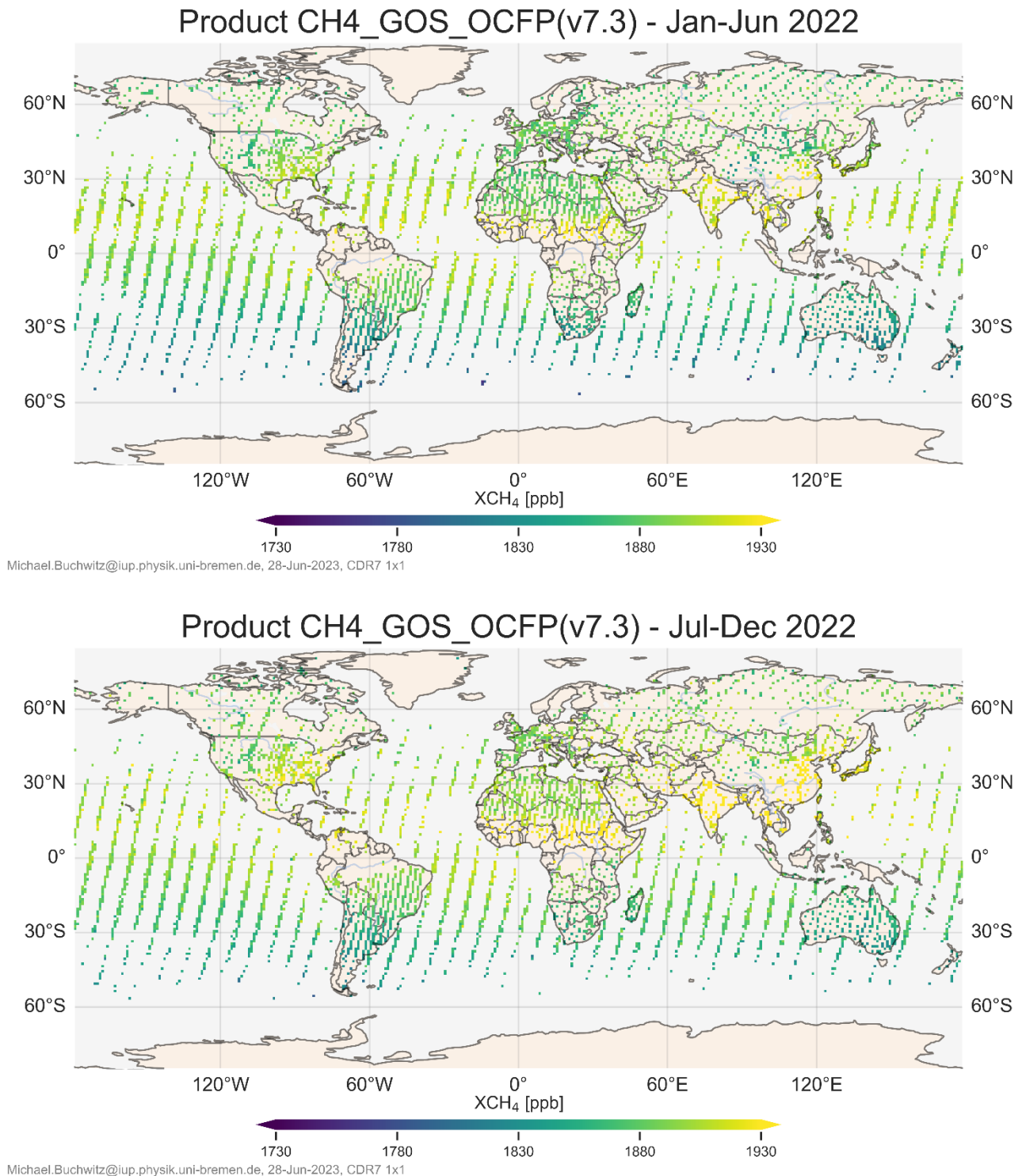
Figure 7 - XCH 4 product CH4_GOS_OCFP. Top: January to June 2022. Bottom: July – December 2022.
