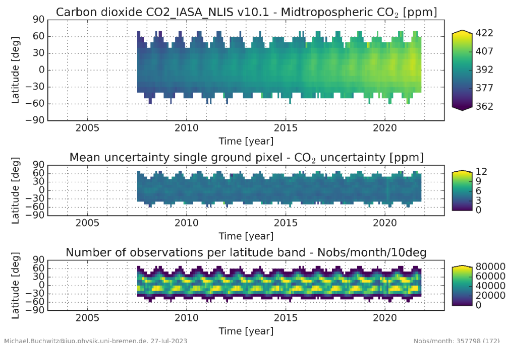
Figure 13 – Mid-tropospheric CO 2 (top) as seen by IASI/Metop-A, reported uncertainty (middle) and number of observations per month and 10 deg latitude band (bottom).
