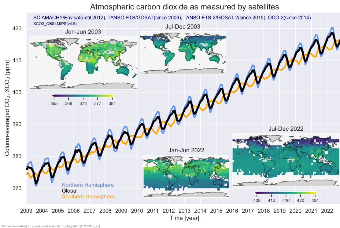
Figure 1 - C3S XCO 2 global maps and time series (product XCO 2 _OBS4MIPS version 4.5).
