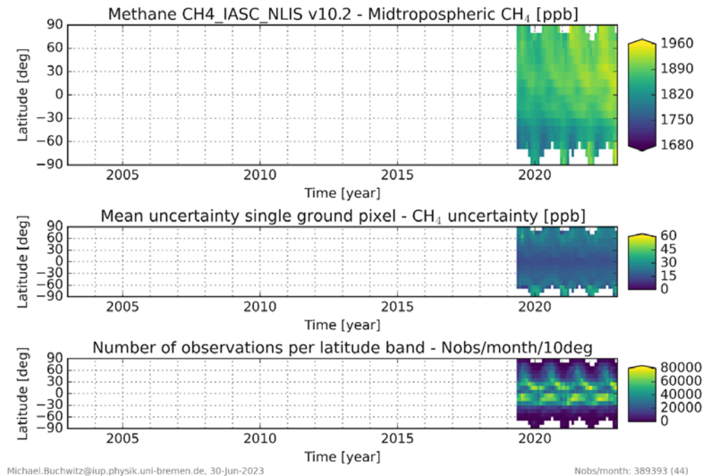
Figure 21 - Mid-tropospheric CH 4 (top) as seen by IASI/Metop-C, reported uncertainty (middle) and number of observations per month and 10 deg latitude band (bottom).
