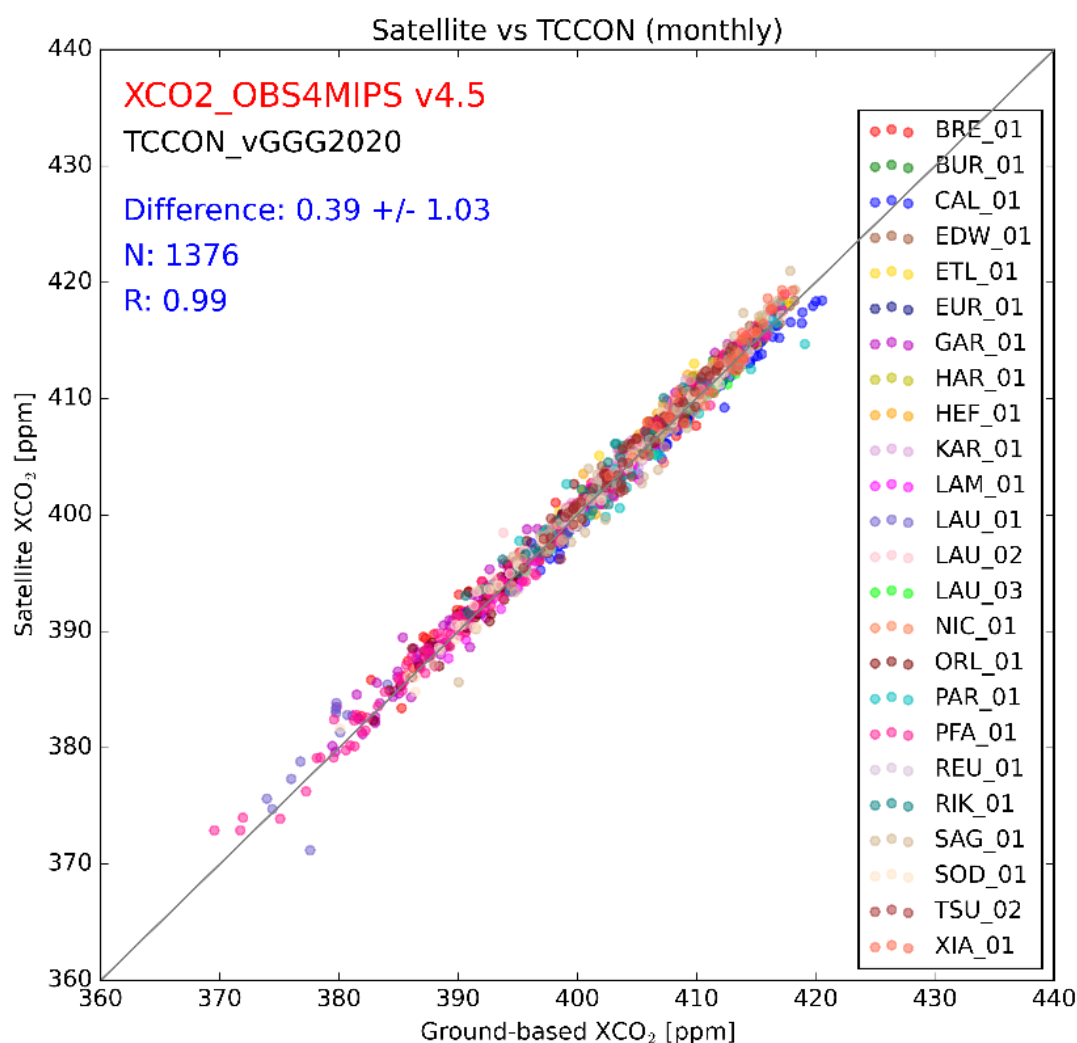
Figure 35 - Overview data quality assessment results for Level 3 XCO 2 Obs4MIPs format data product. Note that each dot corresponds to a given TCCON site and month.
