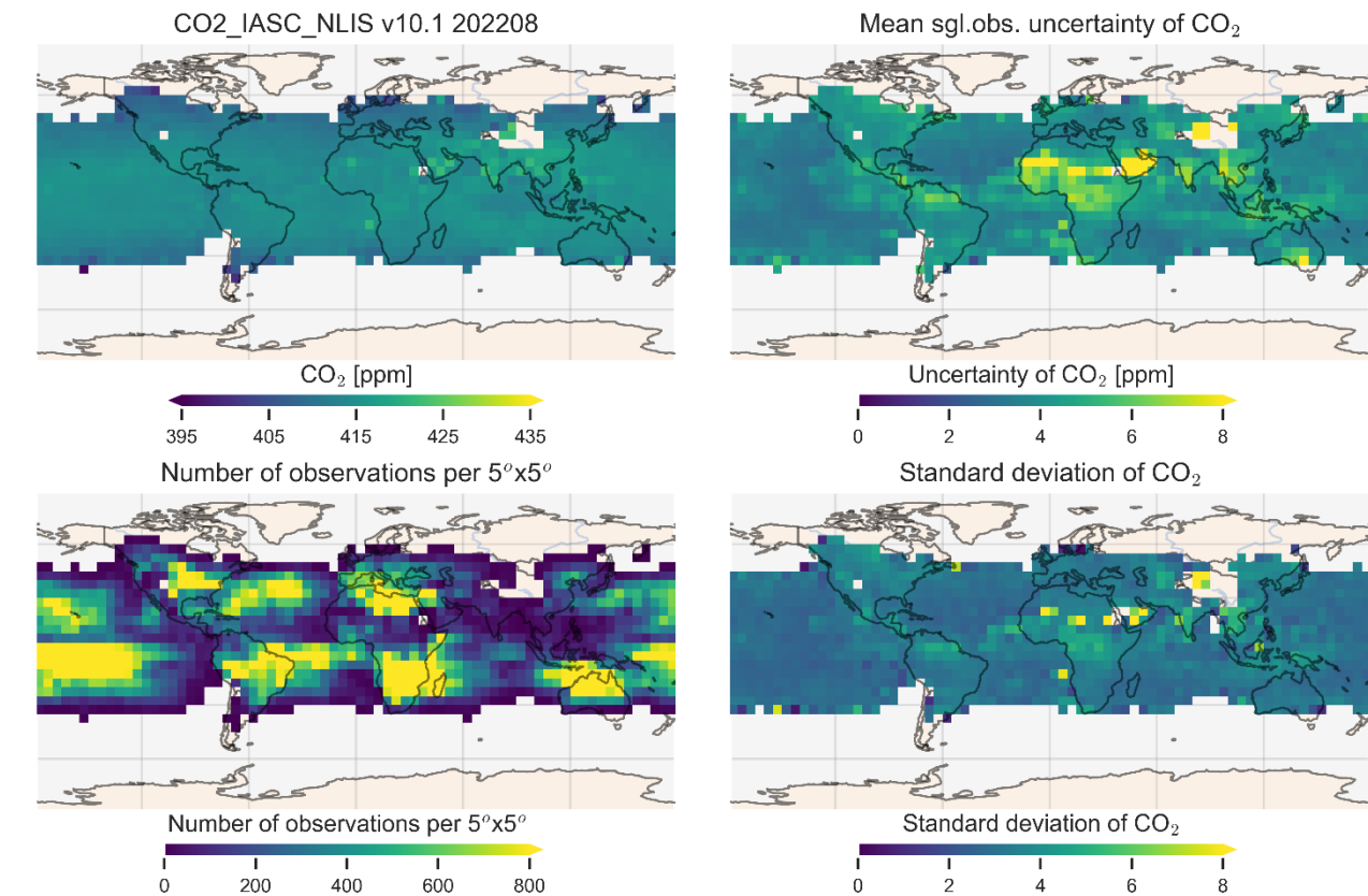
Figure 18 - Map of mid-tropospheric CO 2 from IASI/Metop-C for August 2022 (top left). Mean value of the reported uncertainty (top right), number of observations per 5°x5° grid size (bottom left) and standard deviation (bottom right).
