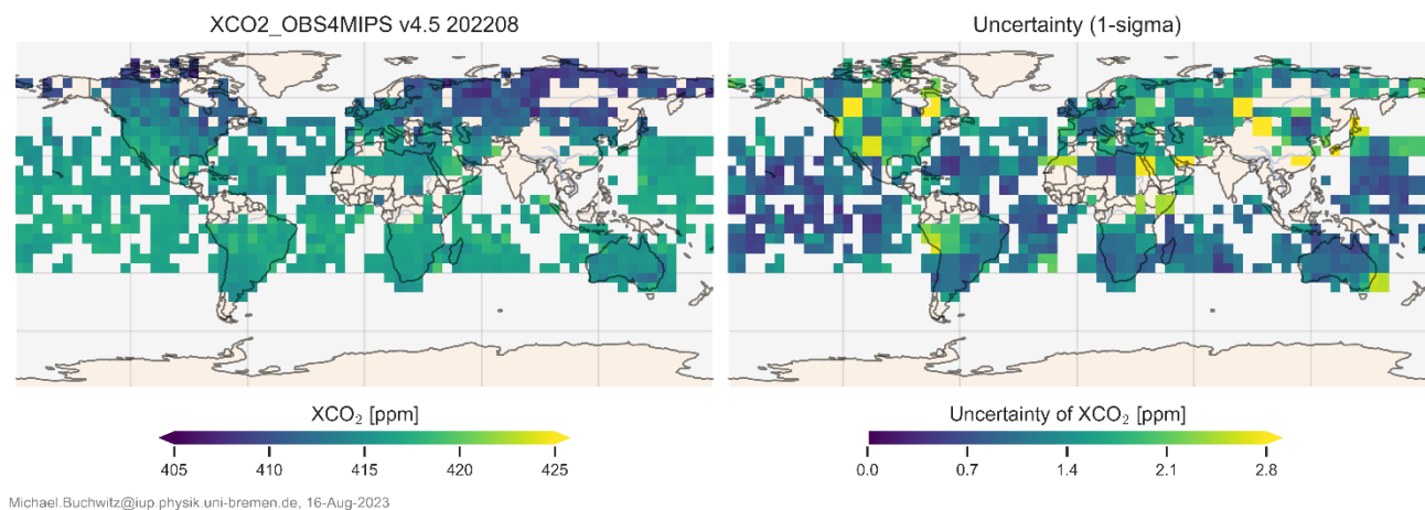
Figure 32 – OBS4MIPS XCO 2 (left) and corresponding uncertainty (right) for August 2022.
