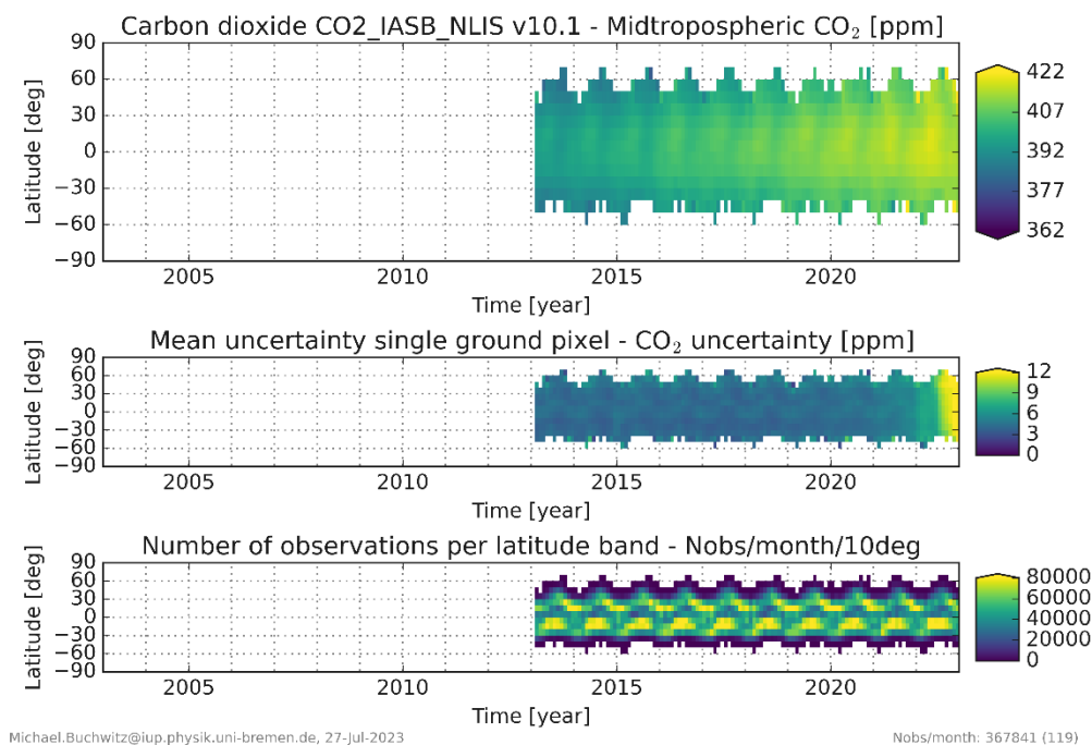
Figure 14 - Mid-tropospheric CO 2 (top) as seen by IASI/Metop-B, reported uncertainty (middle) and number of observations per month and 10 deg latitude band (bottom). The increasing uncertainty in 2022 indicates instrument degradation (see also Figure 17).
