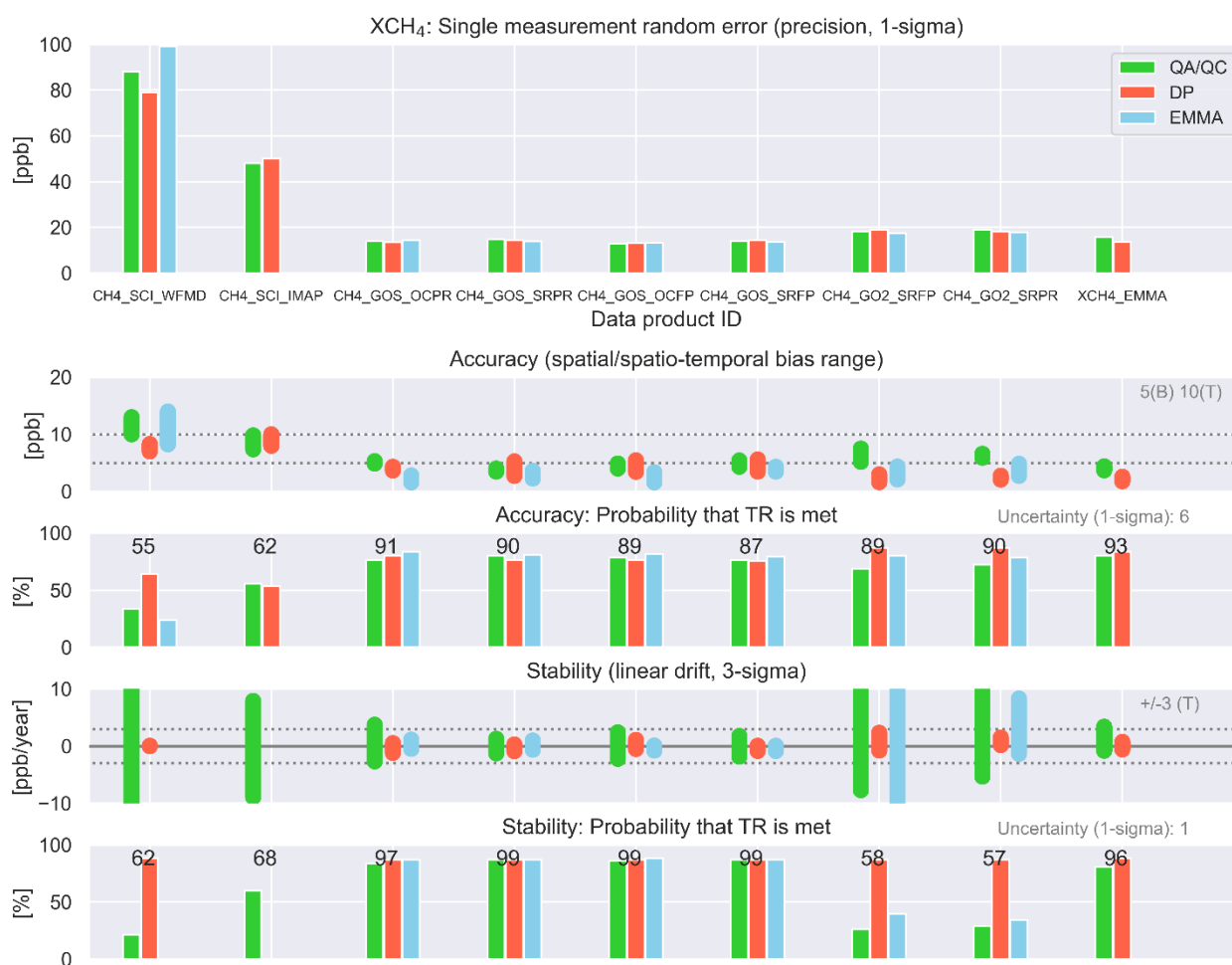
Figure 30 - Overview data quality assessment results for Level 2 XCH 4 data products (from D9). The green bars refer to the “Quality Assessment / Quality control” (QA/QC) results as described in detail in document D9. The red bars refer to results obtained by the data providers (DPs) (see D9). For “Accuracy” and “Stability” also the numerical values for the “Probability that TR is met” are given (computed as mean value if more than one value (bar) exists). Also listed (in grey on the right hand side) is the uncertainty of the reference data as used for the Target Requirement (TR) assessments. The listed values for products generated in previous C3S projects (products CH 4 _SCI_WFMD, CH 4 _SCI_IMAP, CH 4 _GOS_SRFP and CH 4 _GOS_SFPR) are listed here for completeness but have not been updated (for details see D9).
