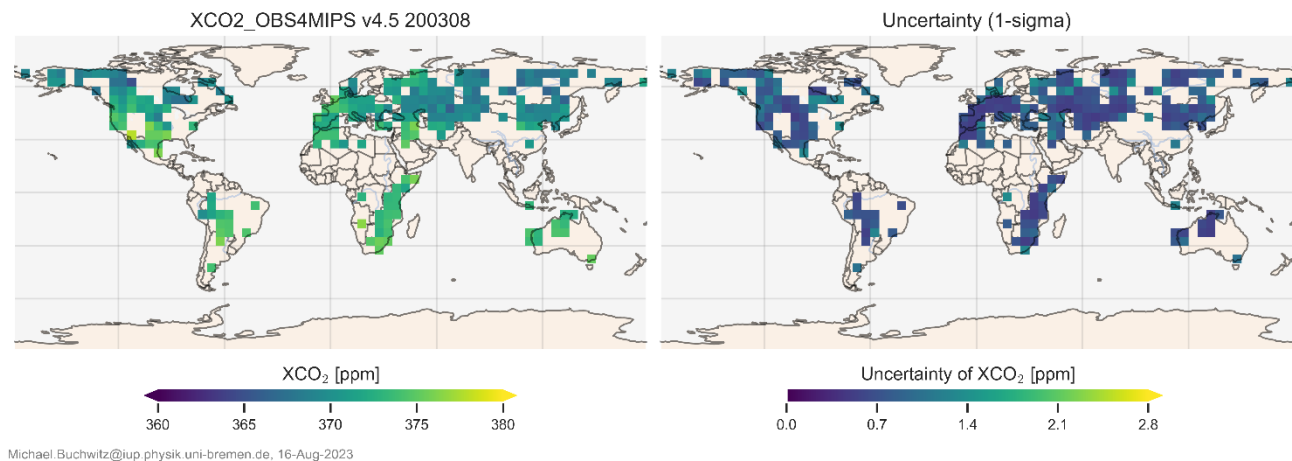
Figure 31 –OBS4MIPS XCO 2 (left) and corresponding uncertainty (right) for August 2003.
