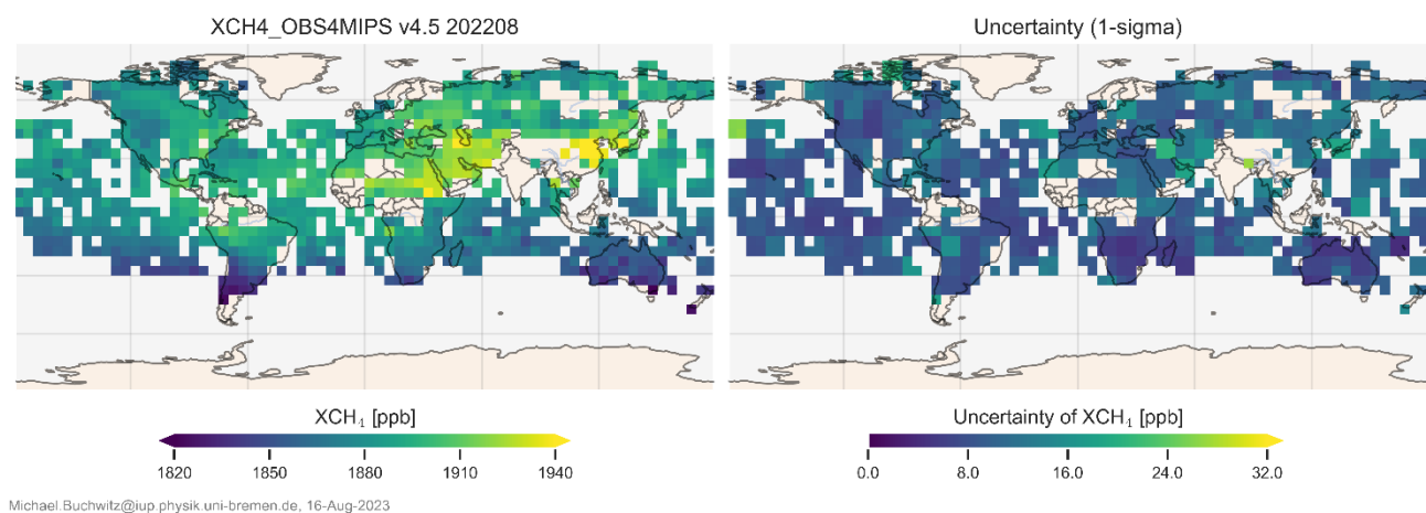
Figure 34 – OBS4MIPS XCH 4 (left) and corresponding uncertainty (right) for August 2022.
