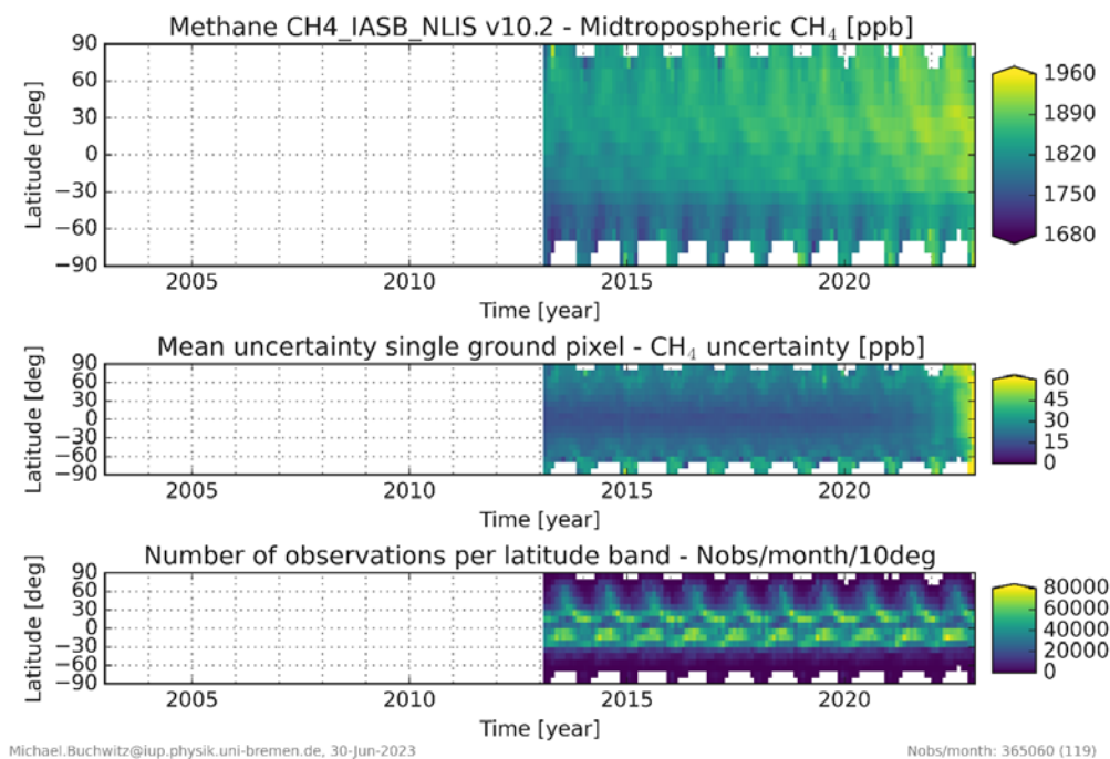
Figure 20 - Mid-tropospheric CH 4 (top) as seen by IASI/Metop-B, reported uncertainty (middle) and number of observations per month and 10 deg latitude band (bottom). The increasing uncertainty in 2022 indicates instrument degradation (as also identified for IASI-B CO 2 ).
