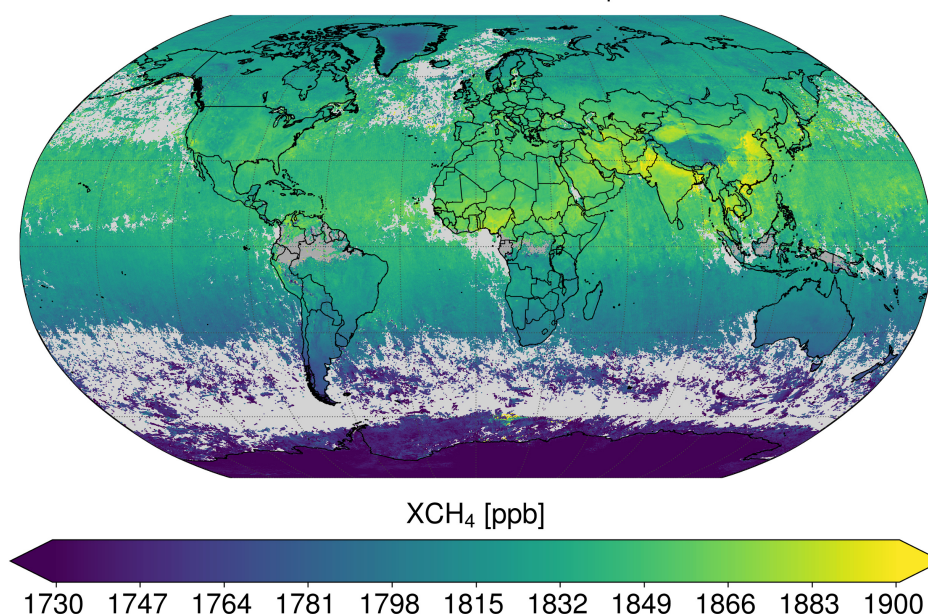
Figure 1: Annual mean (2018) of retrieved TROPOMI/WFMD v1.2 methane.
