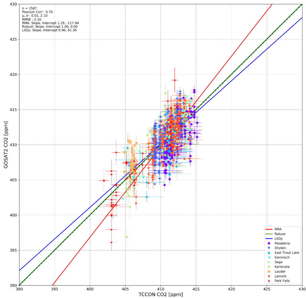
Figure 4.2 Validation of non-glint single soundings of FP-CO 2 with co-located TCCON measurements at all TCCON sites for the period Feb-Oct 2019. Numbers in the figures: \mu = bias, i.e., average of the difference; \sigma = single measurement precision, i.e., standard deviation of the difference; N = number of co-locations.
