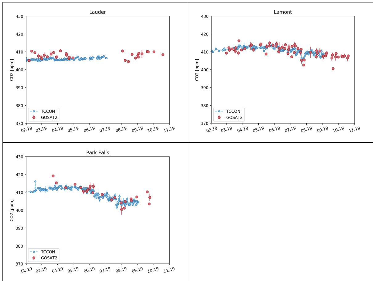
Figure 4.3 Comparison of non-glint single soundings of FP-CO 2 (red) with co-located TCCON (blue) measurements at all TCCON sites for the period Feb-Oct 2019.
