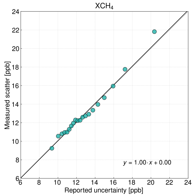
Figure 4.4: Comparison of the reported uncertainty of TROPOMI/WFMD v1.5 XCH 4 with the measured scatter relative to the TCCON after dividing up the reported uncertainties in equal sized bins.
