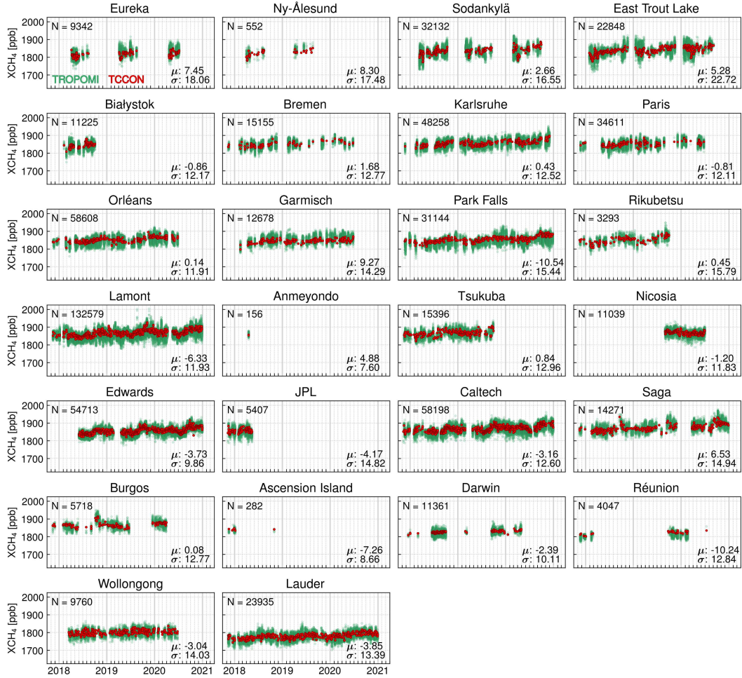
Figure 4.2: Comparison of the TROPOMI/WFMD v1.5 XCH 4 time series (green) with ground based measurements from the TCCON (red). For each site, N is the number of collocations, \mu corresponds to the mean bias and \sigma to the scatter of the satellite data relative to TCCON in ppb.
