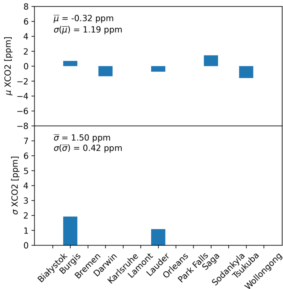
Figure 5: Same as Figure 4 but for sun-glint observations.
