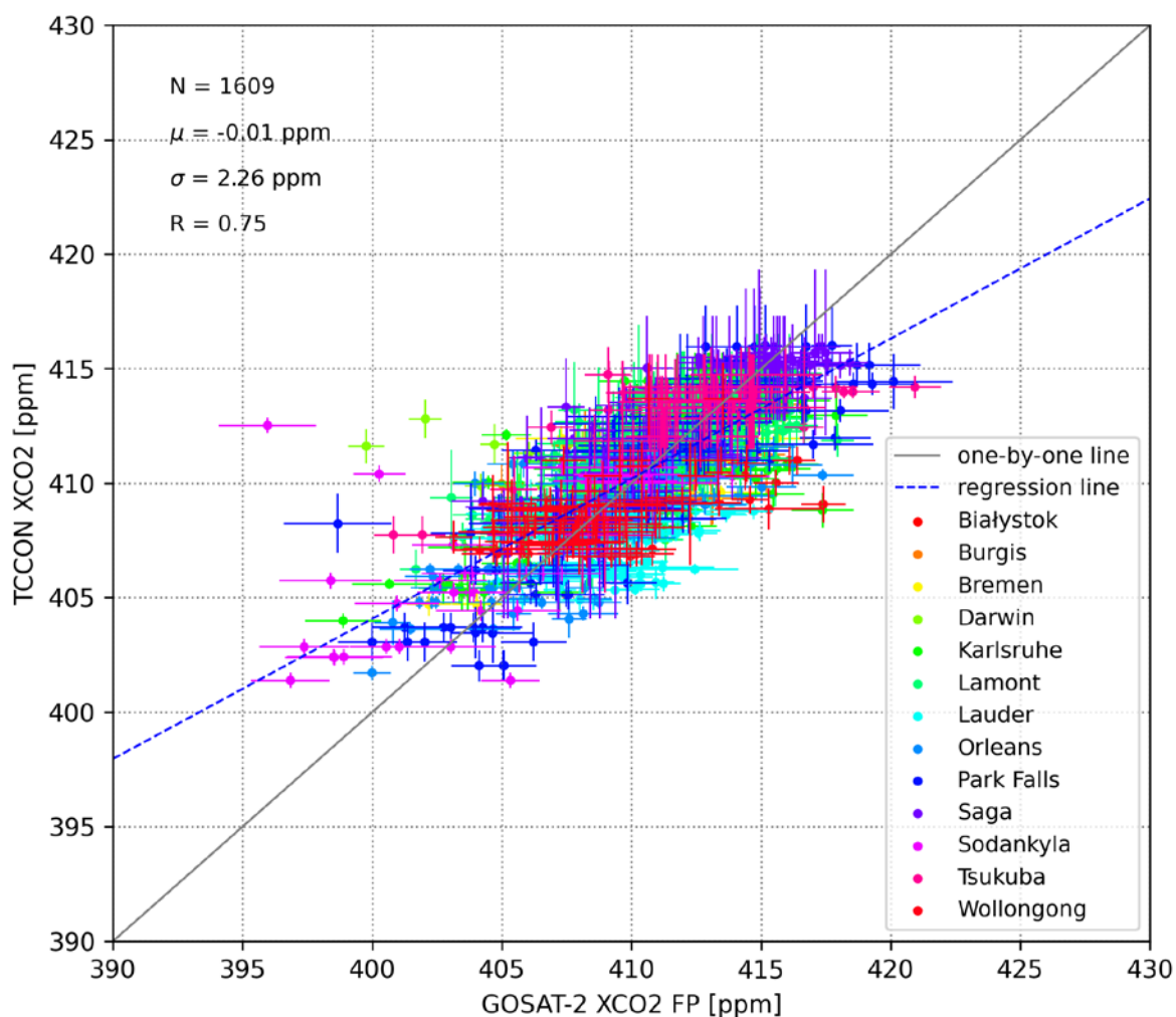
Figure 3: Validation of single soundings of FP-CO 2 with collocated TCCON measurements at all TCCON sites for the period Feb. 2019 - May 2020. Numbers in the figures: \mu = bias, i.e., average of the difference; \sigma = single measurement precision, i.e., standard deviation of the difference; N = number of co-locations; R = Pearson correlation coefficient.
