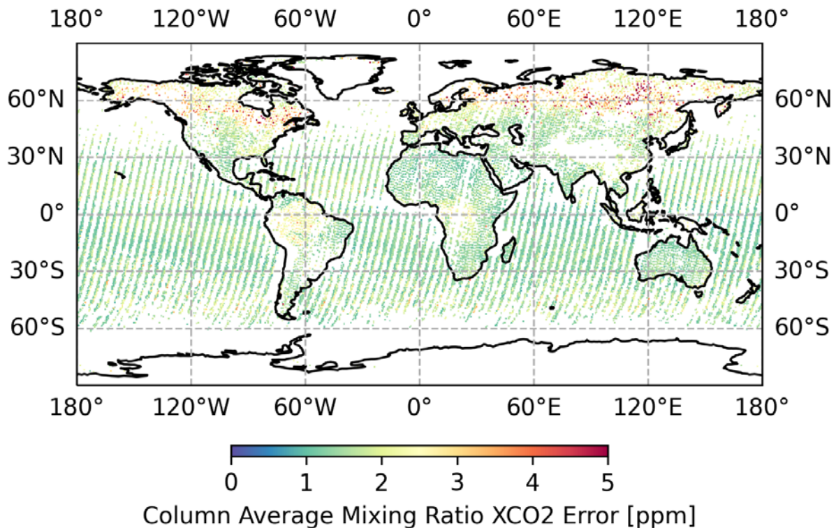
Figure 2: Same as Figure 1 but for the corresponding error.
