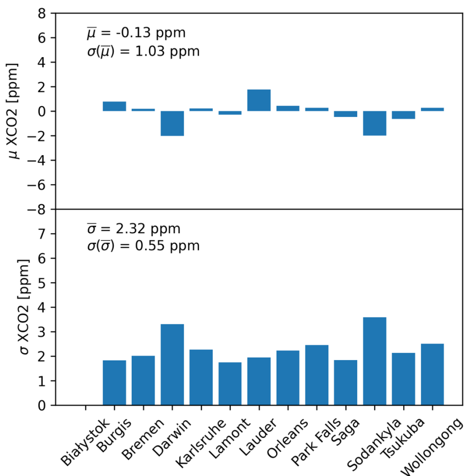
Figure 4: Validation statistics bias ( top ) and scatter ( bottom ) per TCCON site for land observation (bias corrected). The summarizing values represent the standard deviation of the site biases and the average scatter relative to TCCON.
