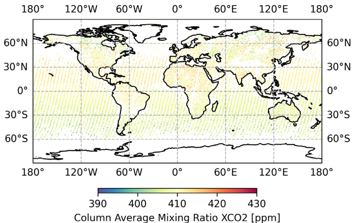
Figure 1: Global averaged XCO 2 between February 2019 and May 2020 for the CO 2 _GO2_SRFP product on a 0.5 by 0.5 degree resolution.
