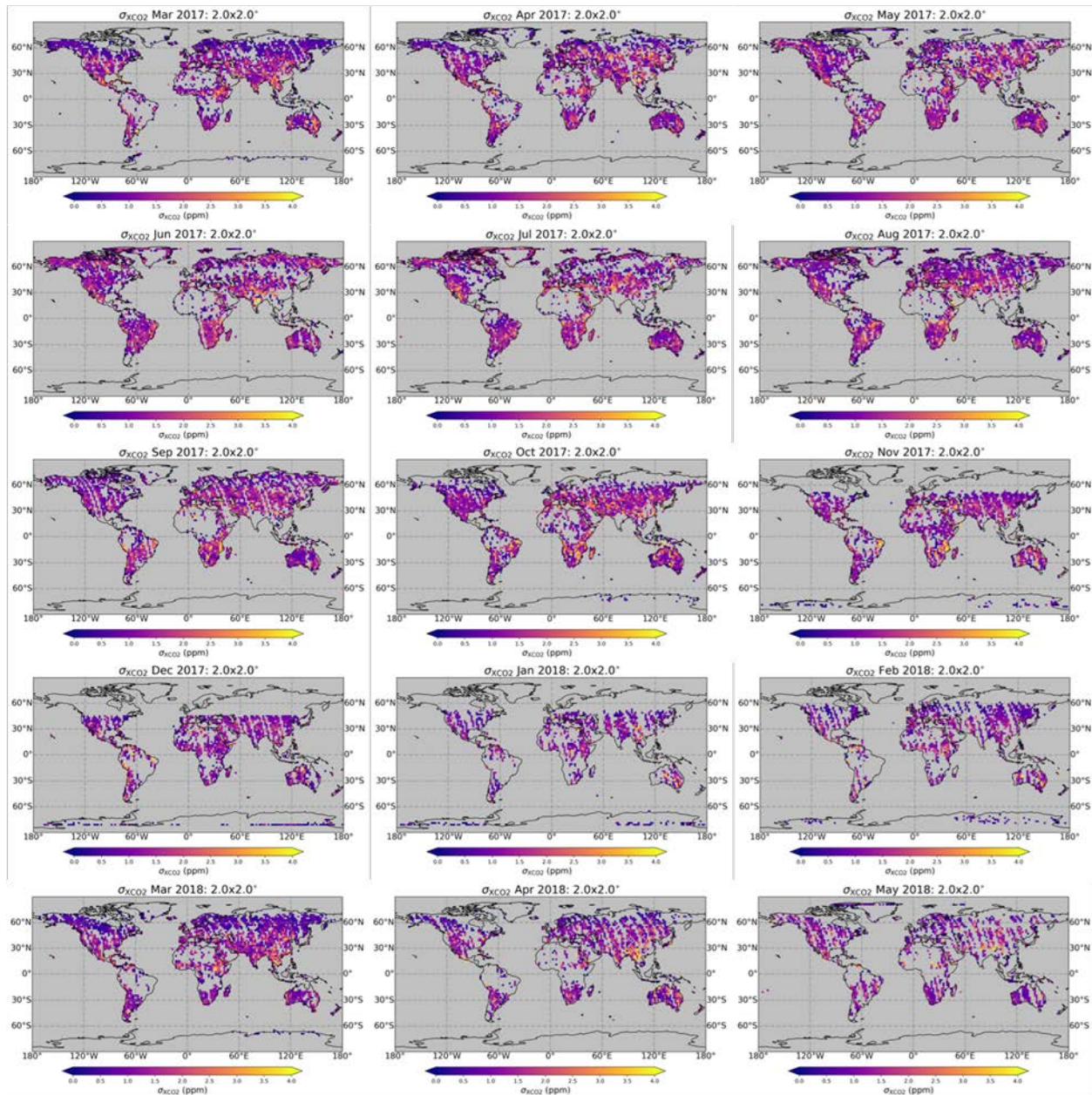
Figure 4: Standard deviation ( \sigma_{XCO_2} ) of XCO 2 concentrations as a function of longitude and latitude for March 2017 – May 2018 as observed by TanSat. The soundings have been bias-corrected and filtered as per Table 1.
