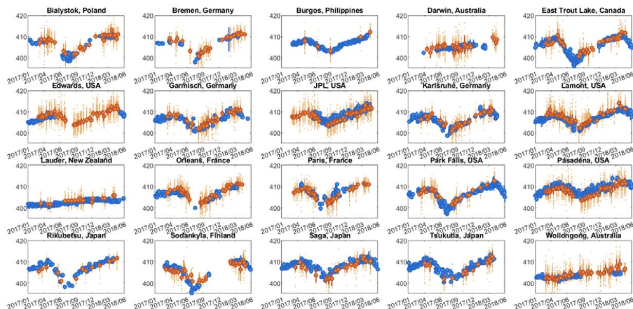
Figure 1: Comparison of the CO 2 _TAN_OCFP v1 (CRDP#5, orange) with the TCCON XCO 2 (blue, overpass mean) between March 2017 and May 2018. The overpass-mean from TanSat is indicated with large orange solid circles with error bars indicating the standard deviation, and small orange points show individual soundings. We plot all measurements that satisfy the co-location criteria of an overpass.
