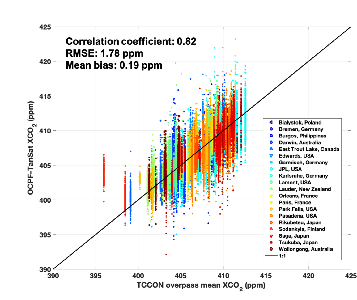
Figure 2: Comparison of individual retrieved XCO 2 from TanSat with the overpass mean of TCCON XCO 2 for the time period of March 2017 to May 2018 across all 20 TCCON sites. Each TCCON site is given by different colour and symbol. Statistics for mean bias and RMSE (calculated by averaging the bias and RMSE of each site) are given along with the correlation coefficient.
