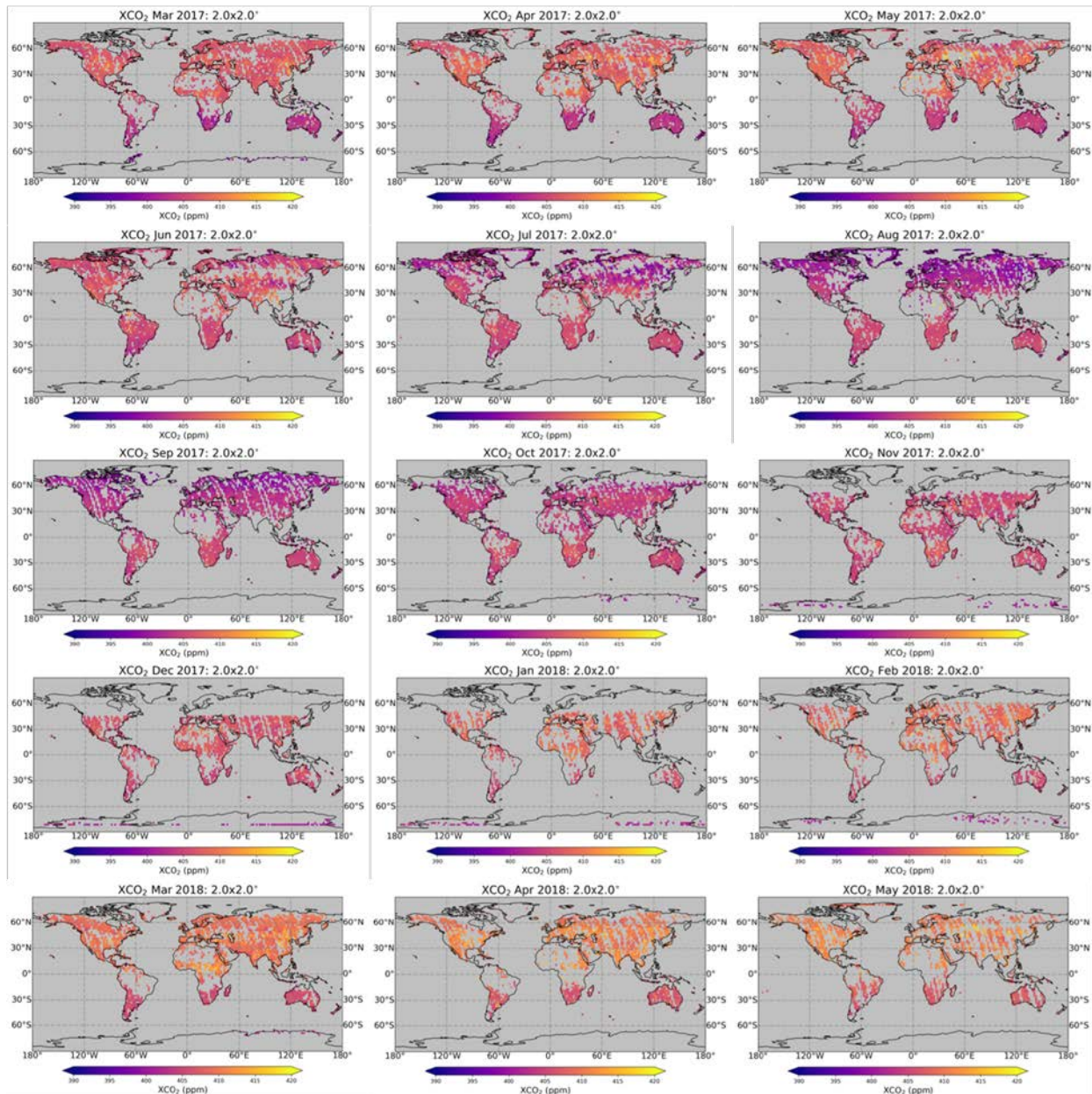
Figure 3: Global monthly median XCO 2 concentrations as a function of longitude and latitude for March 2017 – May 2018 as observed by TanSat. The soundings have been bias-corrected and filtered as per Table 1.
