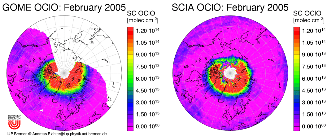
Fig. 1: Comparison of GOME (left) and SCIAMACHY OCIO slant columns for February 2005. As result of the permanent failure of the tape recorder on ERS-2, only partial coverage is available from GOME. Similarly, SCIAMACHY measurements have less coverage owing to the alternating limb nadir measurements. Note that the solar zenith angle at overpass is different for the two instruments, resulting in different OCIO photochemistry.
