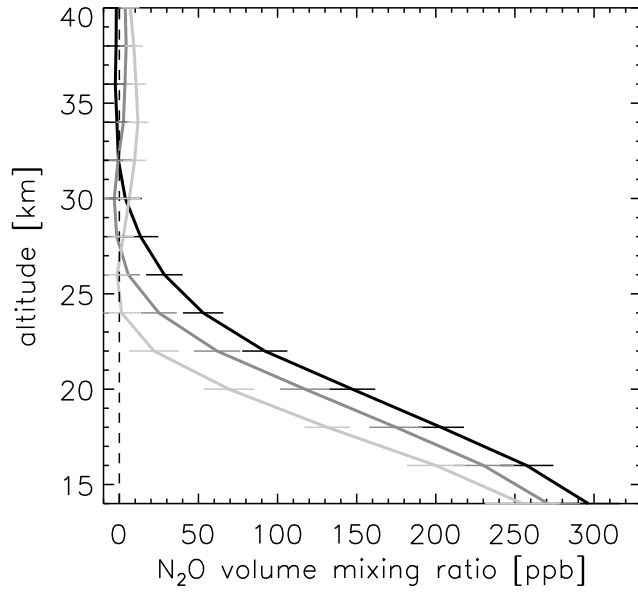
Figure 3. Evolution of ASUR N 2 O measurements during winter 1999/2000. The profiles are an average of all measurements with an equivalent latitude between 70 and 90 degrees for each deployment. Black: December 1999, grey: January 2000, light grey: March 2000. Error bars indicate standard deviation about the mean.
