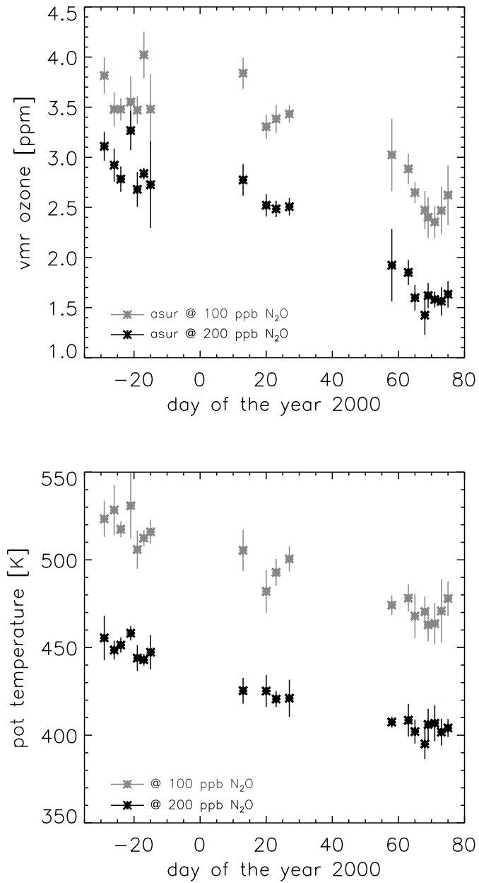
Figure 6. Daily mean ASUR ozone volume mixing ratios [ppm] (top) and potential temperature derived from DAO analysis (bottom) at two different N 2 O levels within the polar vortex: black stars: 200 ppb N 2 O, grey stars: 100 ppb N 2 O. Error bars are the sum of standard deviation of the individual measurements and uncertainties for the given N 2 O level.
