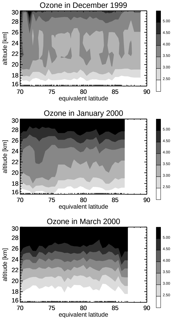
Figure 4. Evolution of ozone volume mixing ratio [ppm] of all ASUR measurements within the polar vortex. Individual measurements are binned every 0.5 degrees. Crosses in the bottom indicate individual measurements.
