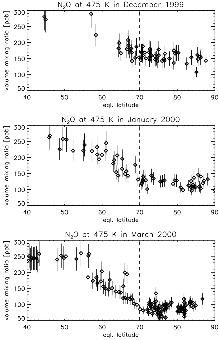
Figure 2. All ASUR \text{N}_2\text{O} measurements during winter 1999/2000 as a function of equivalent latitude. \text{N}_2\text{O} volume mixing ratios in [ppb] at 475 K of potential temperature are plotted. Top: December 1999, middle: January 2000, and bottom: March 2000. Error bars indicate precision of the single measurement.
