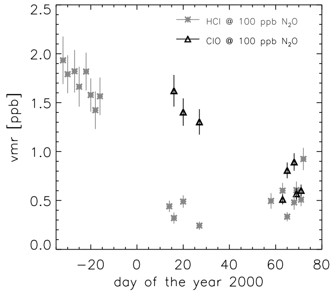
Figure 7. ASUR daily mean of HCl (grey stars) and ClO (black triangles) within the polar vortex at 100 ppb N_2O . Only ClO measurements with Solar Zenith Angles smaller than 86 degrees are shown. Error bars are the sum of standard deviation of the individual measurements and uncertainties for the given N_2O level. In December 1999 no ClO measurements were taken with an equivalent latitude greater 70 degrees and a Solar Zenith Angle smaller than 86 degrees.
