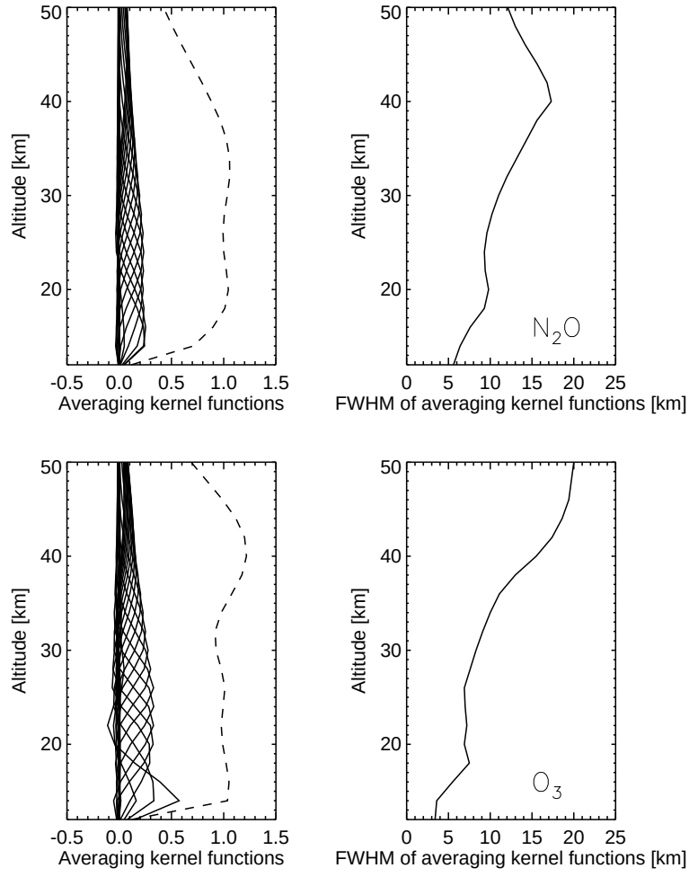
Figure 1. Averaging kernel functions (left) and the full width of half maximum of the averaging kernel functions (right) for a typical \text{N}_2\text{O} (top panel) and ozone (bottom panel) measurement. The dashed line is the sum of the averaging kernels.
