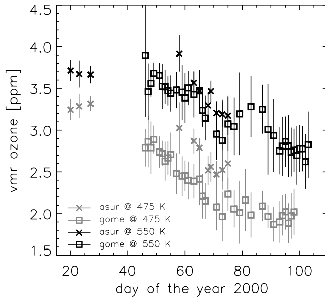
Figure 5. Comparison between ASUR and GOME ozone measurements at 475 K (ASUR grey crosses, GOME grey squares) and 550 K (ASUR black crosses, GOME black squares) isentropic level inside the vortex. Error bars are the sum of standard deviation of the single measurements and uncertainties for the given potential temperature level.
