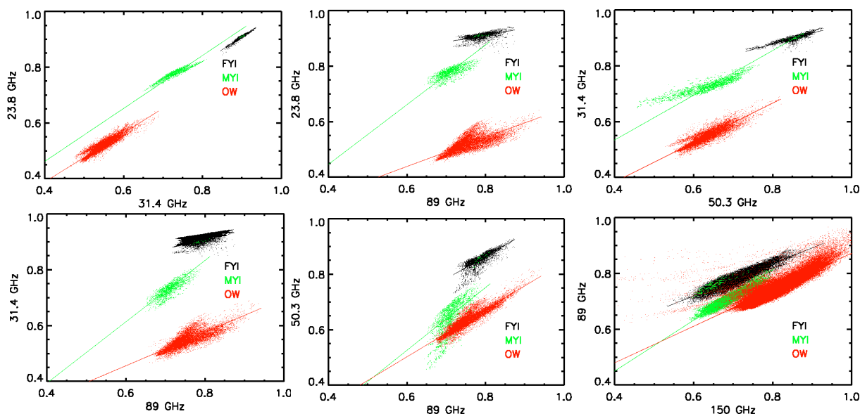
Figure 6.8: Scatter plot of emissivities at several frequency pairs, for three different surface types: First-year ice (black), multiyear ice (green), and open water (red). Average of March 2005.
