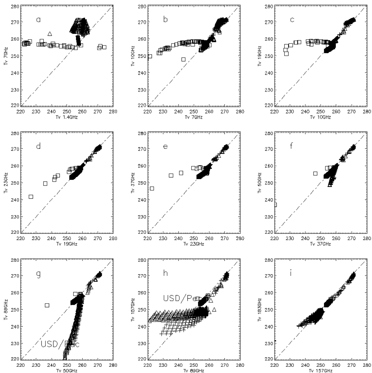
Figure 6.21: The simulated correlation between nilas ( \square ), first-year ice ( + ), and multiyear ice ( \triangle ) T_v for the 10 frequencies using all parameter pairs in Table 6.10 (every 3rd data point). The off-diagonal points marked by USD/p_{ec} in plot g and h are associated with the upper snow density ( USD )/ bottom snow layer correlation length ( p_{ec} ) parameter pair. The nilas T_v extends beyond the range of plots a–e.
