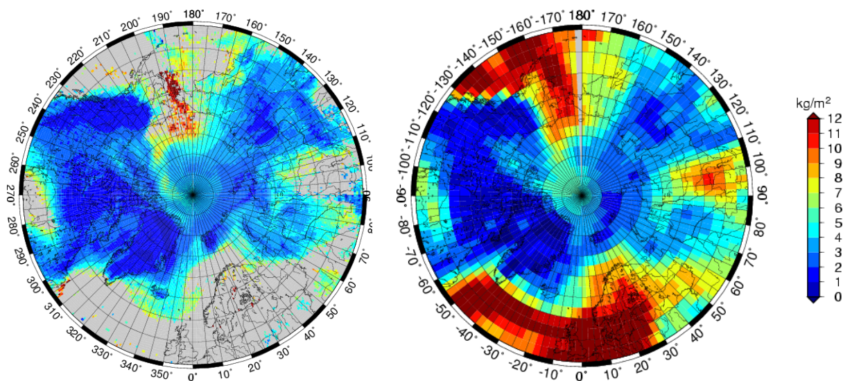
Figure 6.2: Maps of TWV over the Arctic. Comparison of (left:) TWV retrieved from AMSU-B data with the extended algorithm and (right:) TWV from reanalysis data of NCEP (National Centers for Environmental Prediction). 18 March, 2002. Note the intrusion of moist air ( TWV > 10 \text{ kg/m}^2 ) through the Bering Strait (between center and upper edge of the maps).
