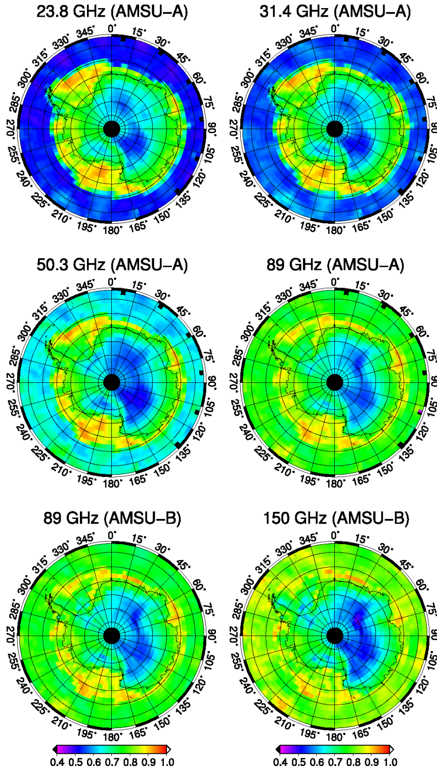
Figure 6.9: Maps of the emissivity of Antarctic for all AMSU window frequencies, 25 Apr 2002
