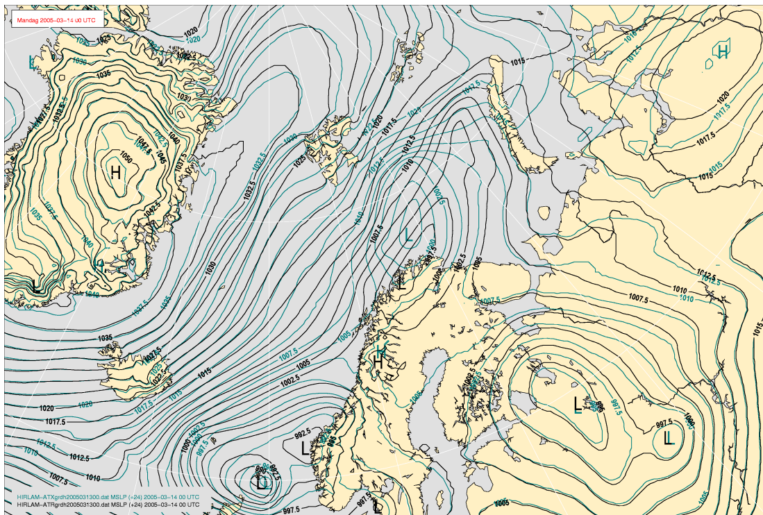
Figure 6.14: Weather situation on 14 March, 2005, 00UTC, 24 hrs forecast. Black: reference, green: experiment using AMSU-A over sea ice.
