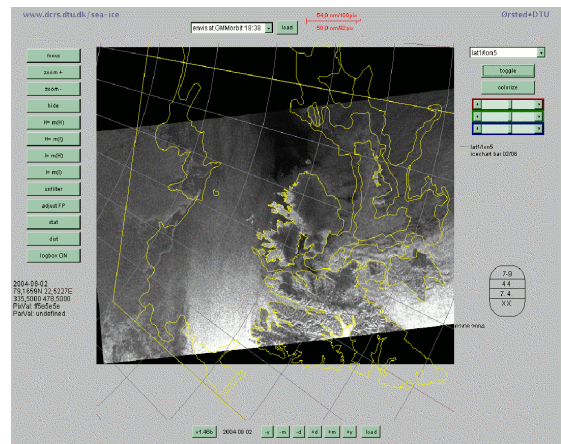
Figure 6.27: Example of clickable NIC ice chart overlaid an ENVISAT ASAR Global Monitoring mode image of the Svalbard area.
