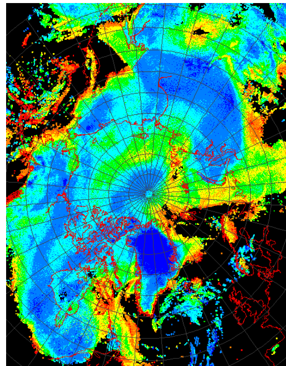
Figure 6.31: Retrieval of total atmospheric water vapour from AMSU-B data using University of Bremen algorithm from from WP1. AMSU-B data from Cooperative Institute for Research in the Atmosphere, Colorado State University, December 5, 2004.
