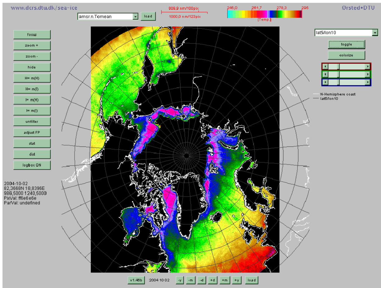
Figure 6.33: The daily SST composites are now being combined into a 7-day mean SST image for the northern hemisphere.
