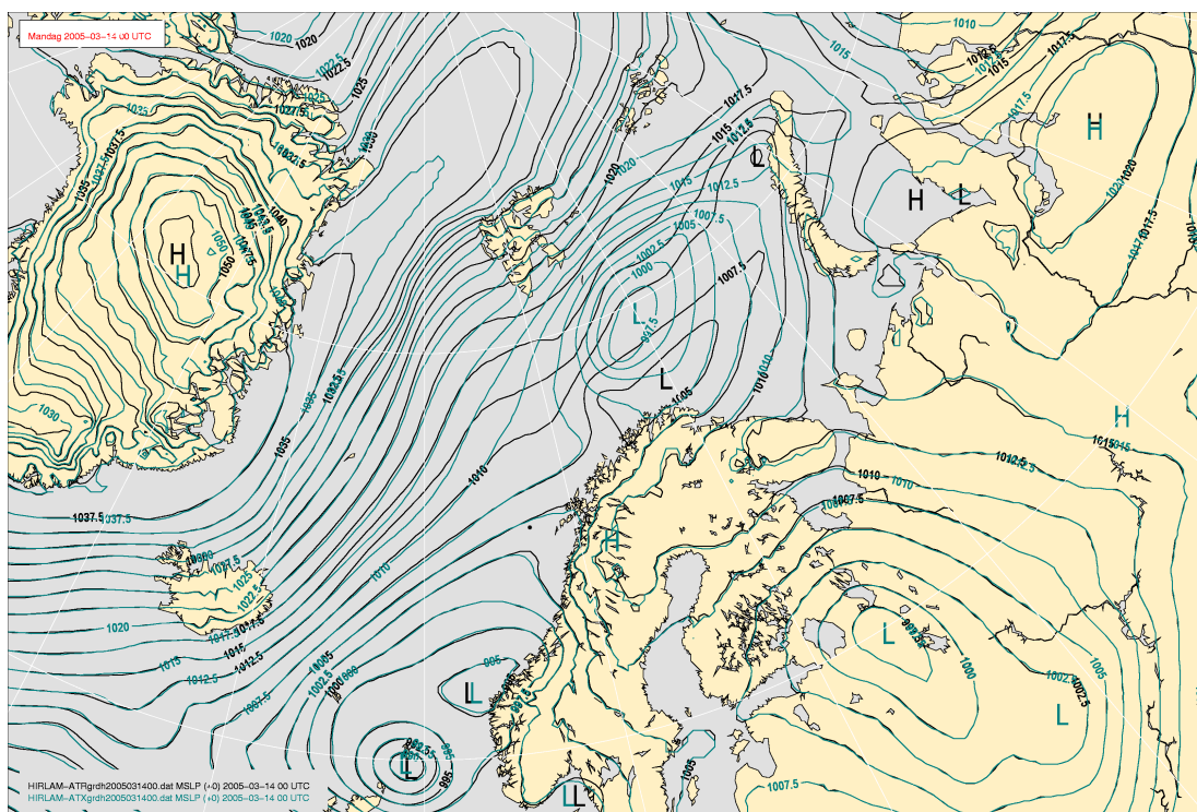
Figure 6.15: Weather situation 14 March 2005 00UTC, analysis. Black: reference, green: experiment using AMSU-A over sea ice.
