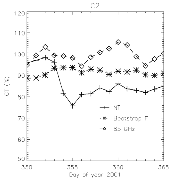
Figure 6.22: The satellite-observed average ice concentration in a small area in Baffin Bay ( 62.6^{\circ}\text{W} , 71.5^{\circ}\text{N} ) using NASA Team (+), Bootstrap in frequency mode (*) and Near 90GHz ( \diamond ) algorithms, December 2001. The variability is a function of ice concentration and both surface and atmospheric emissivity. The measured air temperature on a nearby meteorological station on the Greenland coast (Upernavik) increased above 0^{\circ}\text{C} on day of year 353/354 and the freeze-up began on day 357 [from Tonboe et al., 2003].
