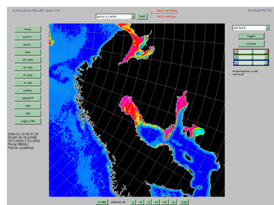
Figure 6.29: Example of a high resolution ice product for the Baltic Area.
