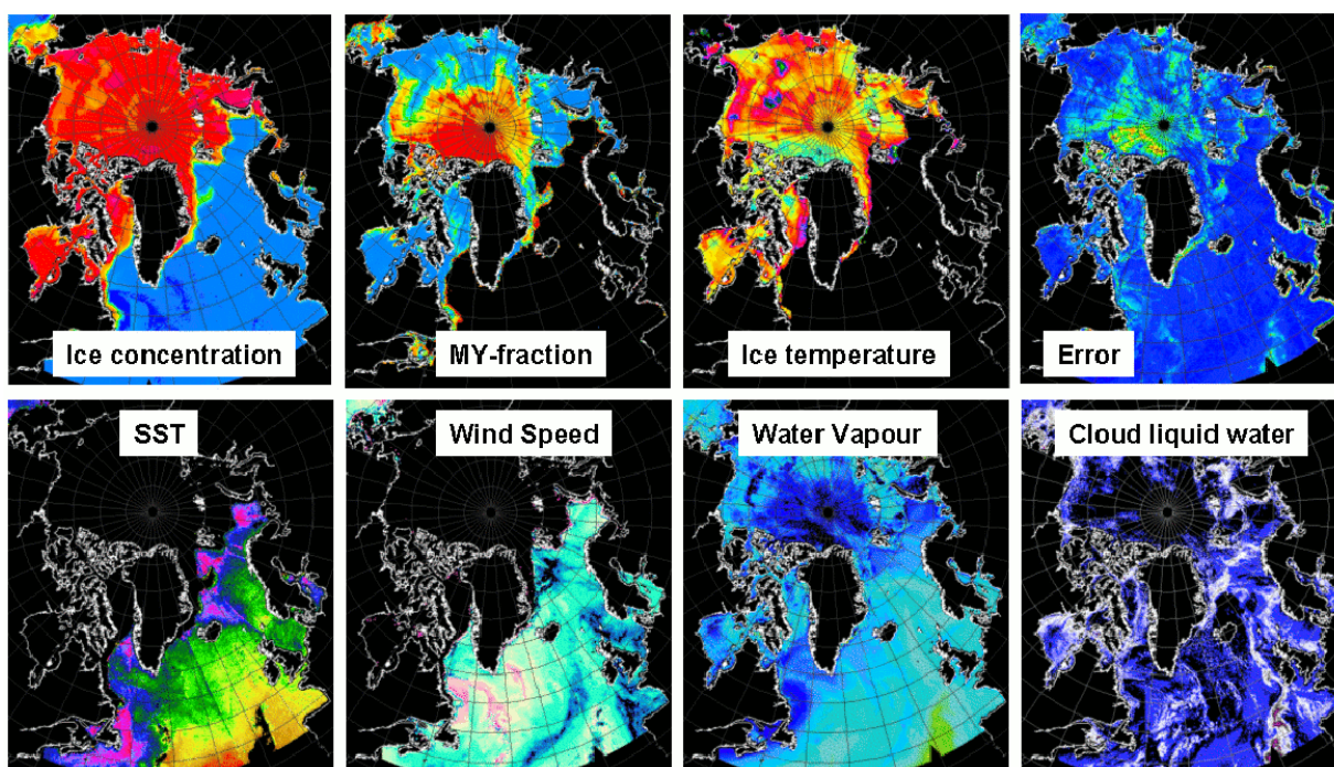
Figure 6.32: All parameters retrieved using the optimal parameter estimation technique. Input AMSR-E swath data from NSIDC, output the 7 parameters presented above. The plot titled Error shows the mismatch between the modelled and the measured antenna temperatures. Blue indicates very small errors, red large errors.
