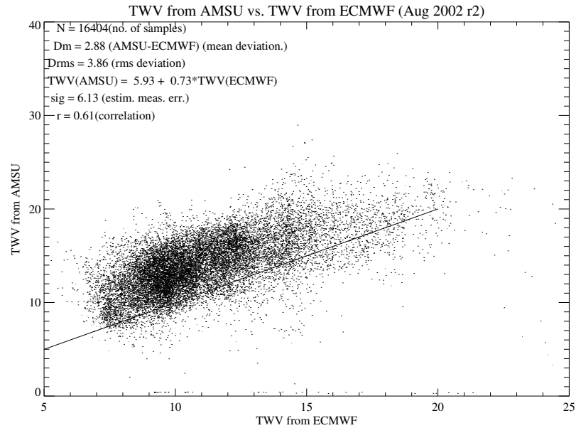
Figure 6.5: AMSU-B-derived TWV versus ECMWF (ERA-40) TWV. August 2002, North of Greenland ( 83-90^\circ N, 0-90^\circ W); solid line = identity.
