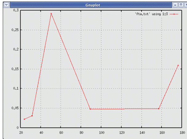
Figure 6.17: Atmospheric absorption coefficient at AMSU frequencies assuming a minimal water vapour load.
