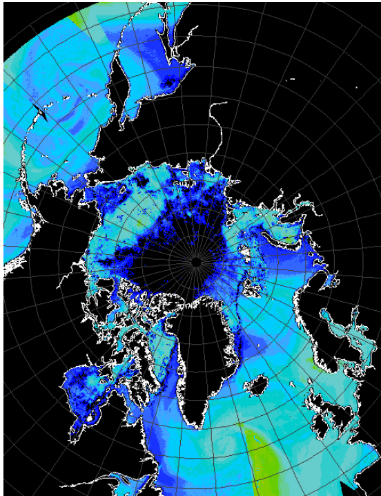
Figure 6.30: Retrieval of integrated water vapour using forward model from WP3. AMSR-E data from National Snow and Ice Data Center, December 5, 2004.
