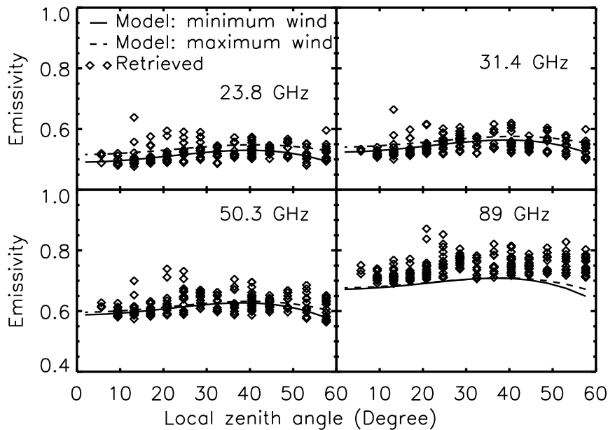
Figure 3.1: Emissivity of open water from AMSU-A/Polarstern profiles (symbols) and from FASTEM (lines); Arctic, all AMSU-A window channels; wind: 6.3 m/s, 16.8 m/s
