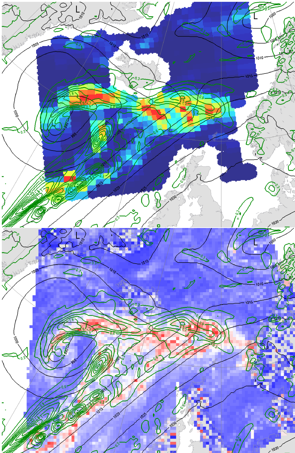
Figure 6.10: Weather situation on 3 October 2005, 18UTC. Upper panel: AMSU-A TCLW imagery with overlaid HIRLAM pressure analysis analysis and a short-range TCLW forecast. Lower panel: As above, but with R-factor imagery instead of AMSU-A TCLW imagery.
