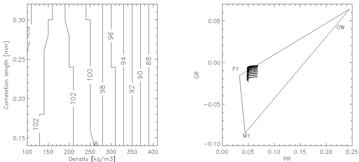
Figure 6.23: Simulated sensitivity at ground level of the NASA Team algorithm ice concentration [%] to variations in the upper snow layer density (layering) and bottom snow layer correlation length (grain size) in the snow cover on 100% first-year ice (left). Simulated data placed in the PR19 and GR19v/37v space with the approximate NASA Team retrieval triangle in the background (right). Tie-points for open water (OW), first-year ice (FY) and multiyear ice (MY) based on Andersen [1999] [from Tonboe and Andersen, 2004].
