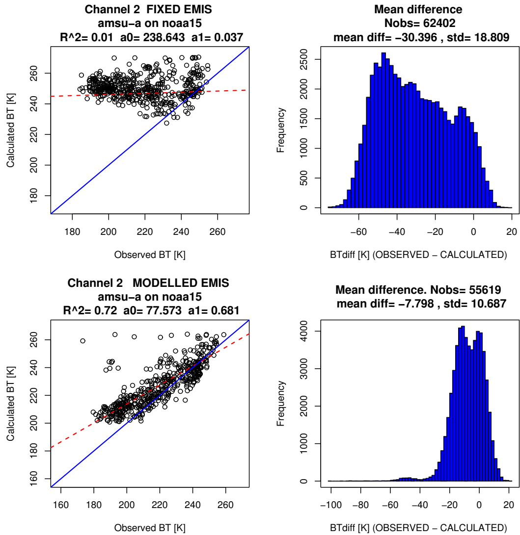
Figure 6.12: Scatterplot of observed versus modelled brightness temperatures and histogram for departures for AMSU channel 2: Top: with constant sea ice emissivity; bottom: with ice-type dependent emissivity estimated as described in the text.
