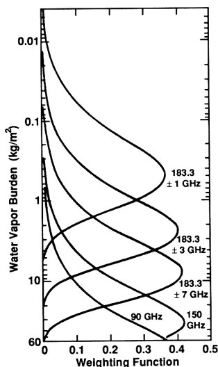
Figure 6.3: Weighting functions of AMSU-B channels as a function of total water vapour (“water vapour burden”) over land, from Janssen [1993]
