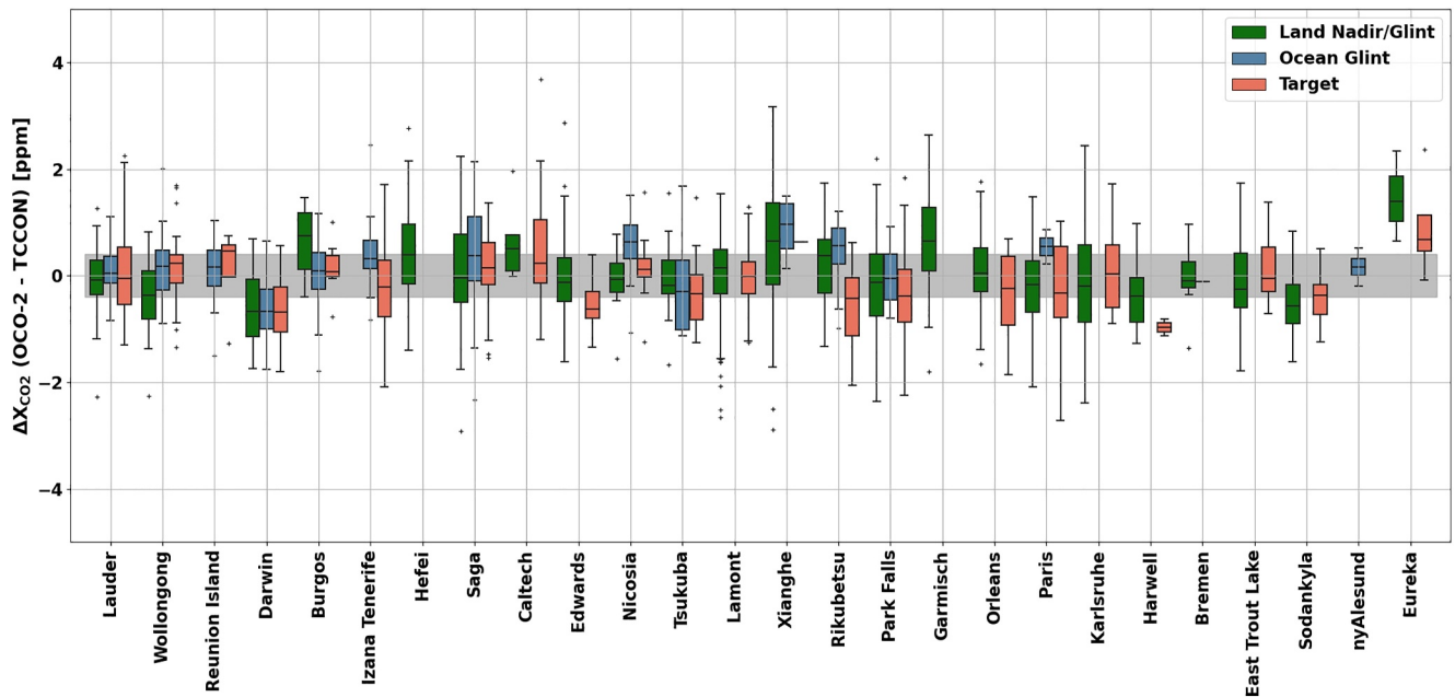
Figure 8. The observation mode-separated site-to-site \Delta X_{CO_2} values in ppm (OCO-2 minus corresponding coincident TCCON X_{CO_2} measurements). The bottom and top edges of the boxes indicate the 25 and 75 percentile limits, respectively. The whiskers show the full range of the data excluding outliers, and the outliers are shown by plus (“+”) symbols. The gray shaded area represents the \pm 0.4 ppm uncertainty margin. Deviations beyond this shaded region are attributed more strongly to the uncertainties in the OCO-2 data.
