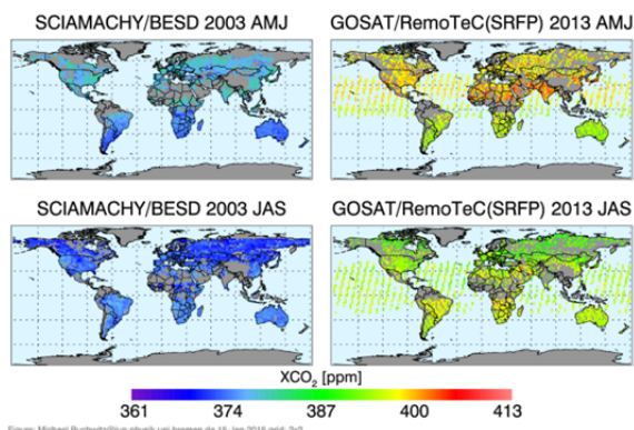
Fig.2: GHG-CCI CRDP#2 XCO 2 products.
