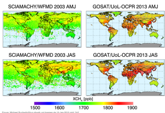
Fig.3: GHG-CCI CRDP#2 XCH 4 products.
