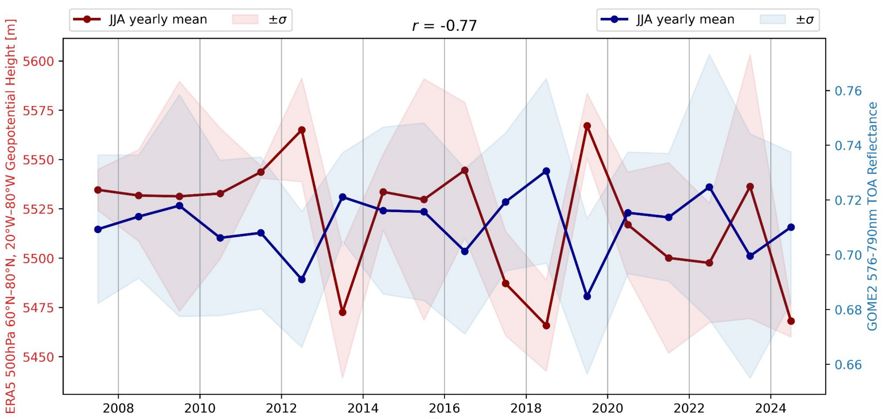
Fig. 3: GOME2 576-790nm reflectance over Greenland and ERA5 500 hPa 60°N-80°N, 20°W-80°W geopotential height, i.e. the Greenland Blocking Index (GBI), JJA averages (where 500 hPa geopotential height corresponds to the height of the 500 hPa pressure level adjusted to account for variation in gravity, altitude and latitude)
