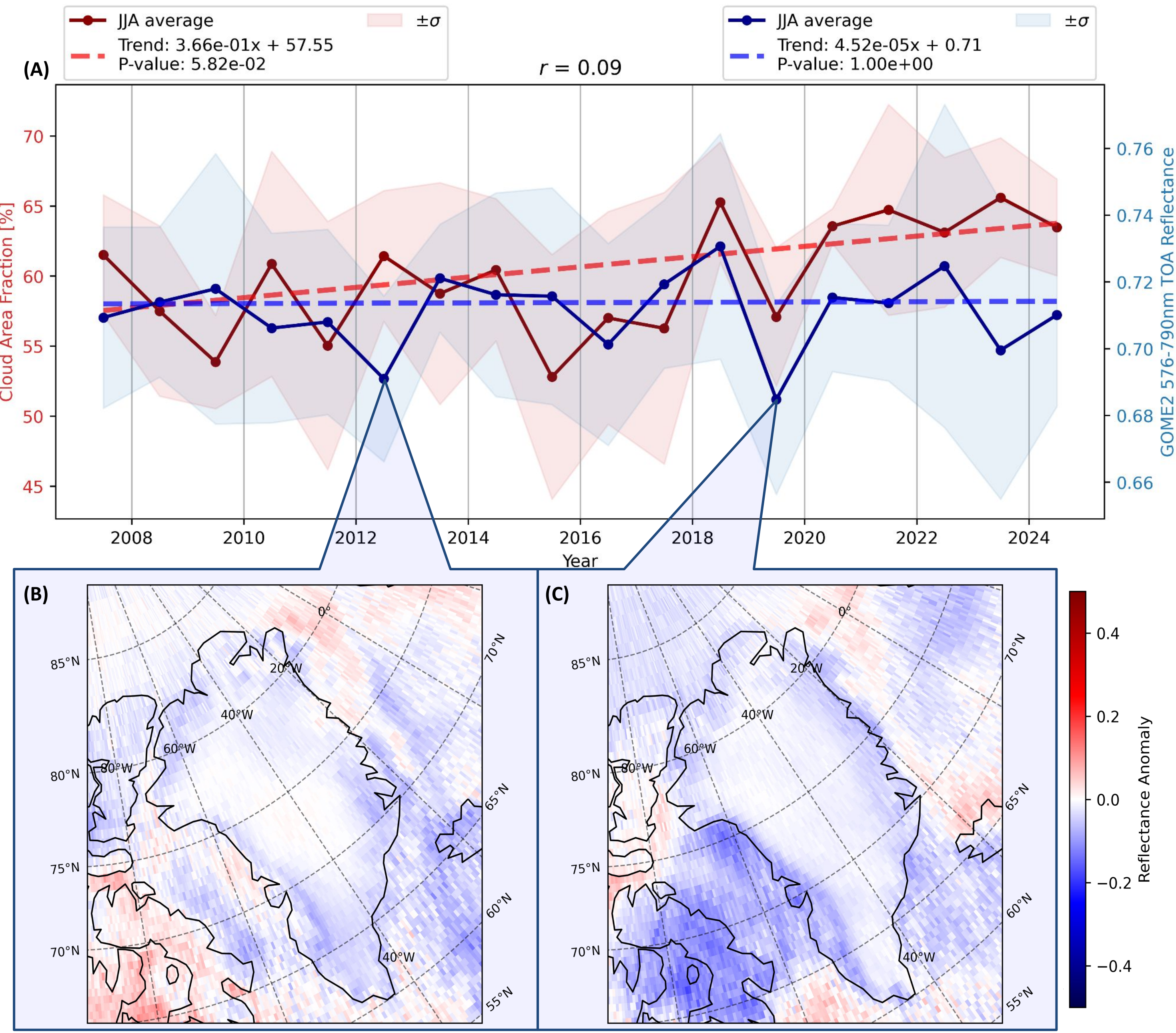
Fig. 2: (A) GOME2 576-790nm Reflectance and CERES cloud area fraction (CAF) JJA averages over Greenland, (B) 2012 JJA Reflectance anomaly, (C) 2019 JJA Reflectance anomaly (where an anomaly is defined as a given summer average subtracted from the average of all summers in the 2007-2024 period)
