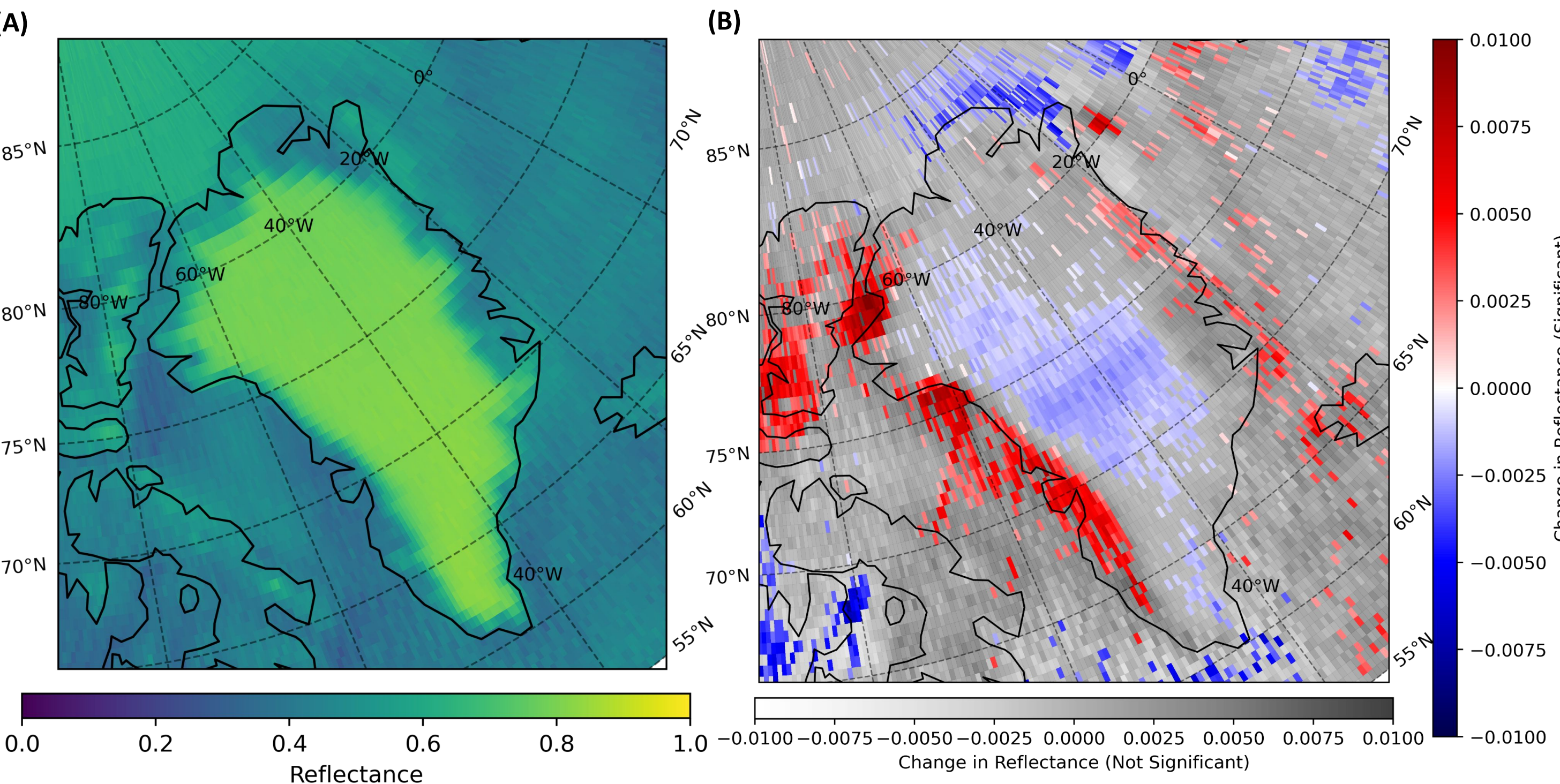
Fig. 1: (A) 2024 Summer GOME2 576-790nm Reflectance (B) 2007-2024 GOME2 576-790nm Reflectance Trends (grid cells with trends that are statistically significant at the 95% confidence level use the diverging blue-red colorbar whereas those that are not use the grayscale colorbar)
